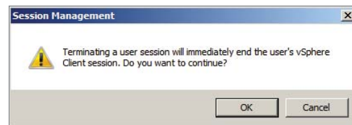
FIGURE 11.14 Session management
