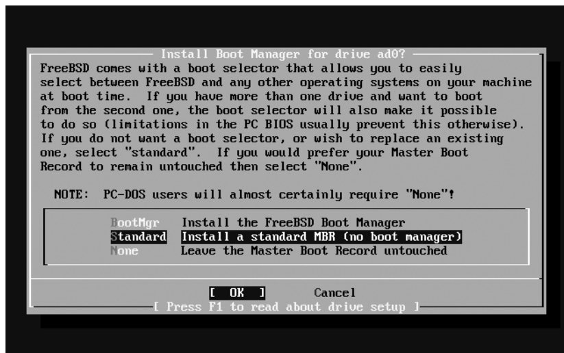
Figure 2-5: The MBR installer
