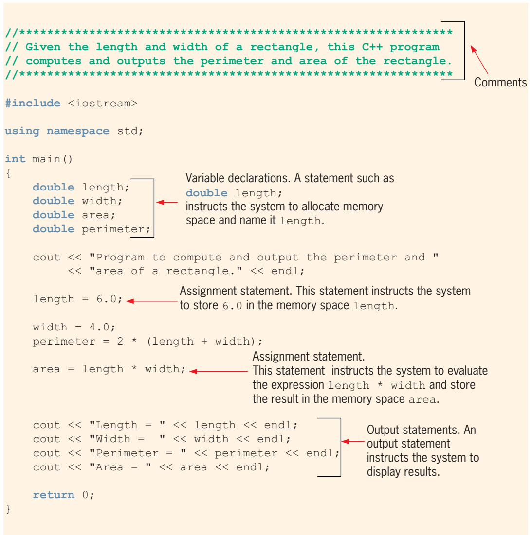
FIGURE 2-1 Various parts of a C++ program
