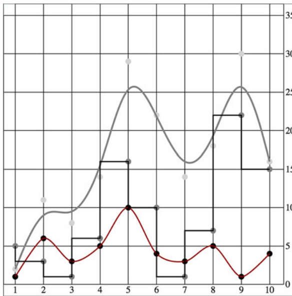
Figure 4.20 Light gray: “basis” interpolation; dark gray: “step” interpolation; black: “cardinal” interpolation 🌈
