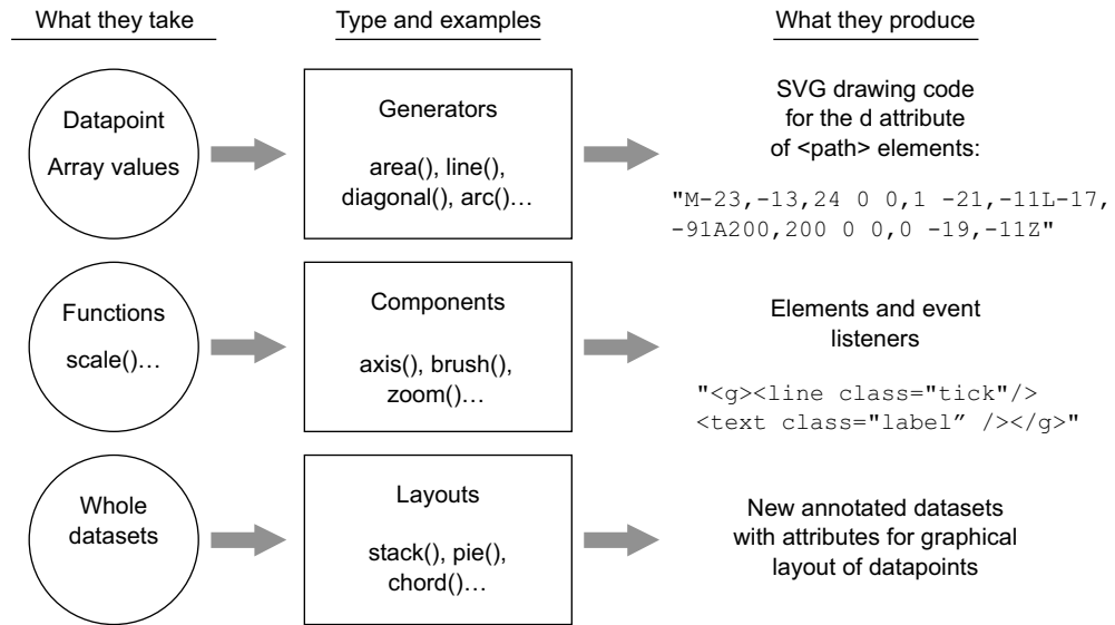
Figure 4.2 The three main types of functions found in D3 can be classified as generators, components, and layouts. You'll see components and generators in this chapter and layouts in the next chapter.
