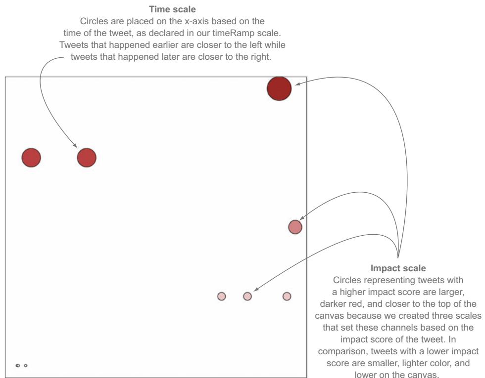
Figure 2.23 Tweets are represented as circles sized by the total number of favorites and retweets, and are placed on the canvas along the x-axis based on the time of the tweet and along the y-axis according to the same impact factor used to size the circles. Two tweets with the same impact factor that were made at nearly the same time are shown overlapping at the bottom left. 🗺️
