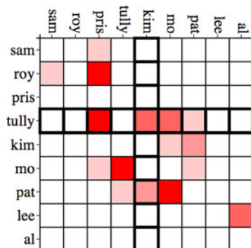
Figure 6.4 Adjacency highlighting column and row of the grid square. In this instance, the mouse is over the Tully-to-Kim edge. You can see that Tully favored tweets by four people, one of whom was Kim, and that Kim only had tweets favored by one other person, Pat. 🇺🇸
