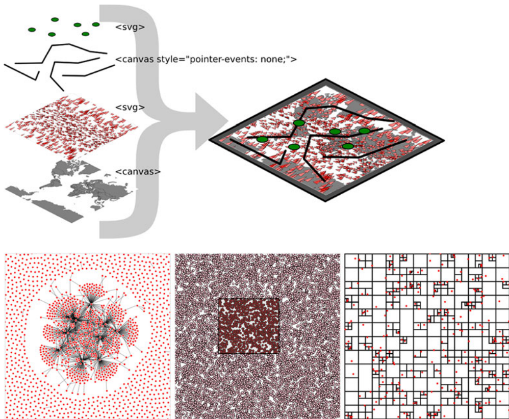
Figure 11.1 This chapter focuses on optimization techniques such as using HTML5 canvas to draw large datasets in tandem with SVG for the interactive elements. This is demonstrated with maps (section 11.1), networks (11.2), and traditional xy data (section 11.3), which uses the D3 quadtree function (section 11.3.2).
