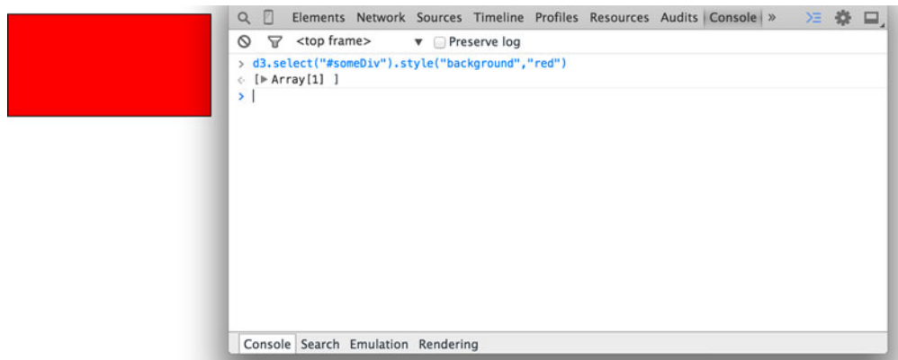
Figure 1.12 You can run JavaScript code in the console and also call global variables or declare new ones as necessary. Any code you write in the console and changes made to the web page are lost as soon as you reload the page.
