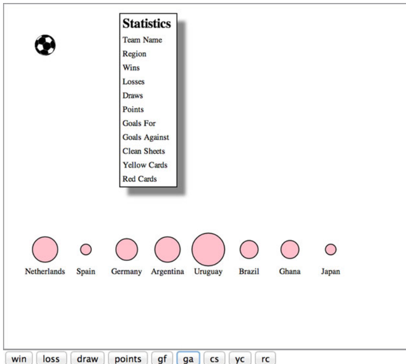
Figure 3.22 A hand-drawn football icon is loaded onto the <svg> canvas, along with the other SVG and HTML elements we created in our code.
