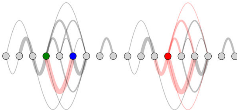
Figure 6.6 Mouseover behavior on edges (left), with the edge being moused over in pink, the source node in blue, and the target node in green. Mouseover behavior on nodes (right), with the node being moused over in red and the connected edges in pink. 🎨
