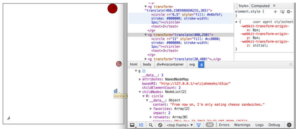
Figure 2.26 Only four <g> elements remain, corresponding to the four data values in the new array, with their <text> labels reset to match the new values in the array. But when you inspect the <g> element, you see that its __data__ property, where D3 stores the bound data, is different from that of its <circle> child element, which still has the JSON object we bound when we first created the visualization.
