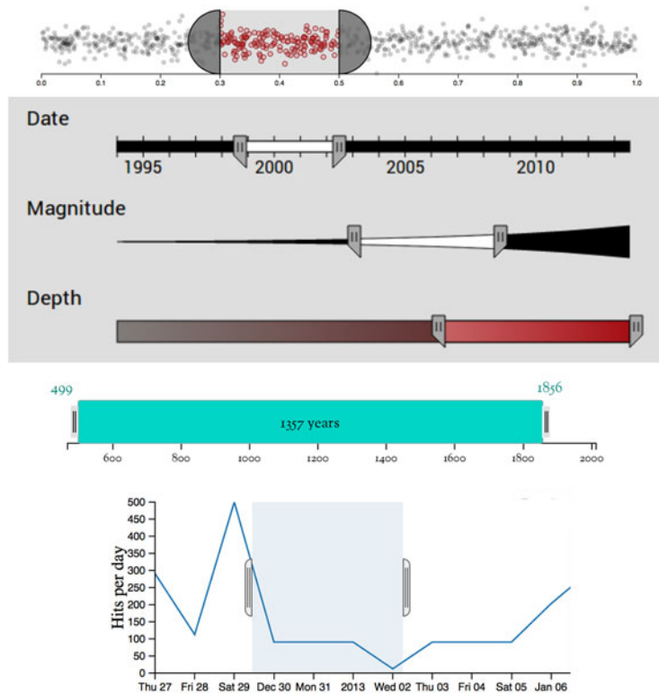
Figure 9.11 Brush handles on a variety of brushes, such as (from top) an example by Mike Bostock, a CS project exploring earthquake frequency, the Kindred Britain search brush, and dc.js. 1
