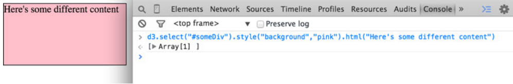
Figure 1.16 The D3 select syntax modifies style using the .style() function, and traditional HTML content using the .html() function.
