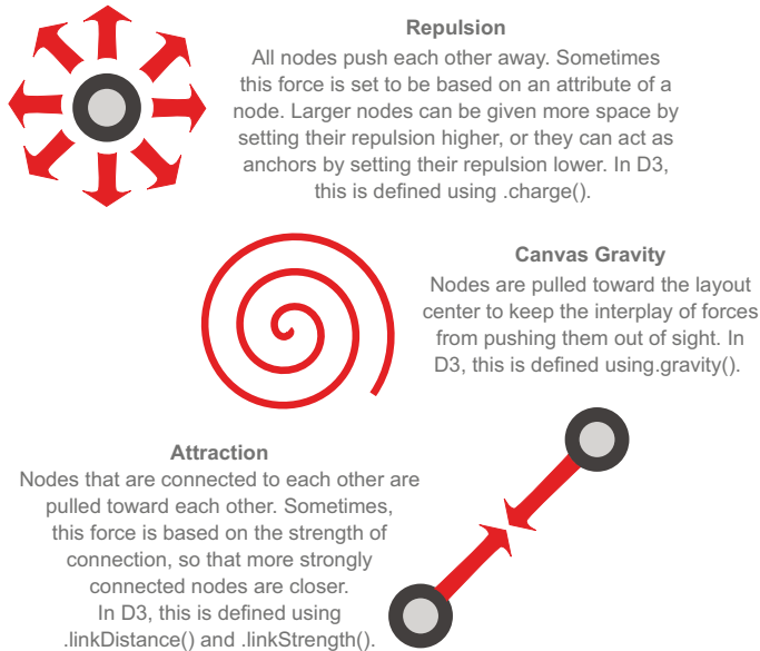
Figure 6.7 The forces in a force-directed algorithm: repulsion, gravity, and attraction. Other factors, such as hierarchical packing and community detection, can also be factored into force-directed algorithms, but these features are the most common. Forces are approximated for larger networks to improve performance.
