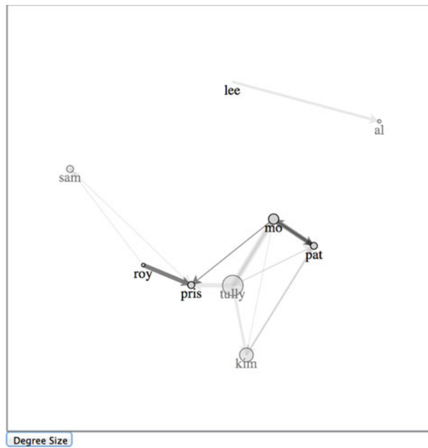
Figure 6.18 The network has been filtered to only show nodes with more than 20 followers, after clicking the Degree Size button. Notice that Lee, with no connections, has a degree of 0 and so the associated circle has a radius of 0, rendering it invisible. This catches two processes in midstream, the transition of nodes from full to 0 opacity and the removal of edges.
