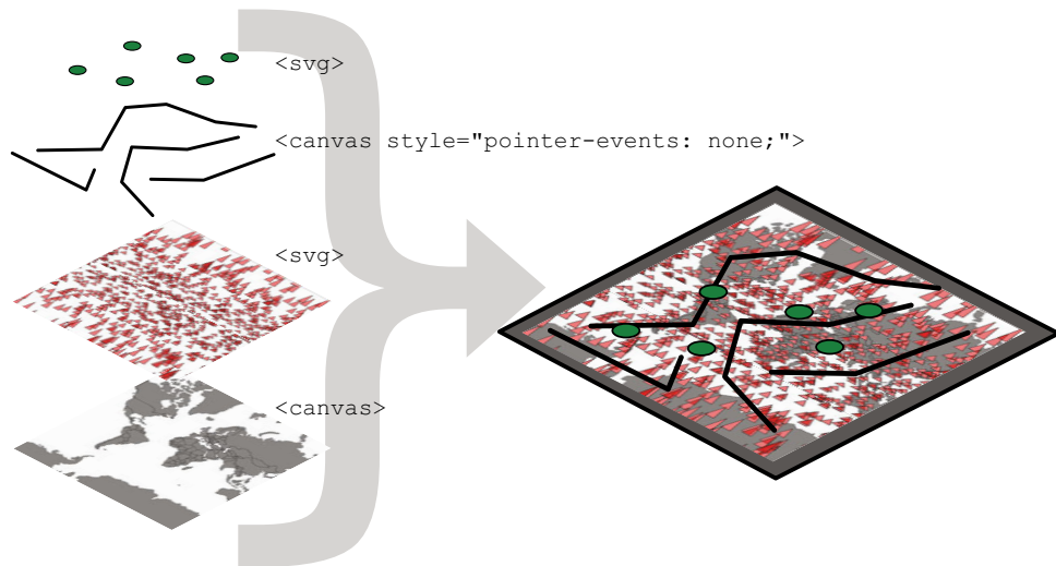
Figure 11.7 Placing interactive SVG elements below a <canvas> element requires that you set its pointer-events style to "none", even if it has a transparent background, in order to register click events on the <svg> element underneath it.
