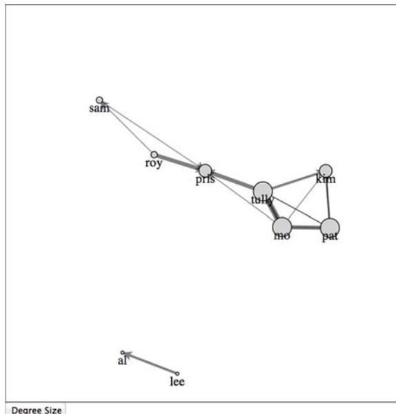
Figure 6.11 Sizing nodes by weight indicates the number of total connections for each node by setting the radius of the circle equal to the weight times 2.
