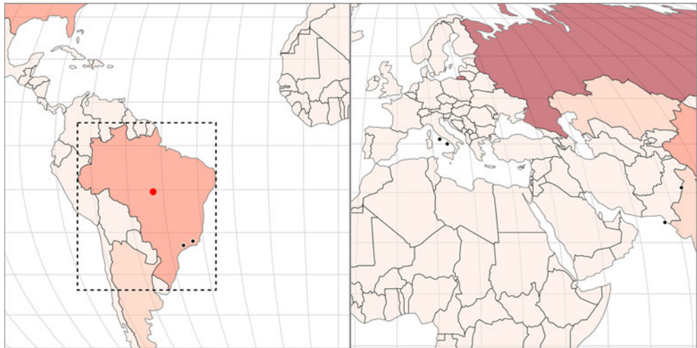
Figure 7.9 Our map with zooming enabled. Panning occurs with the drag behavior and zooming with mousewheel and/or double-clicking. Notice that the bounding box and centroid functions still work, because they're based on our constantly updating projection.
