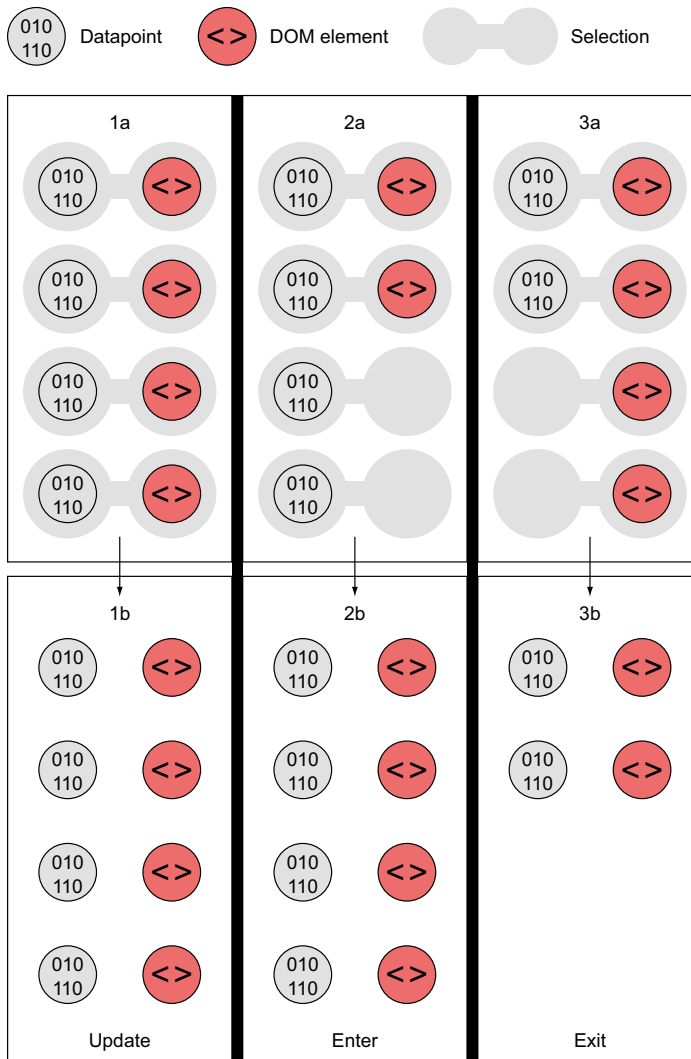
Figure 2.24 Selections where the number of DOM elements and number of values in an array don't match will fire either an .enter() event or an .exit() event, depending on whether there are more or fewer data values than DOM elements, respectively.
