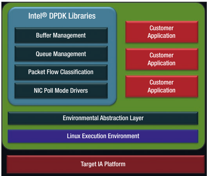
Figure 4-20. The Intel DDPK library structure
