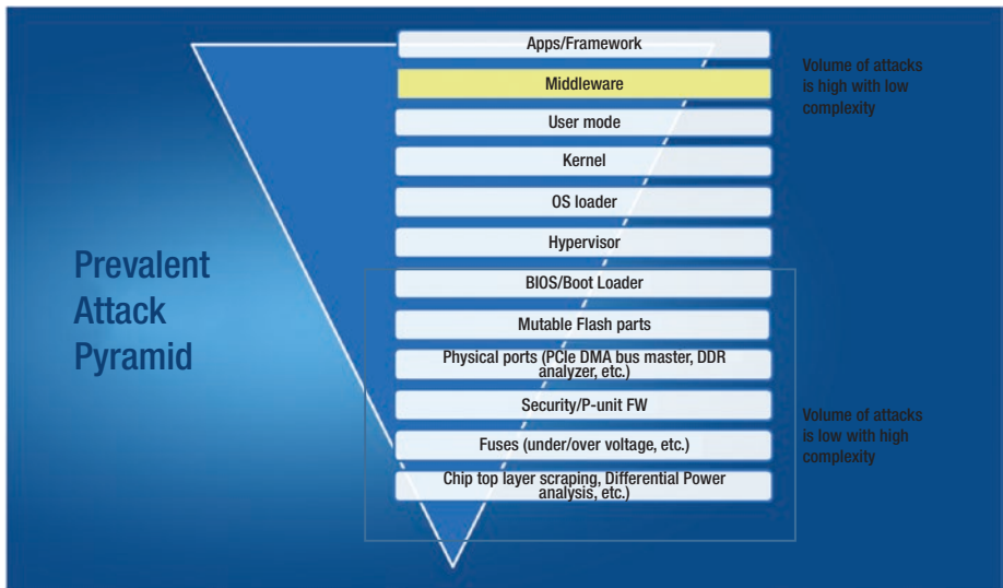
Figure 3-3. Attack pyramid
