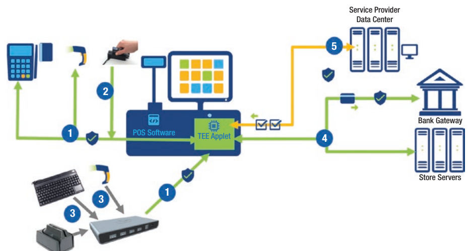
Figure 6-7. The end-to-end data flow in a Retail POS architecture
