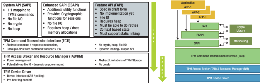
Figure 4-22. Intel TPM2 software stack (TSS) 50
