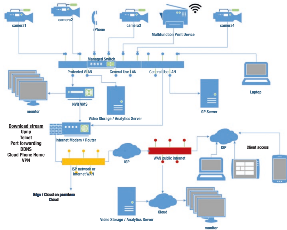
Figure 6-17. Digital Surveillance System (DSS) typical network architecture
