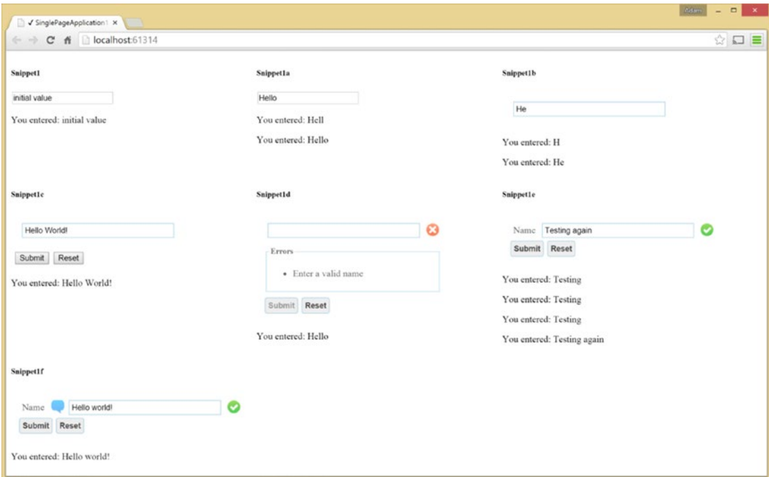
Figure 14-5. Simple formlets
