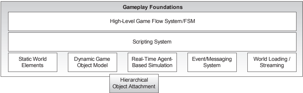
Figure 1.29. Gameplay foundation systems.
