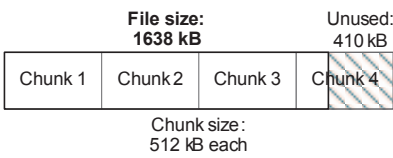
Figure 6.5. The last chunk of a resource file is often not fully utilized.
