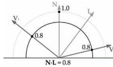
Figure 10.24. The diffuse term of the Phong reflection model is dependent upon N \cdot L , but is independent of the viewing angle V .
