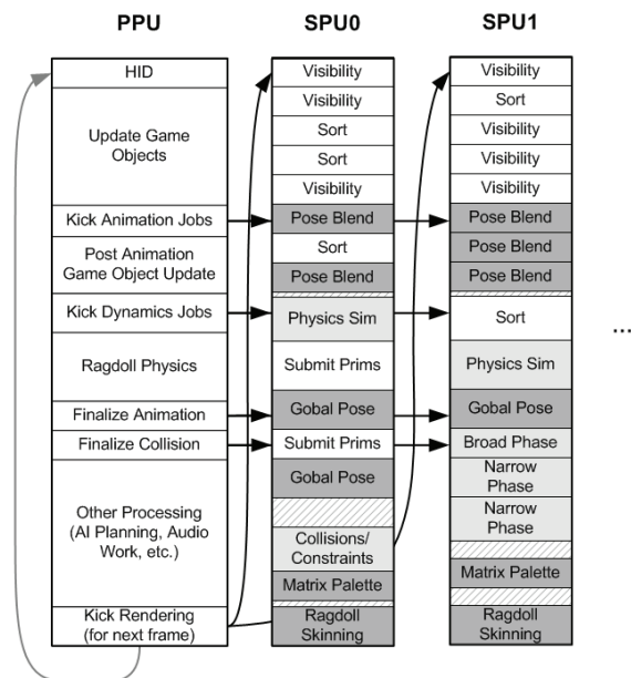
Figure 7.8. In a job architecture, work is broken down into fine-grained chunks that can be picked up by any available processor. This can help maximize processor utilization, while providing the main game loop with improved flexibility.
