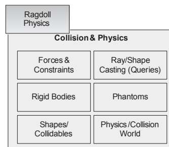
Figure 1.24. Collision and physics subsystem.
