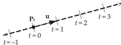
Figure 4.24. Parametric equation of a line.
