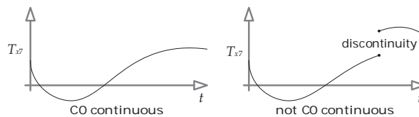
Figure 11.26. The channel function on the left has C0 continuity , while the path on the right does not.
