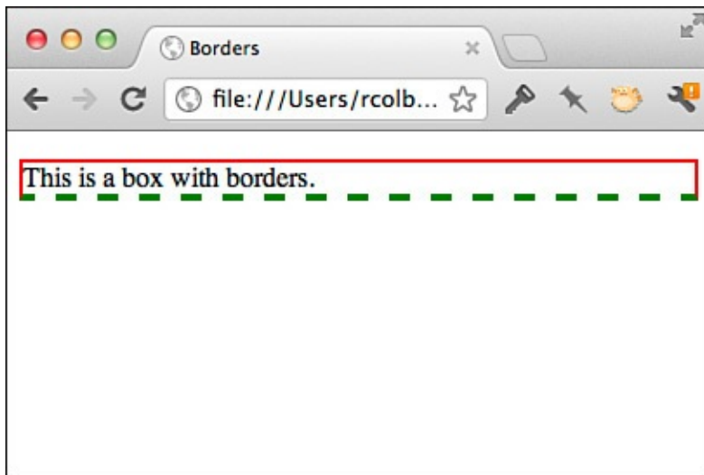
FIGURE 8.6 Border styles.
