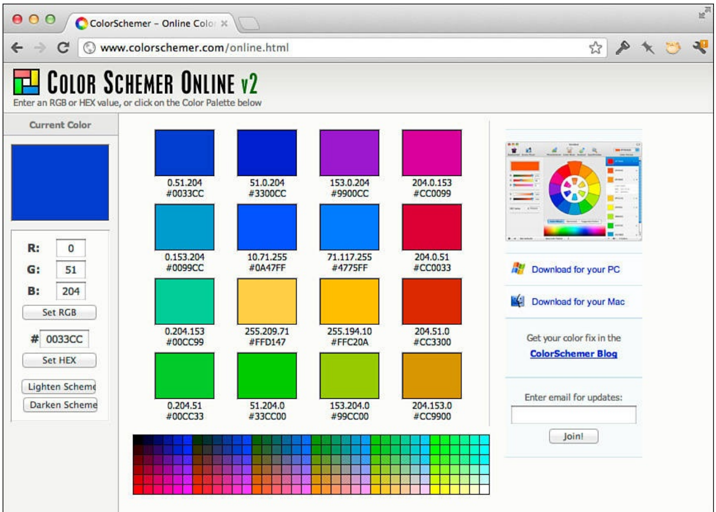
FIGURE 8.2 Color Schemer.
