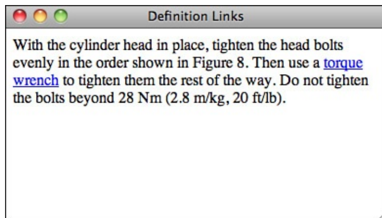
FIGURE 21.6 Definition links.
