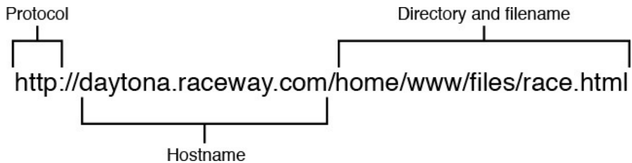
FIGURE 6.14 URL parts.
