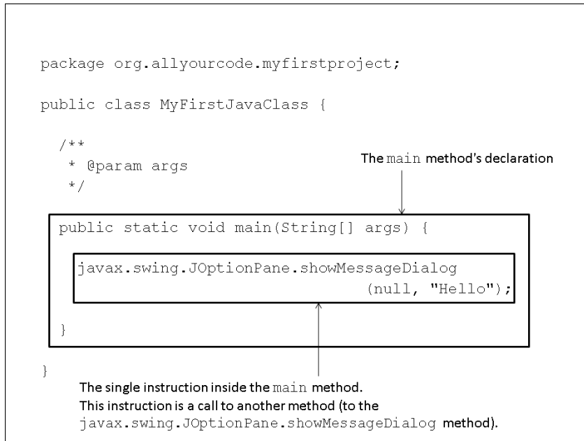
Figure 5-5: A method declaration and a method call.
