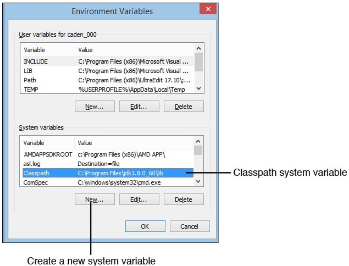
FIGURE D.9 Setting environment variables in most Windows versions.
