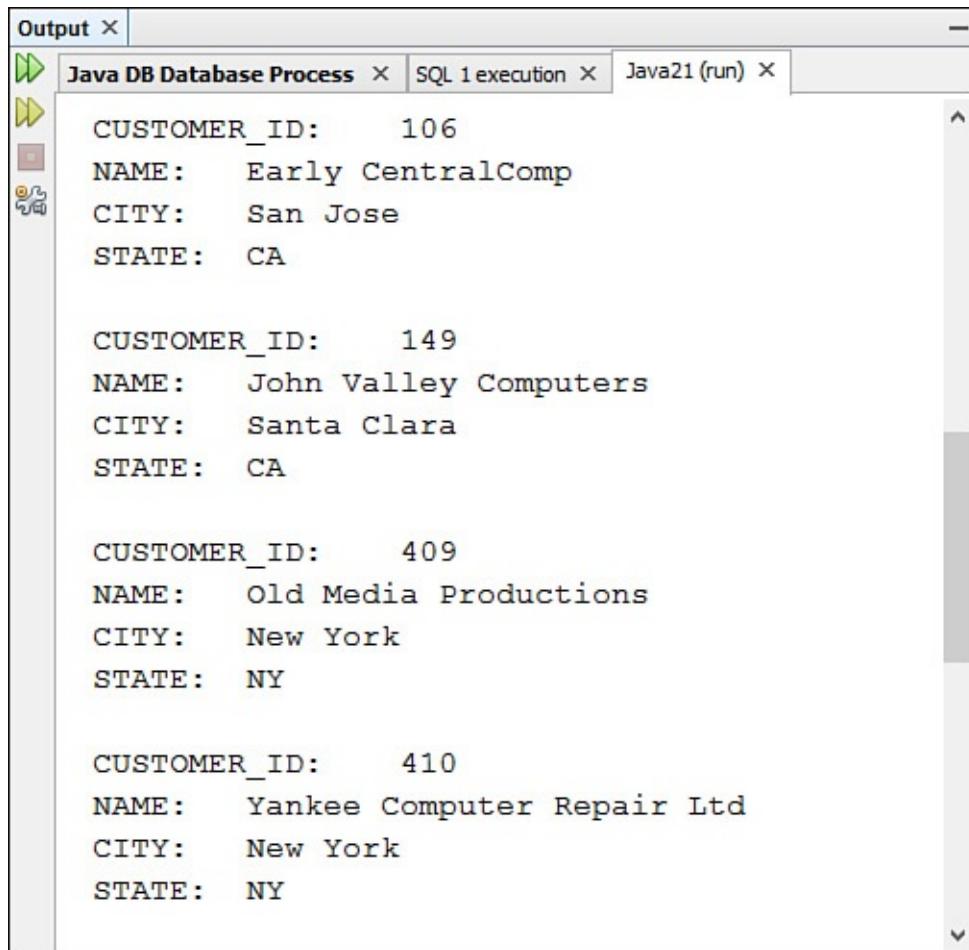
FIGURE 18.6 Reading records from a Java DB database.
