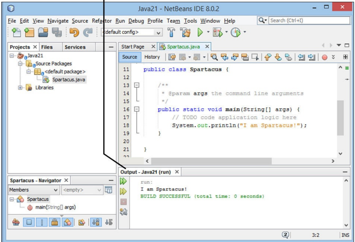
FIGURE A.4 Viewing program output in the NetBeans Output pane.
