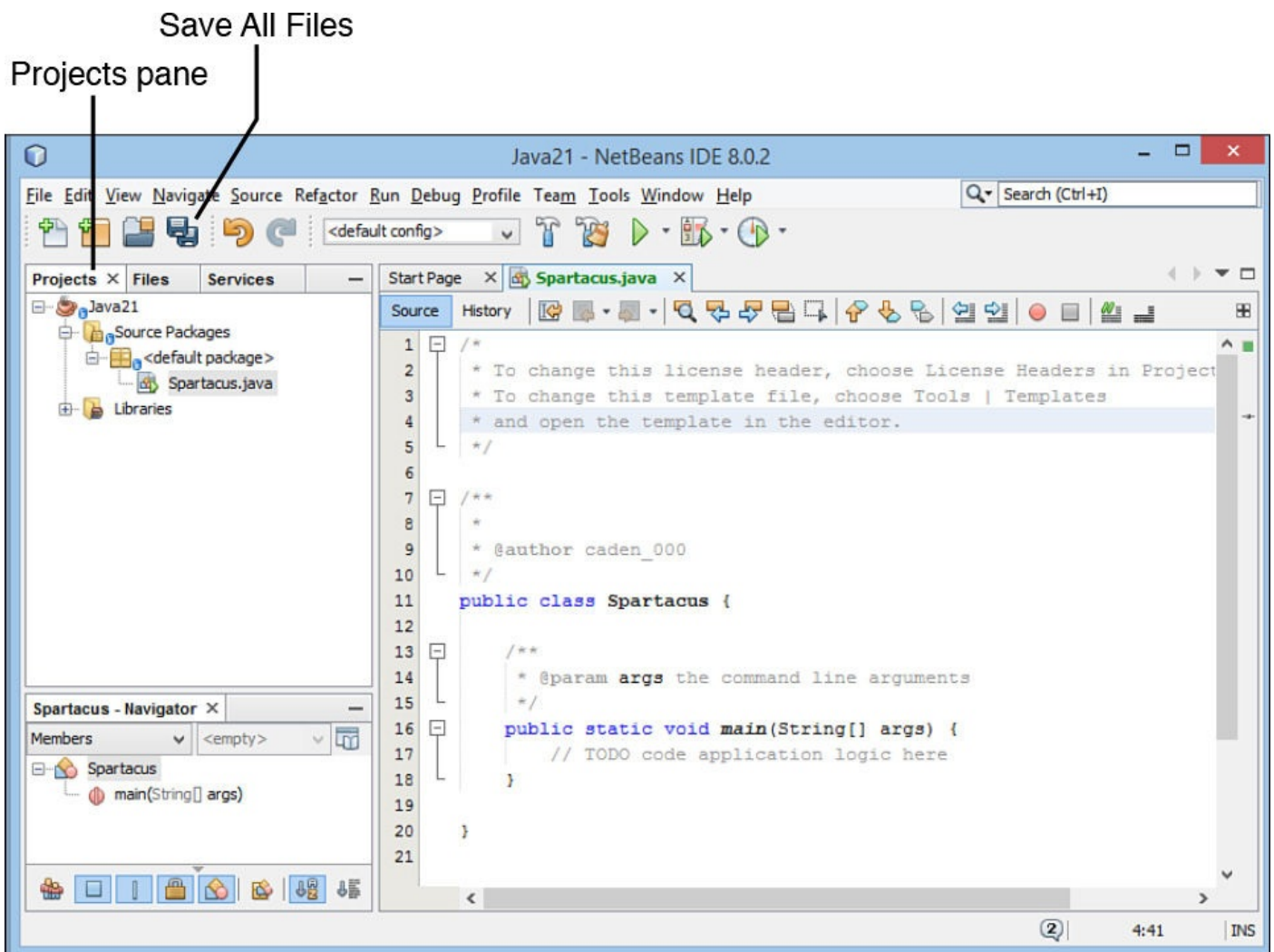
FIGURE A.3 The NetBeans source editor.
