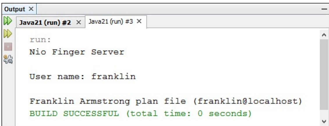
FIGURE 17.6 Making a Finger request from your Finger server.
