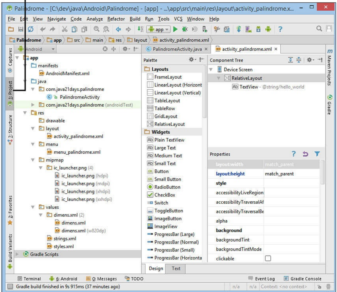
FIGURE 21.3 Viewing the components of an Android project.
