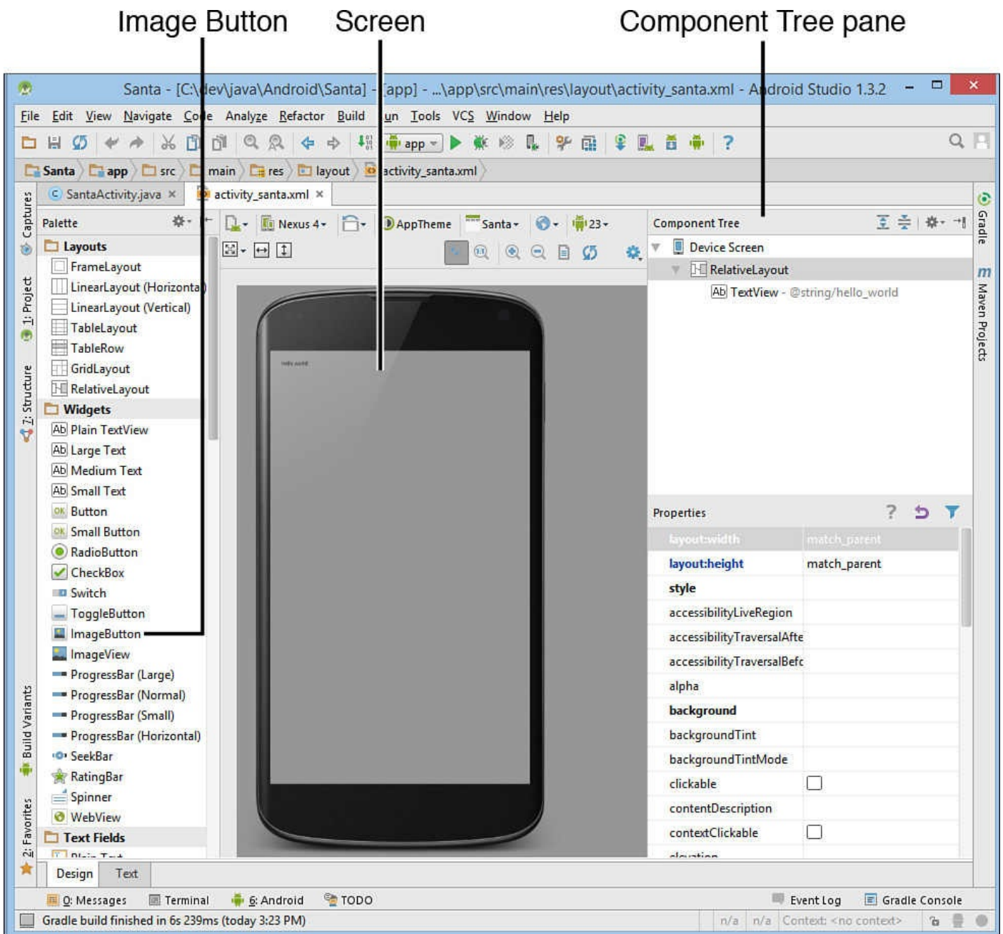
FIGURE 21.9 Editing an activity’s graphical user interface.
