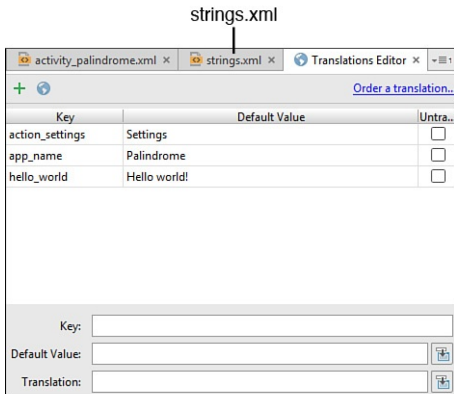
FIGURE 21.4 Creating an app's string resources.
