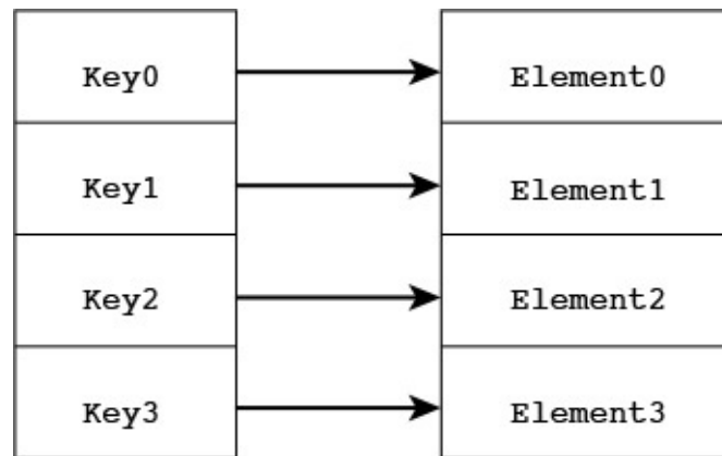
FIGURE 8.5 The organization of a key-mapped data structure.
