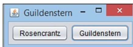
FIGURE 12.1 The TitleBar application.
