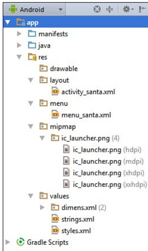
FIGURE 21.7 Examining an app's resources.
