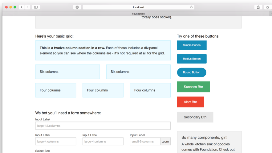
Figure 7.2. Example index.html
