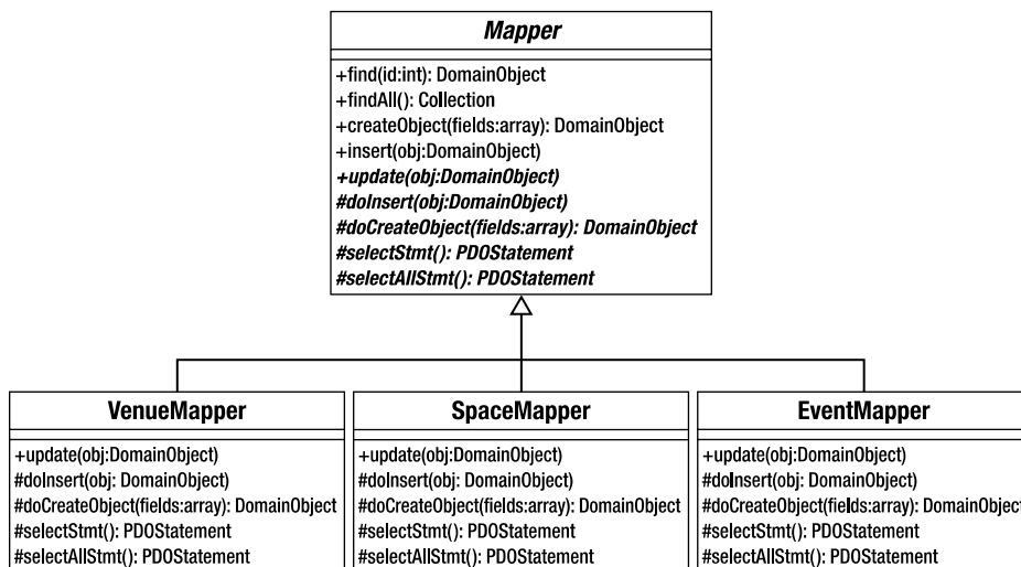
Figure 13-1. Mapper classes
