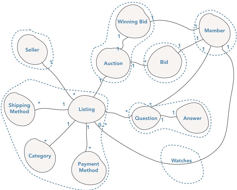
FIGURE 19-20: All aggregate boundary definitions.
