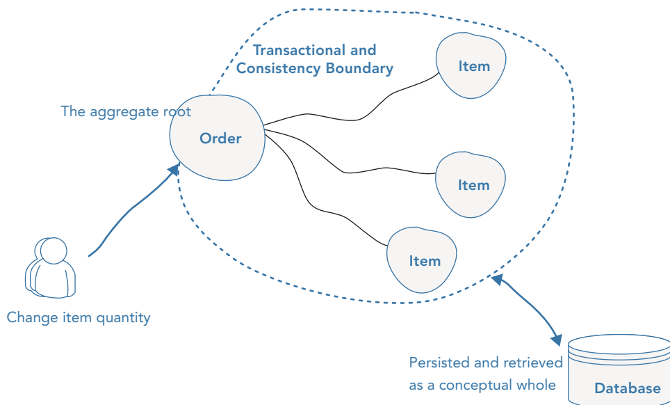
FIGURE 19-12: Enforcing consistency with help from aggregate roots.
