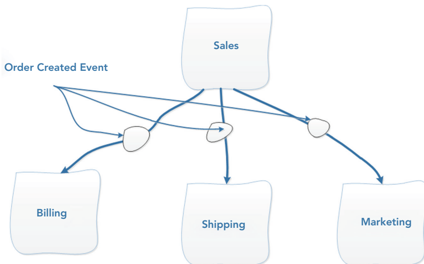
FIGURE 12-2: Adding new event subscribers doesn't affect existing code.
