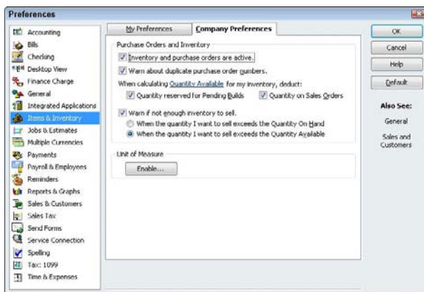
Figure 3-11: The Company Preferences tab of the Items & Inventory dialog box.
