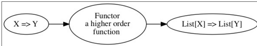
Figure 9.1: Functor translation
