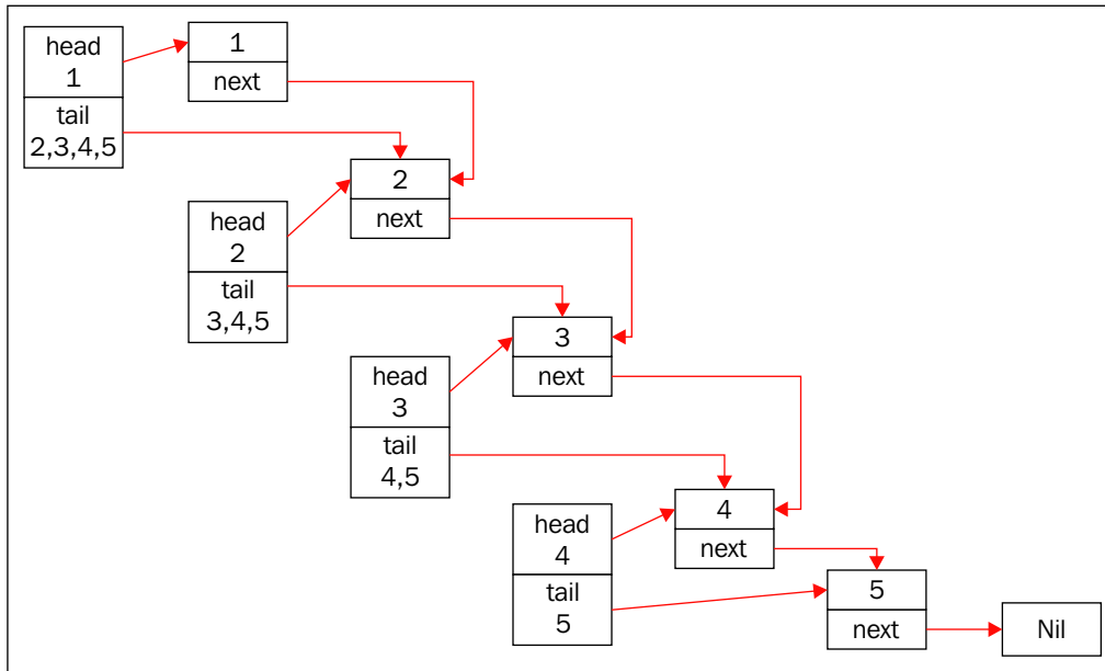
Figure 3.2: Losing head at every iteration
