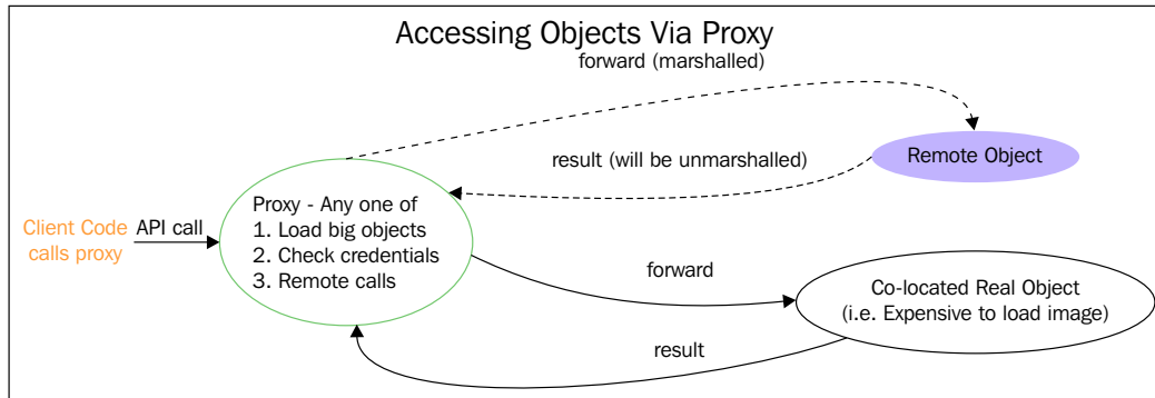
Figure 4.2: Proxy – execution flow
