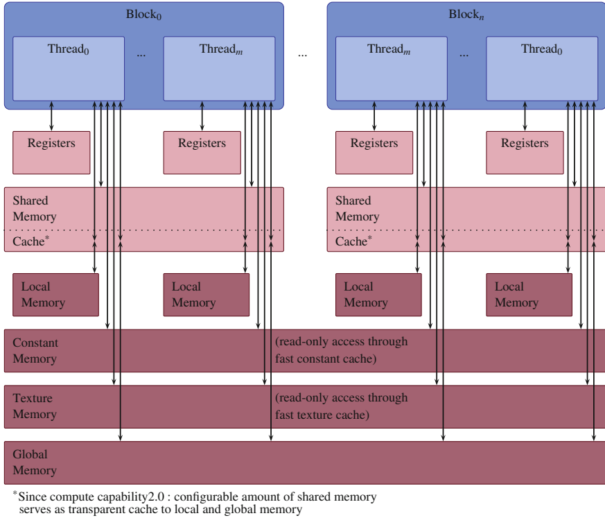
Fig. 8.1 Access to different memories from threads on NVIDIA CUDA devices. Light-red memories are fast; dark-red memories are parts of device memory with high-latency access
