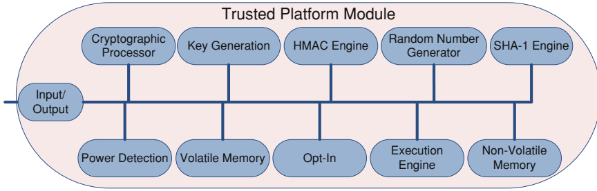
Fig. 4.2 Generic architecture of trusted platform module [1]
