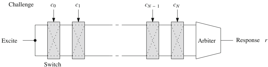
Fig. 19.1 Basic arbiter PUF design (for N bit challenge and 1 bit response)
