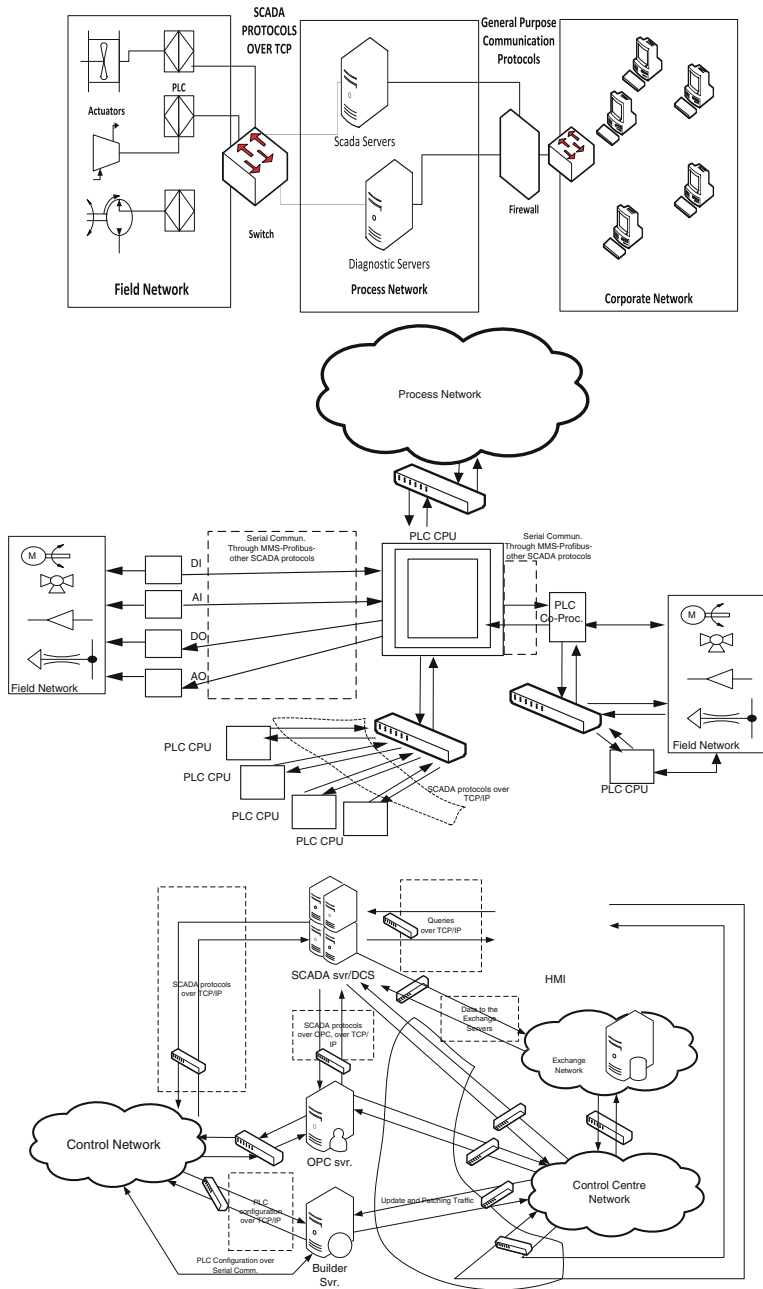
Fig. 20.1 a High level schema of the SCADA cyber layer, b Control network, c Process network
