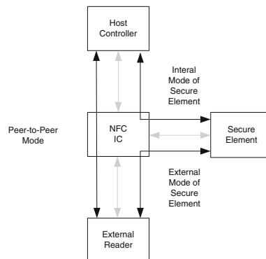
Fig. 15.4 SmartConnect architecture for NFC chips with an embedded secure element [13]
