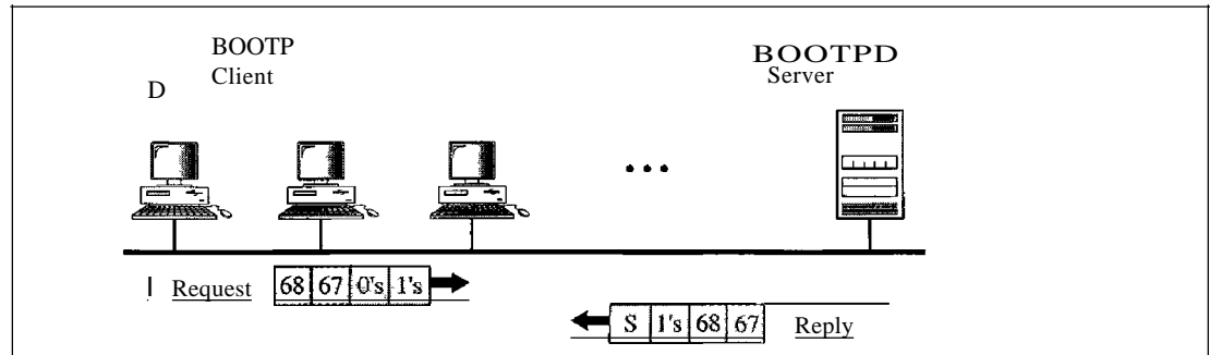
a. Client and server on the same network
