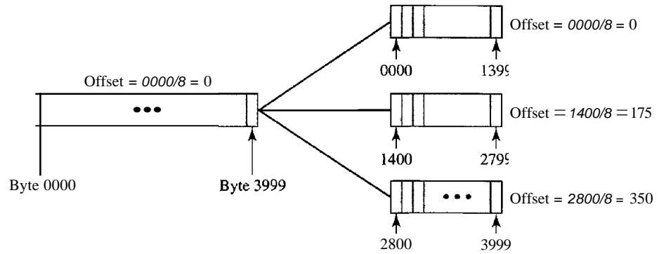
Figure 20.11 Fragmentation example
