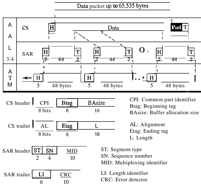
Figure 18.22 AAL3/4
