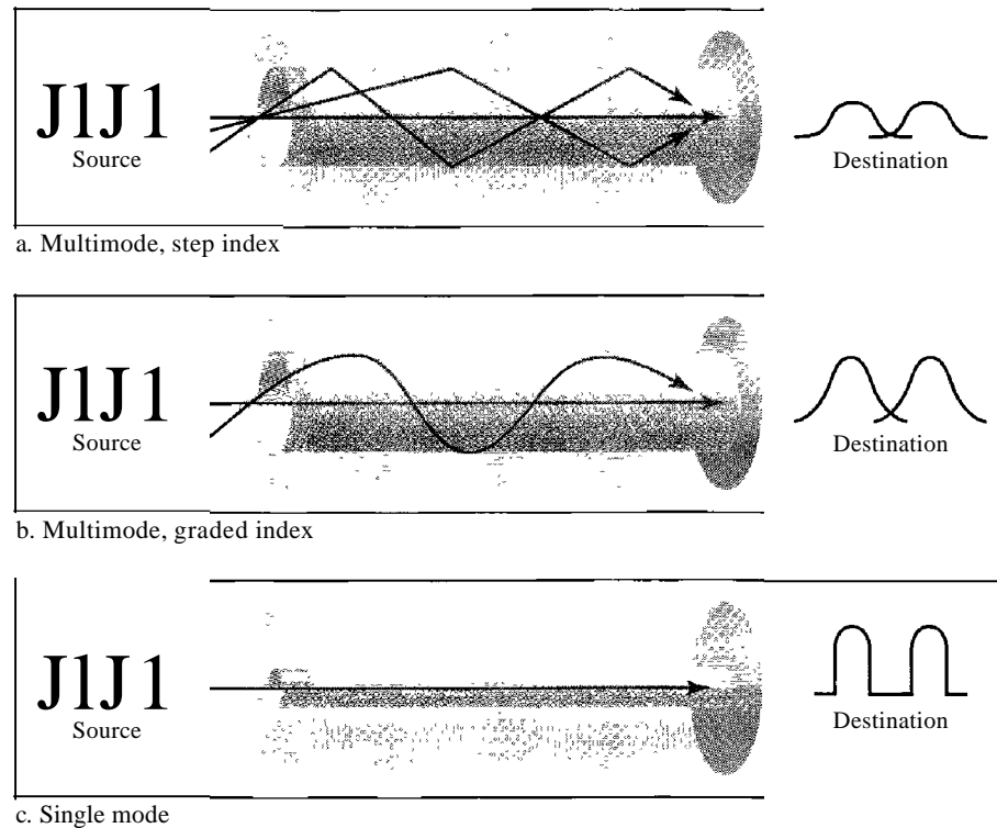
Figure 7.13 Modes
