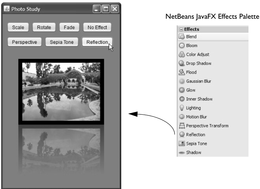
Figure 8.4 Applying various effects and transformations to components
