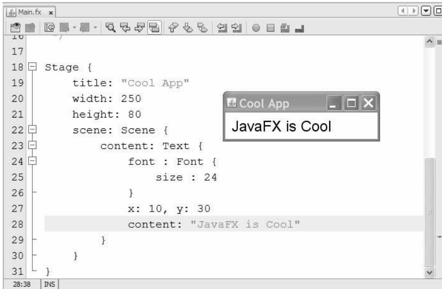
Figure I.7 Run CoolApp Application
