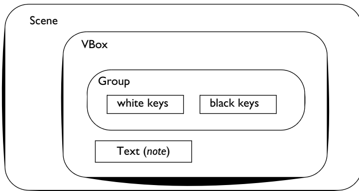
Figure 6.7 Scene Node Diagram for updated Piano application
