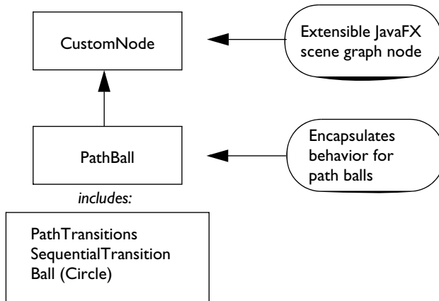
Figure 7.12 Chutes and Ladders PathBall class
