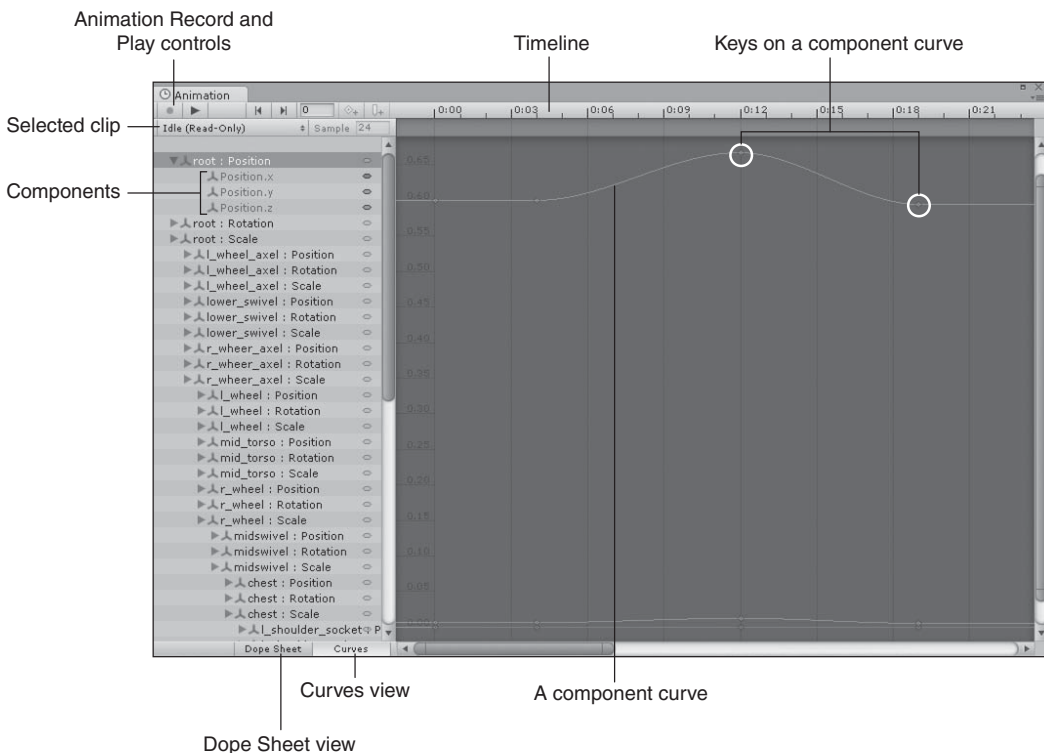
Figure 8.1 The Animation view. Source: Unity Technologies.
