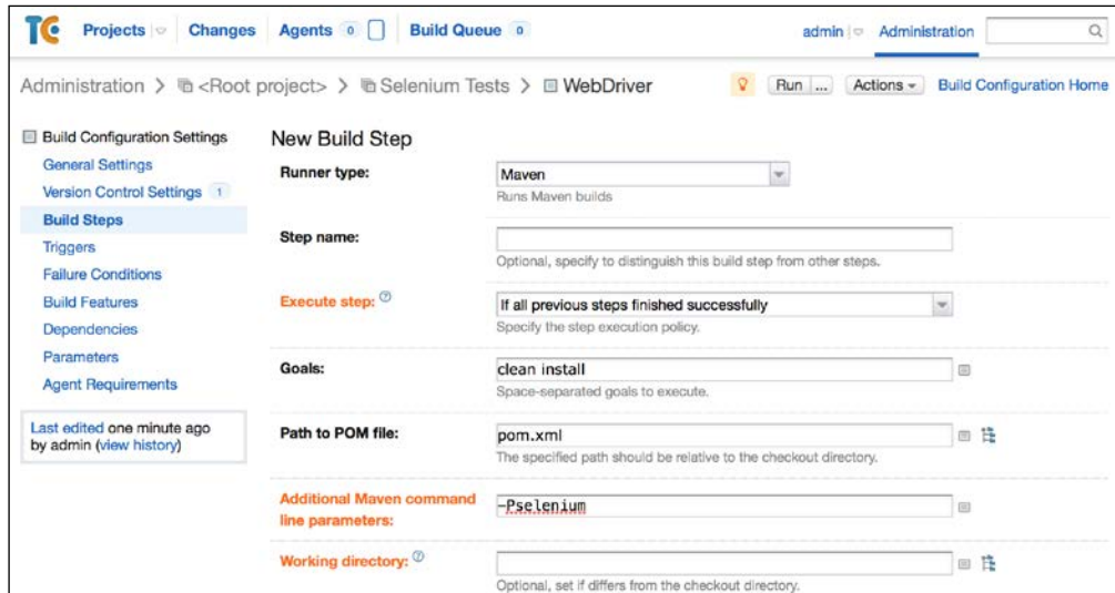
Configuring your Maven build step
