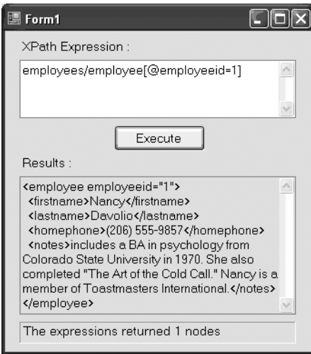
Figure 4-3. Executing XPath expressions
