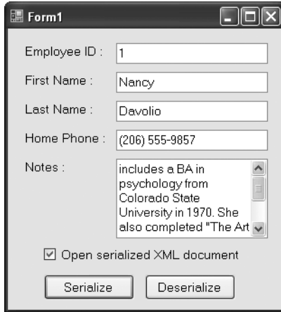
Figure 8-1. Application for illustrating XML serialization
