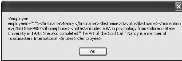
Figure 7-22. The XmlElement retrieved by using the GetElementFromRow() method
