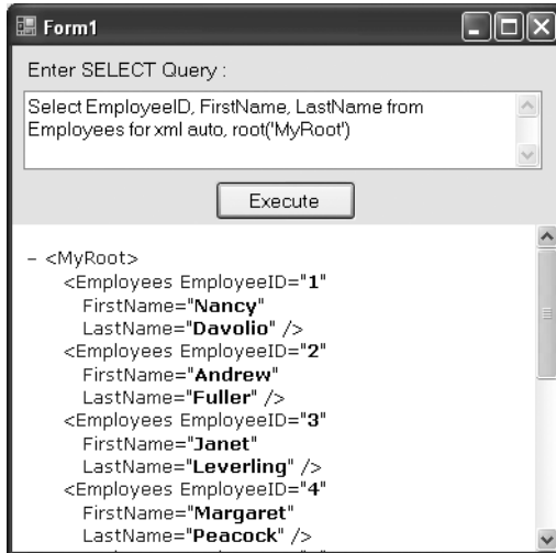
Figure 10-2. Application for executing SELECT queries via SqlXmlCommand
