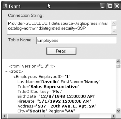
Figure A-2. Application that consumes TableReader class
