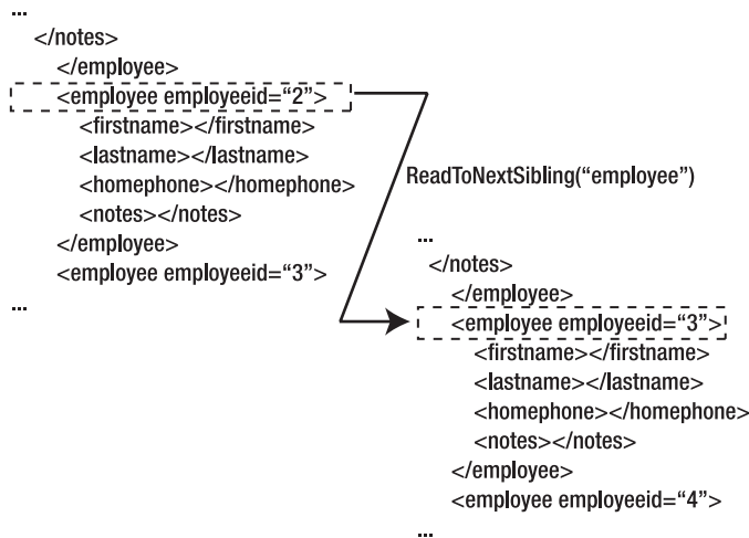
Figure 3-5. Using the ReadToNextSibling() method
