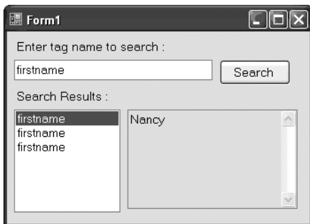
Figure 2-4. Using the GetElementsByTagName() method
