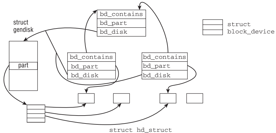
Figure 6-10: Connection between block devices, generic hard disks, and partitions.
