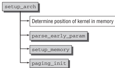
Figure D-2: Code flow diagram for setup_arch on IA-32 systems.
