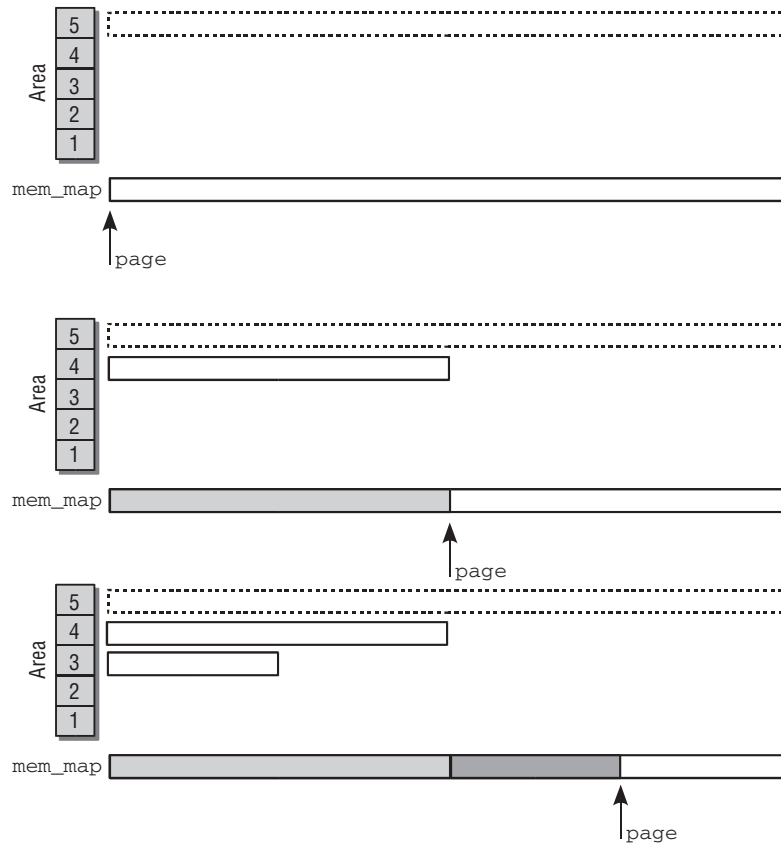
Figure 3-34: Steps performed by expand when splitting a memory area.
