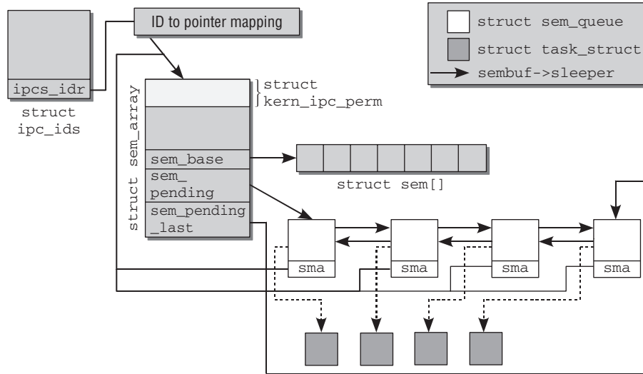
Figure 5-2: Interplay between the semaphore data structures.
