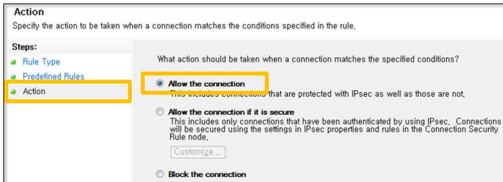
Figure 4-15 Select Action
