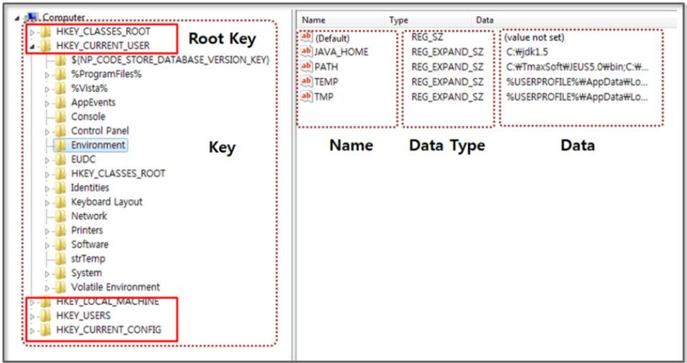
Figure 5-11 Registry settings
