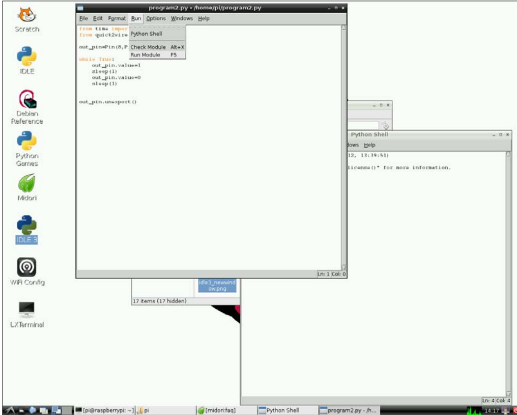
Executing the Python example
