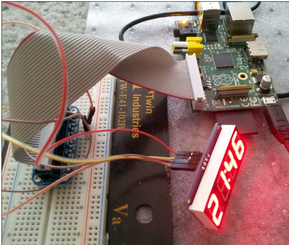
A 7-segment backpack connected to the Cobler
