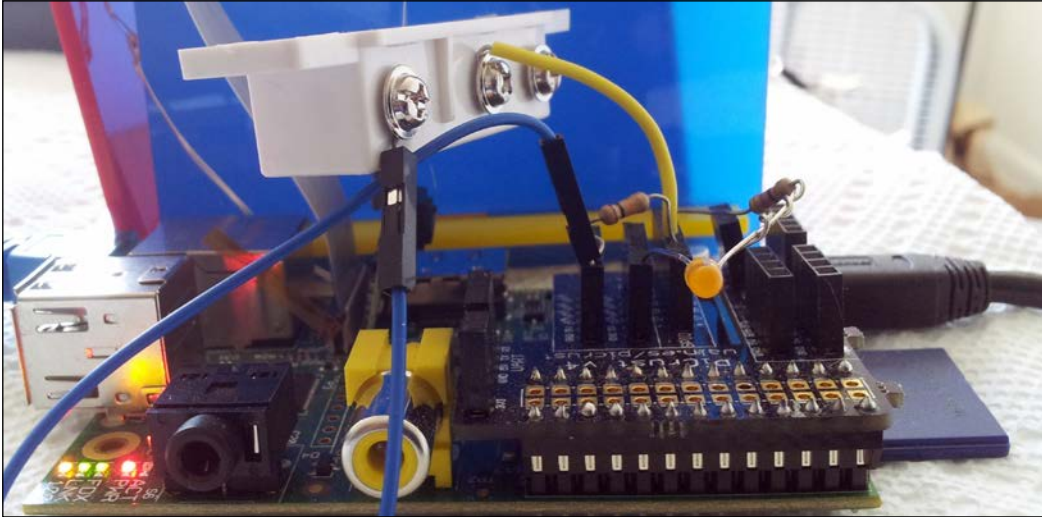
Reed switch interfaced to Raspberry Pi
