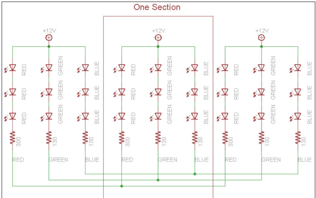
RGB LED strip schematic (borrowed from Adafruit)
