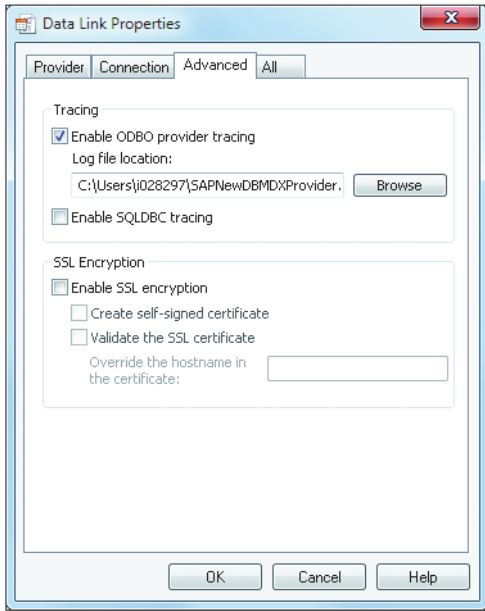
Figure 16.28 MDX/ODBO Trace
