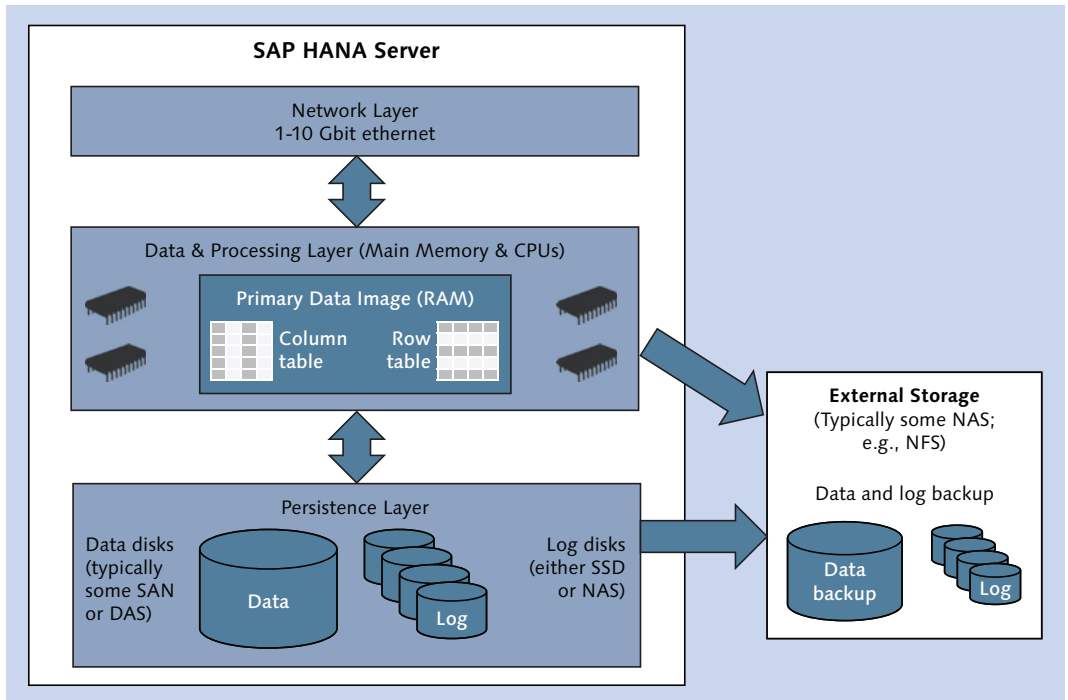
Figure 1.2 Hardware Building Blocks of an SAP HANA Server
