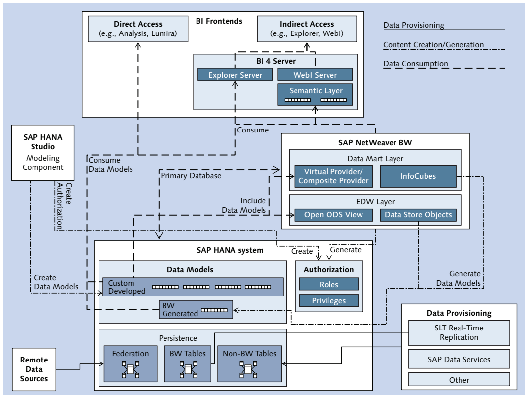
Figure 2.5 Options for Data Flow and Content Usage in SAP BW Mixed Scenarios
