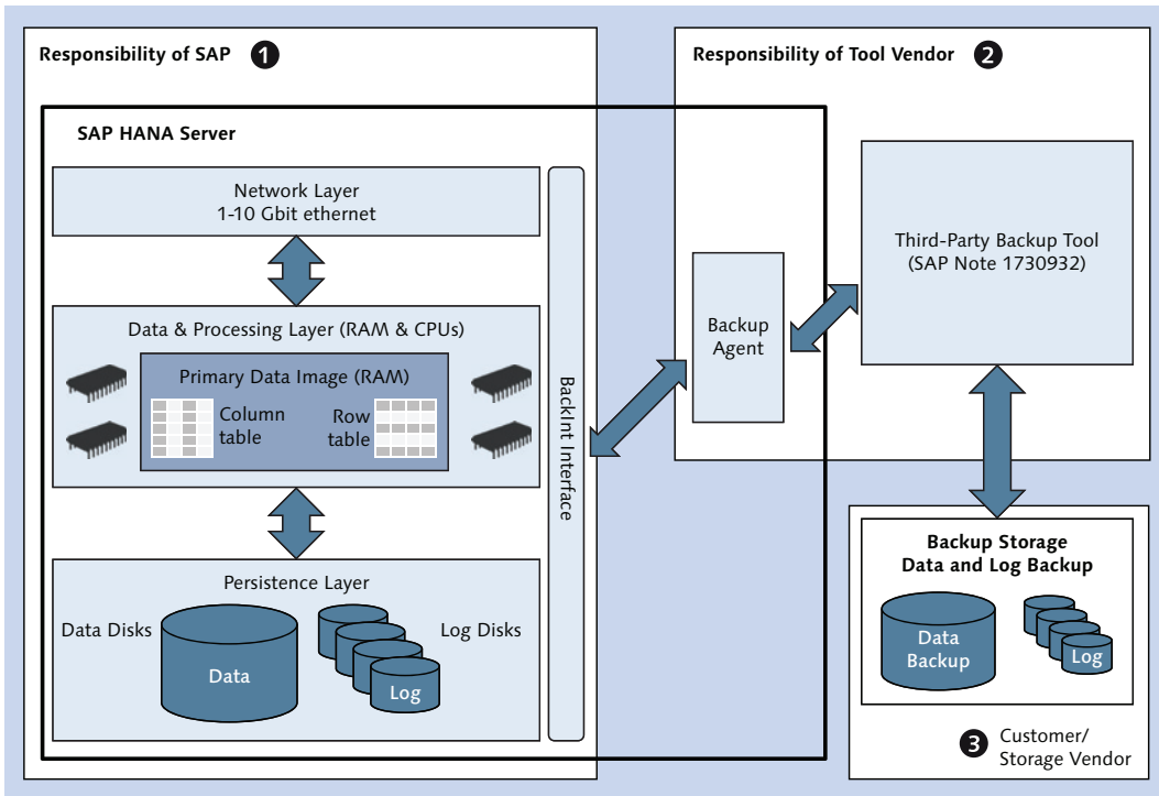
Figure 5.12 Integration with Third-Party Backup Tools and BackInt
