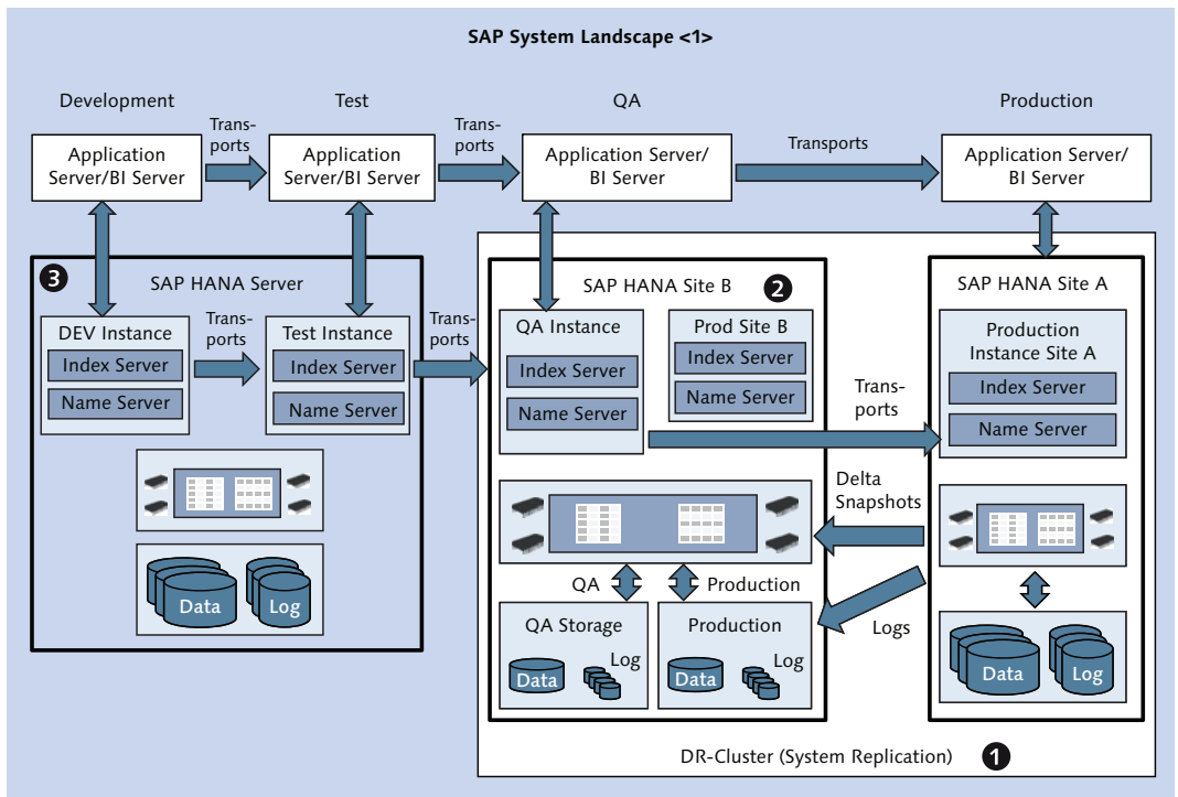
Figure 14.5 Using a DR Setup for Nonproduction Instances
