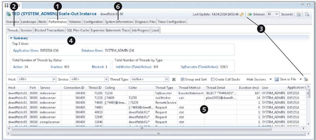
Figure 4.17 Typical Monitoring View in SAP HANA Studio
