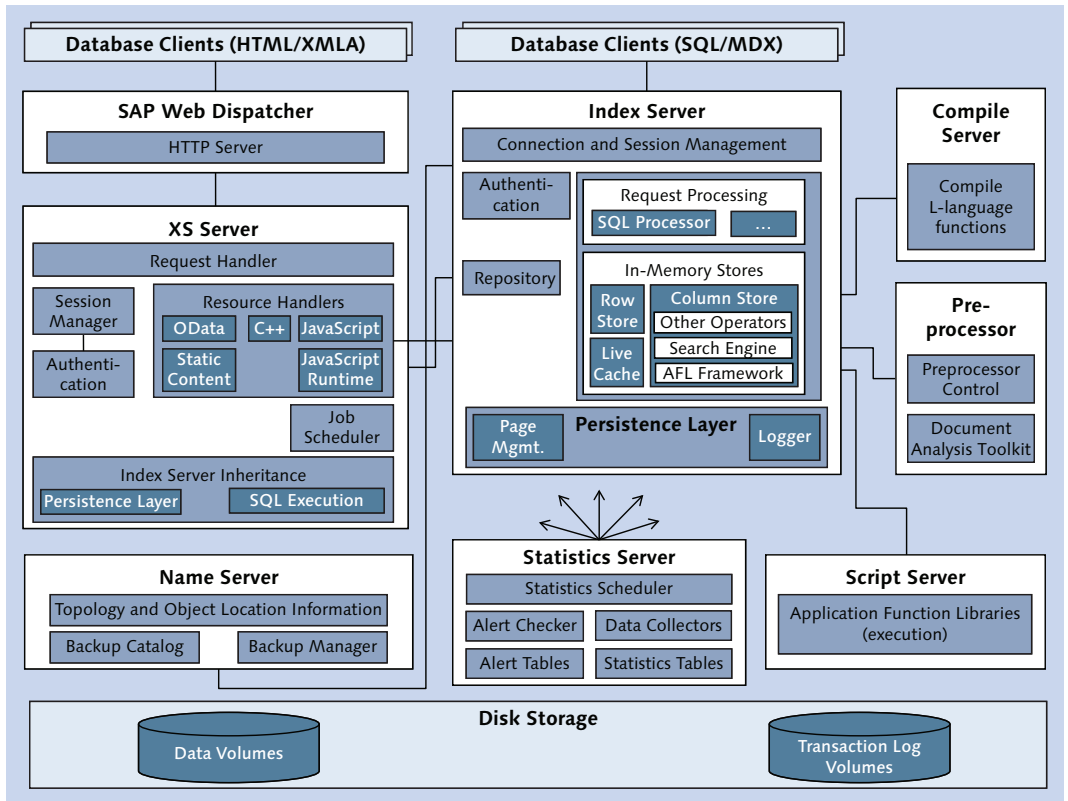
Figure 1.6 Internal Architecture of SAP HANA Database
