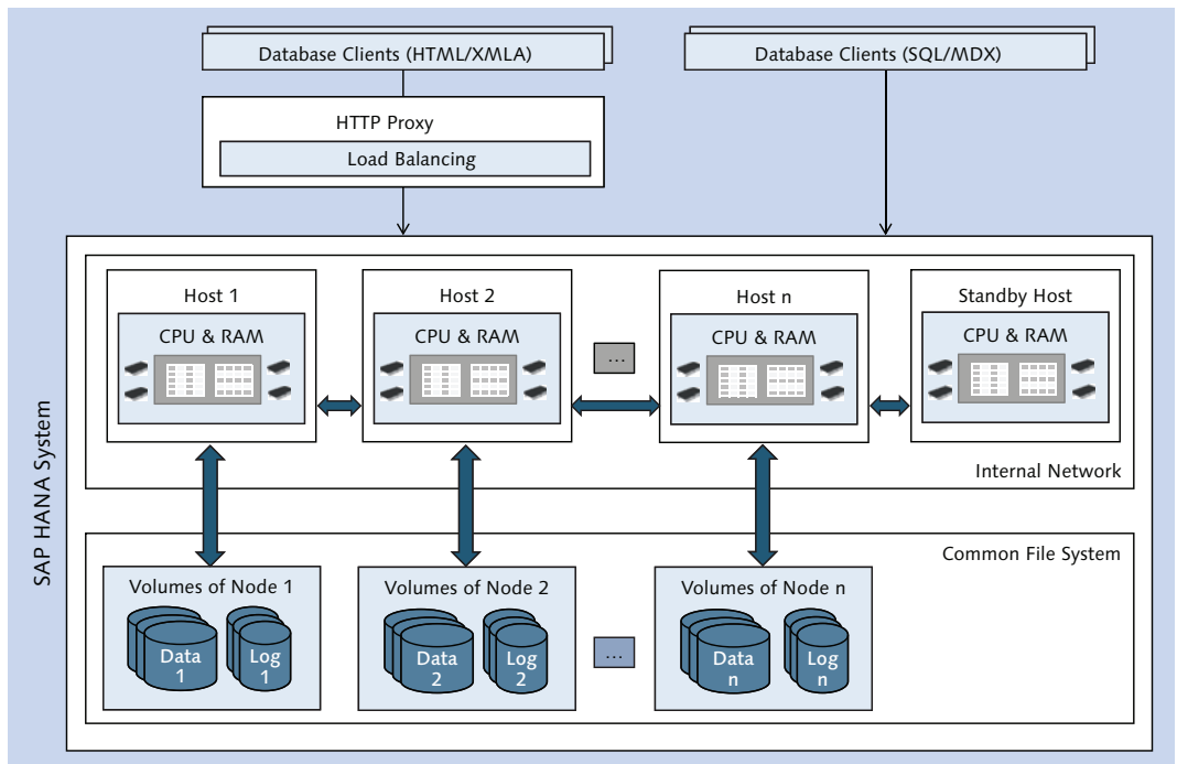
Figure 6.1 Schematic View of a Scale-Out Setup
