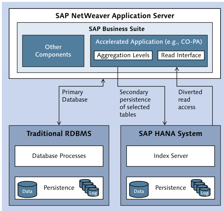
Figure 2.1 Simplified Architecture of an Accelerator System
