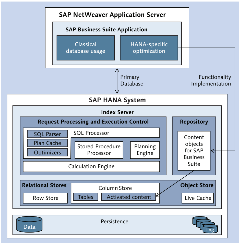
Figure 2.3 Architecture of SAP Business Suite on SAP HANA
