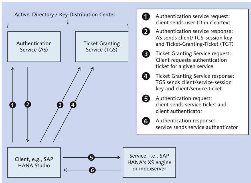
Figure 12.11 Schematic View of Client-Server Kerberos Authentication
