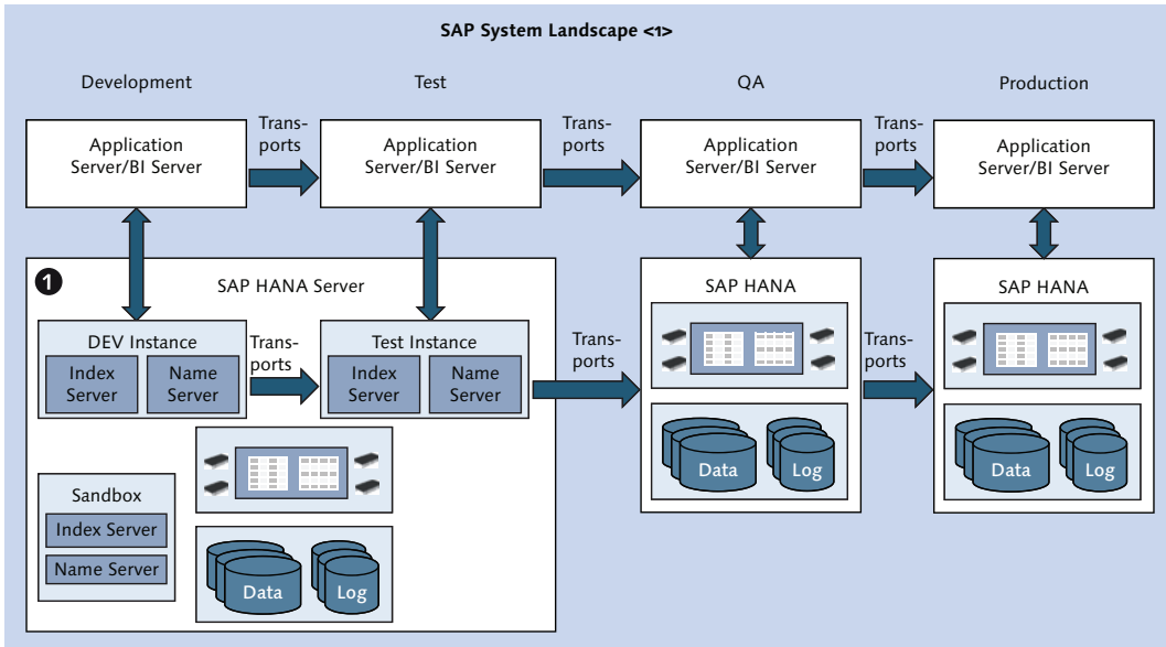
Figure 14.3 Combining Nonproduction Systems on One Physical Server
