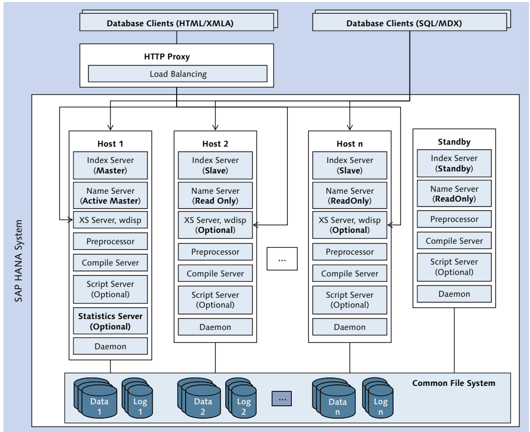
Figure 6.2 Database Processes in a Distributed System
