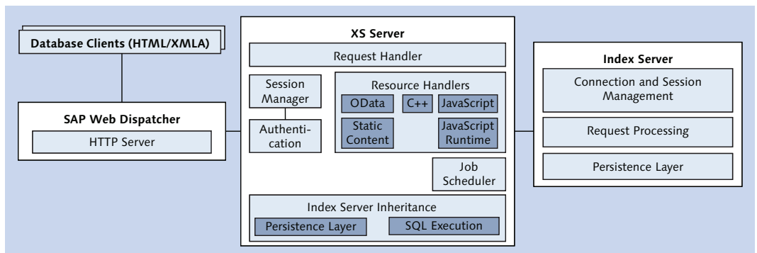
Figure 1.8 XS Server Architecture
