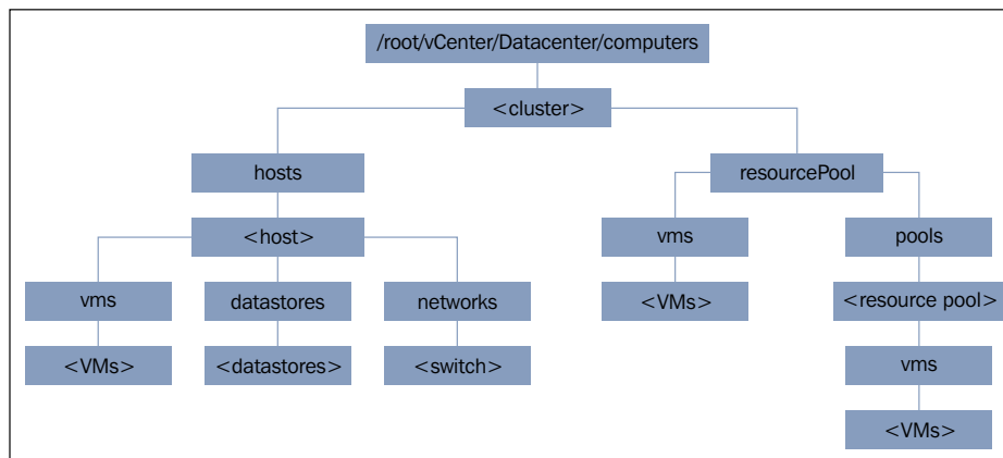
RVC "computers" branches
