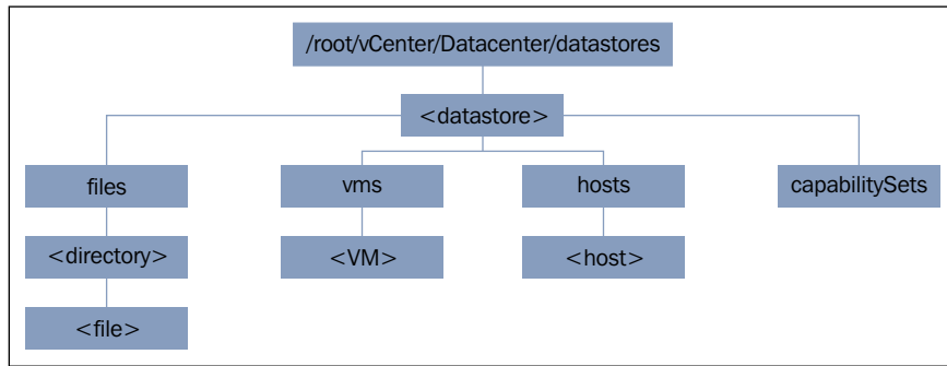
RVC "datastores" branches
