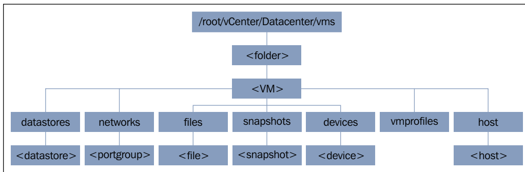
RVC "vms" branches
