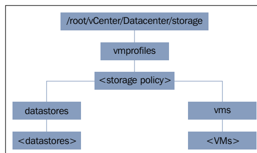
RVC "storage" branches
