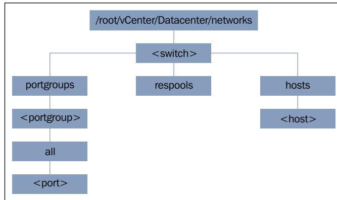
RVC "networks" branches
