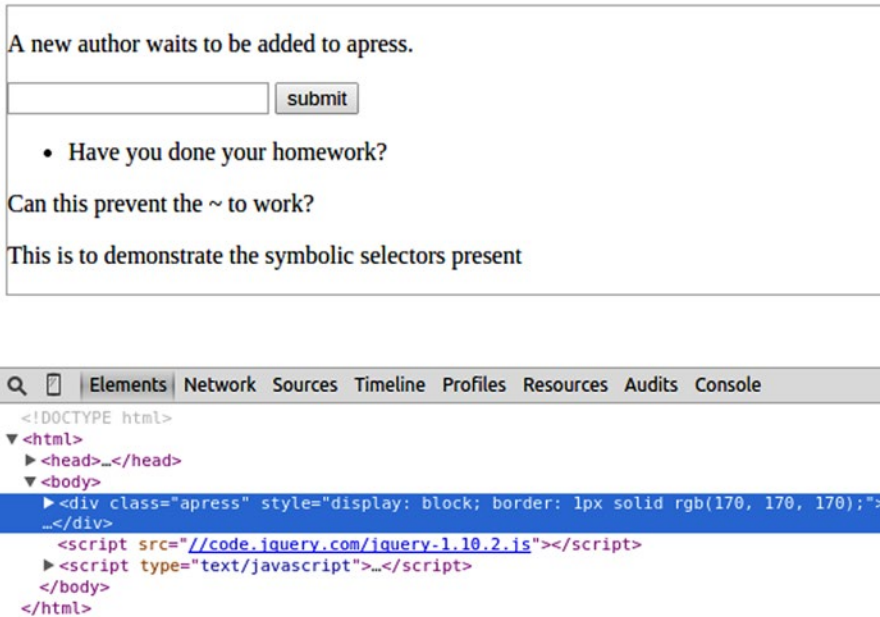
Figure 3-16. The output of .filter()
