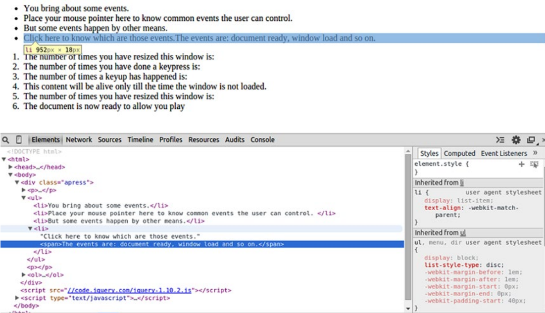
Figure 5-5. Showing mouse click event
