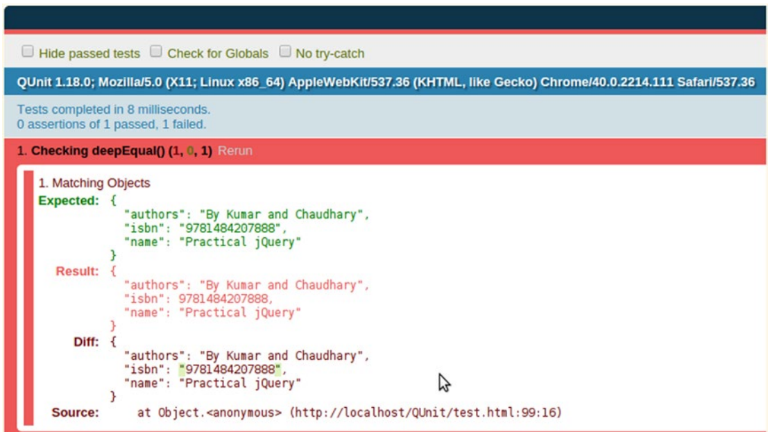
Figure 12-5. Execution of deepEqual
