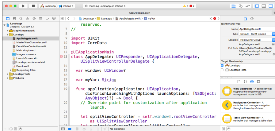
Figure 3-4: Using AppDelegate.swift .
