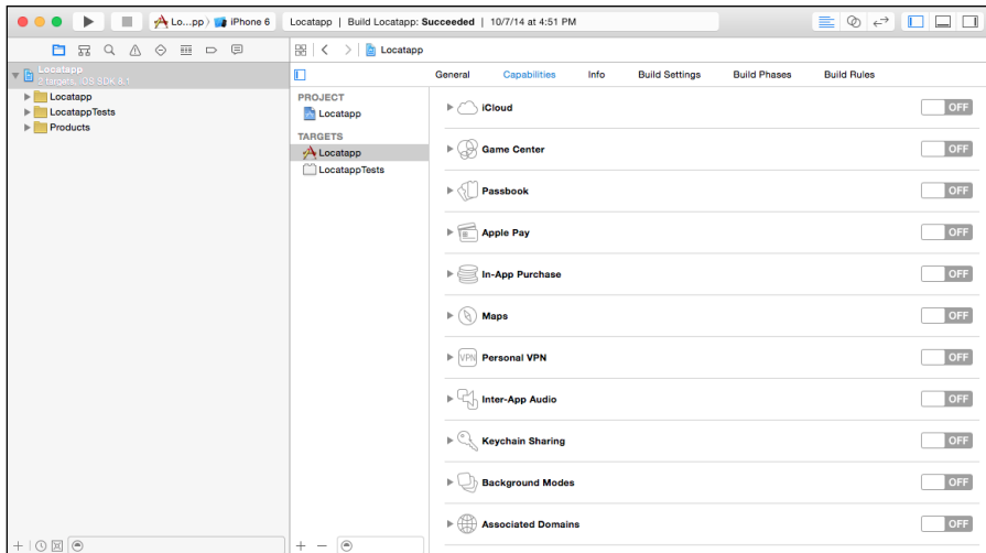
Figure 1-18: Reviewing capabilities.
