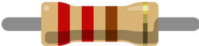
Figure 3-4. 220Ω +- 5% carbon-compound resistor
