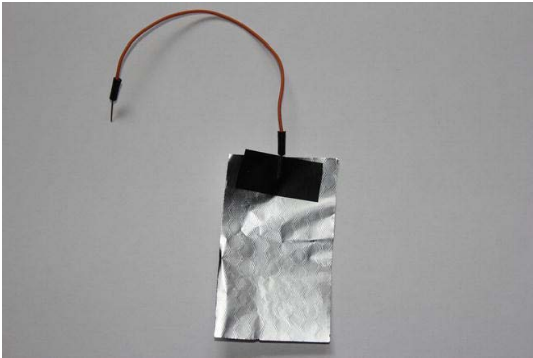
Figure 8-5. Capacitive touch sensor
