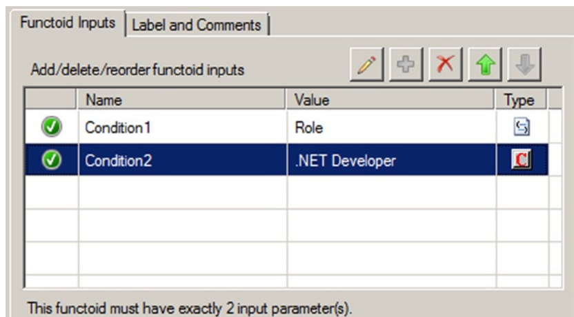
Figure 3-20. Configuring the Not Equal functoid
