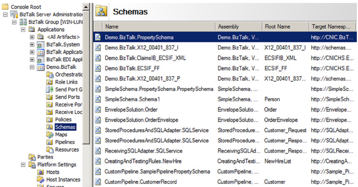
Figure 10-14. Schema resource added to an application
