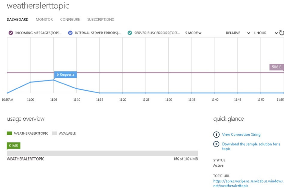
Figure 12-9. Topic details page
