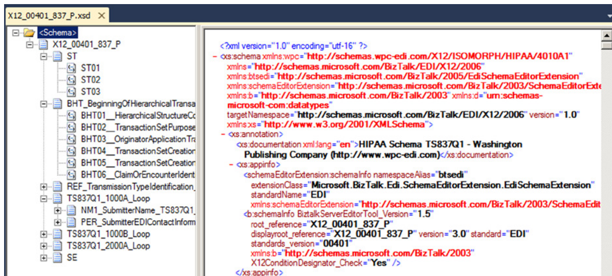
Figure 8-1. The 837 Professional schema
