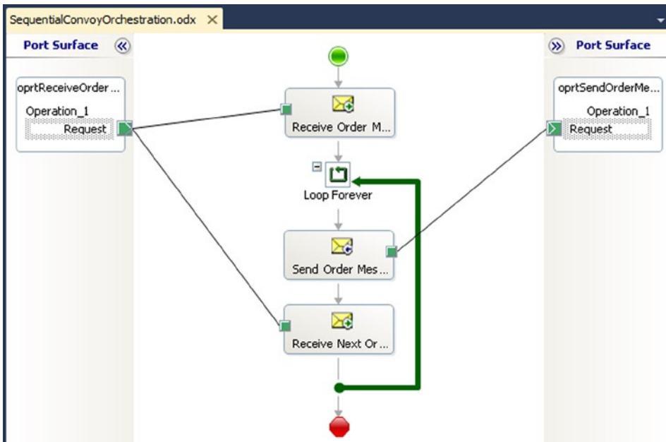
Figure 5-40. Configuring a sequential convoy
