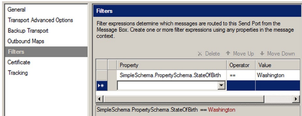
Figure 2-9. Subscription for Washington
