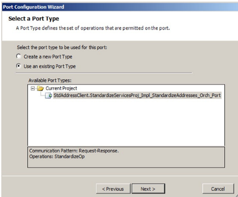
Figure 5-68. Selecting Existing Port Types
