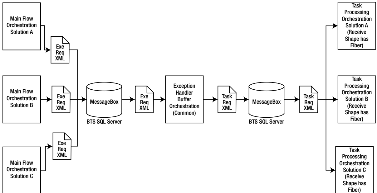
Figure 5-53. High-level architecture of the request
