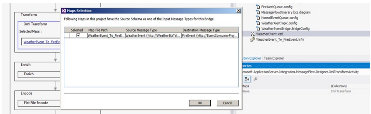
Figure 12-41. Xml One-Way Bridge—Maps Selection
