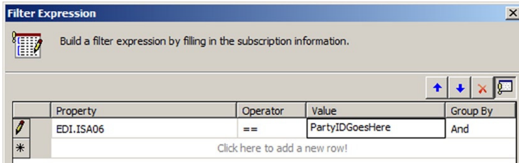
Figure 8-24. Configuring the filter on the orchestration
