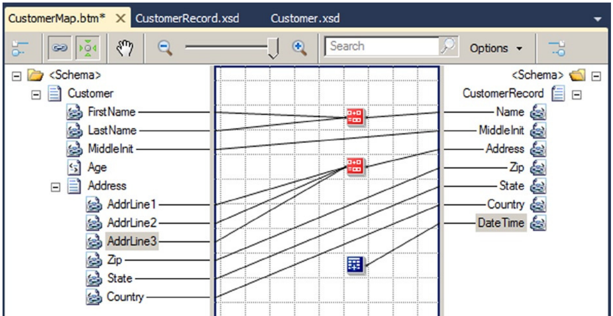
Figure 3-8. Completed customer map
