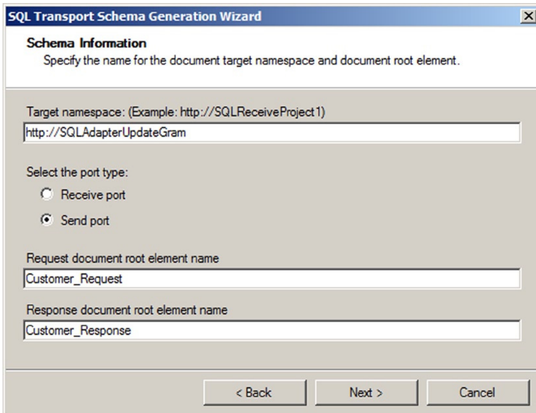
Figure 6-15. Using the SQL Transport Schema Generation Wizard
