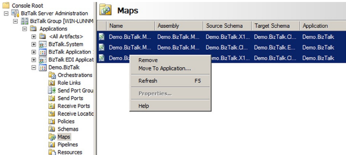
Figure 9-12. Removing maps manually
