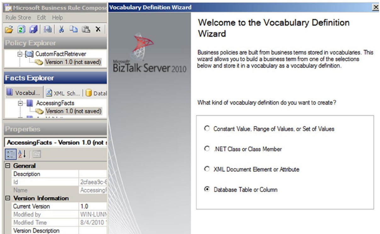
Figure 7-14. Creating a new database column definition
