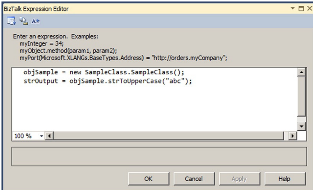
Figure 5-25. Adding code to the Expression shape
