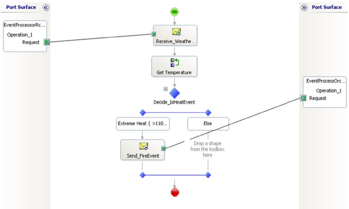
Figure 6-52. Orchestration to receive subscribed events and to send events Queue
