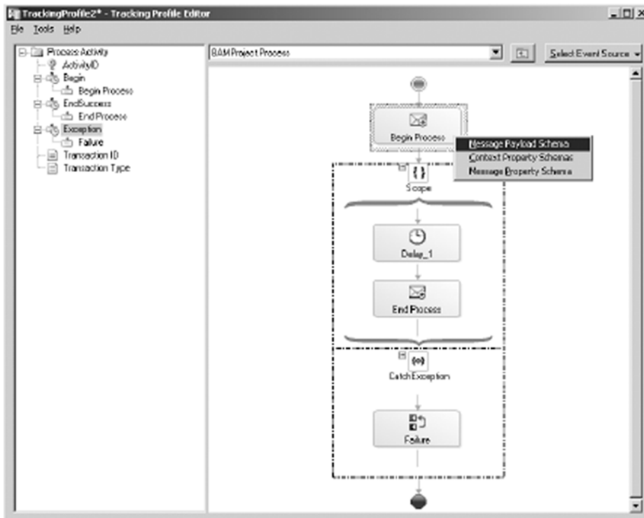
Figure 11-18. Selecting the Message Payload Schema option
