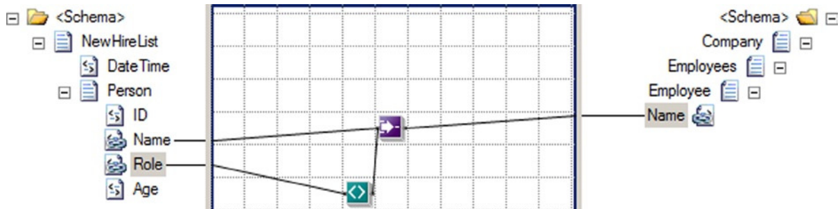
Figure 3-22. Map with Value Mapping (Flattening) functoid
