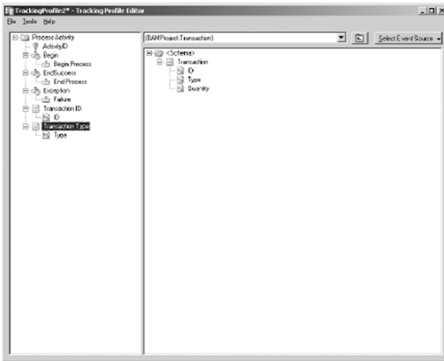
Figure 11-19. Activity definition business data mapping
