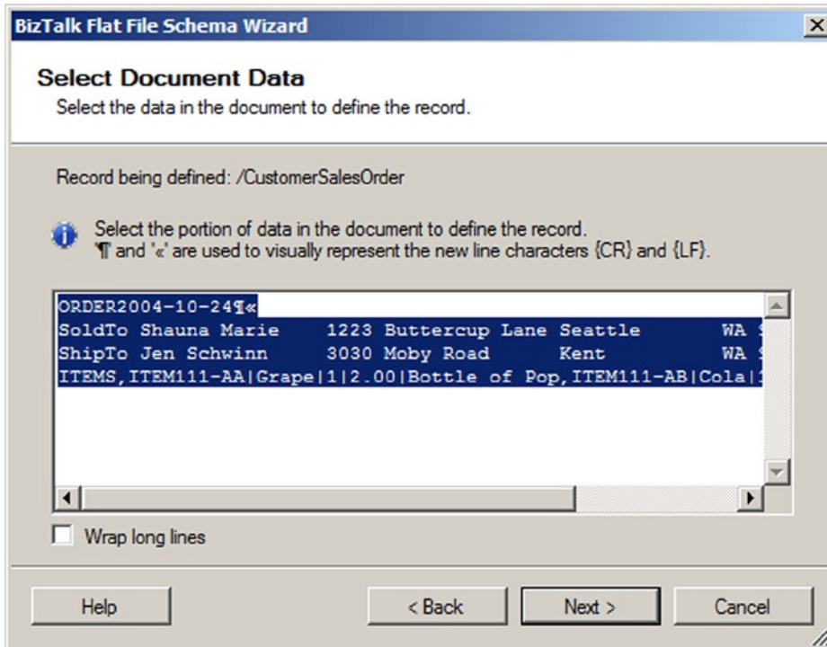
Figure 2-24. Source Document Data page
