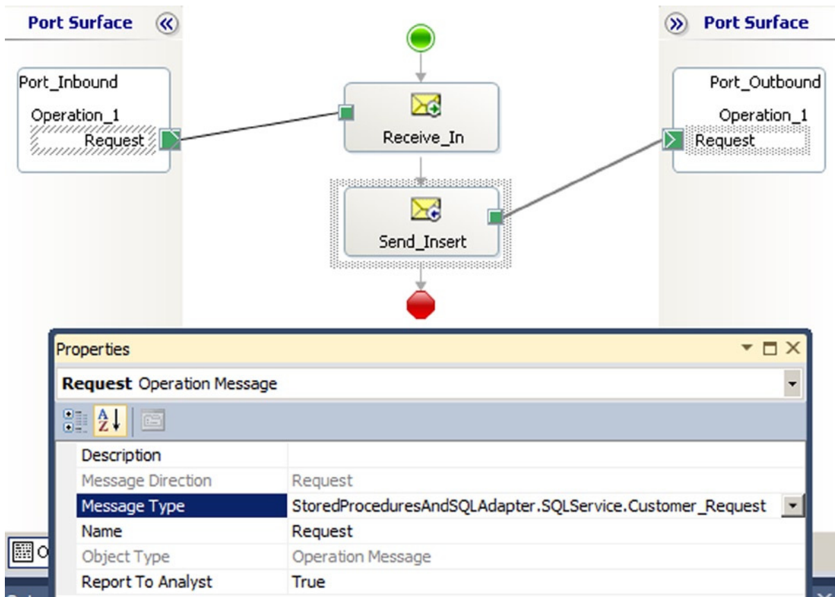
Figure 6-24. Configuring the SQL stored procedure orchestration
