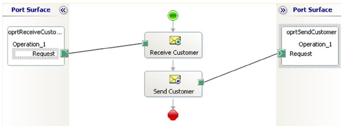
Figure 6-27. Viewing the complete orchestration
