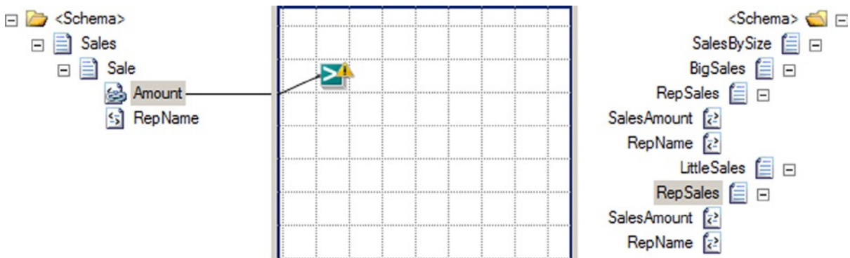
Figure 3-43. Creating the logical operator
