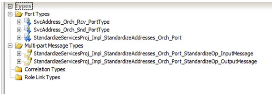
Figure 5-67. Generated Port Types and Multi-part Message Types
