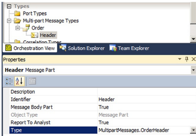
Figure 5-12. Setting the default message part's type
