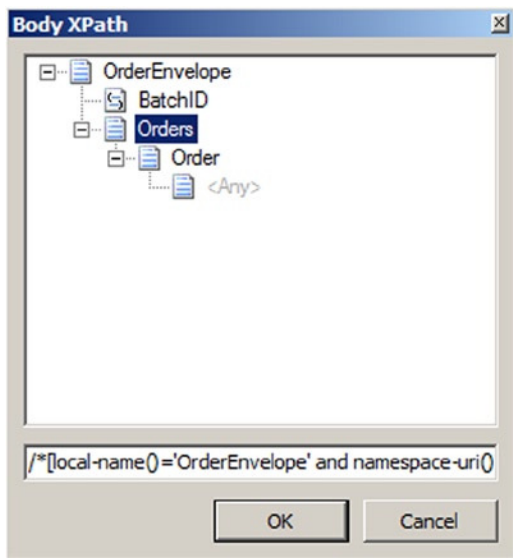
Figure 2-16. Specifying a child record
