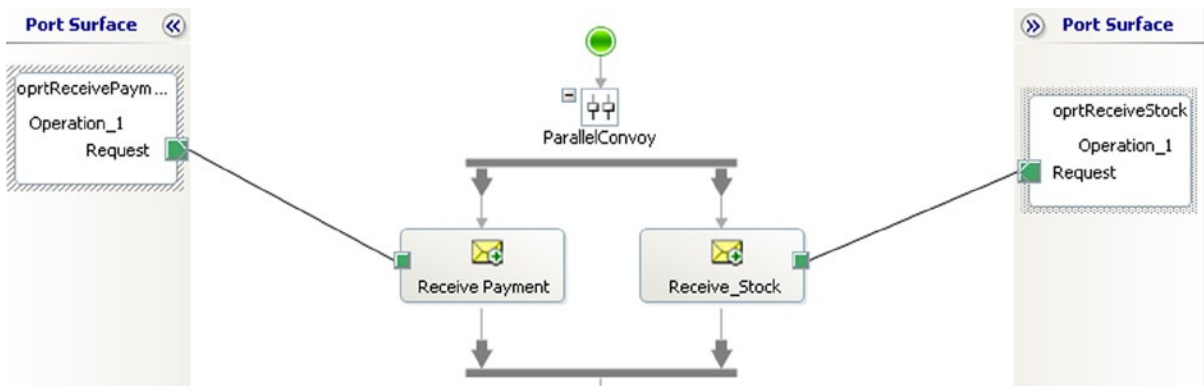
Figure 5-44. Configuring a parallel convoy
