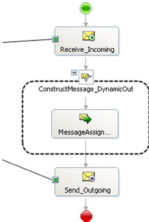
Figure 5-17. Completed dynamic send port orchestration
