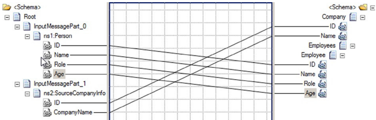
Figure 3-66. A complex map
