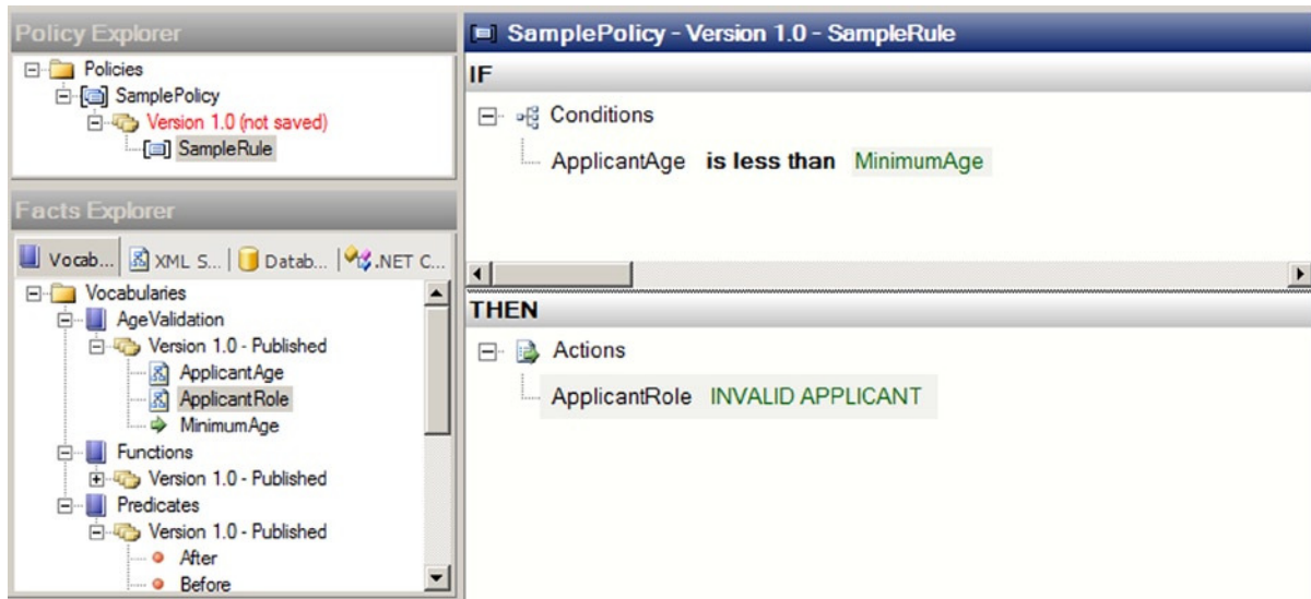
Figure 7-10. Creating the rule
