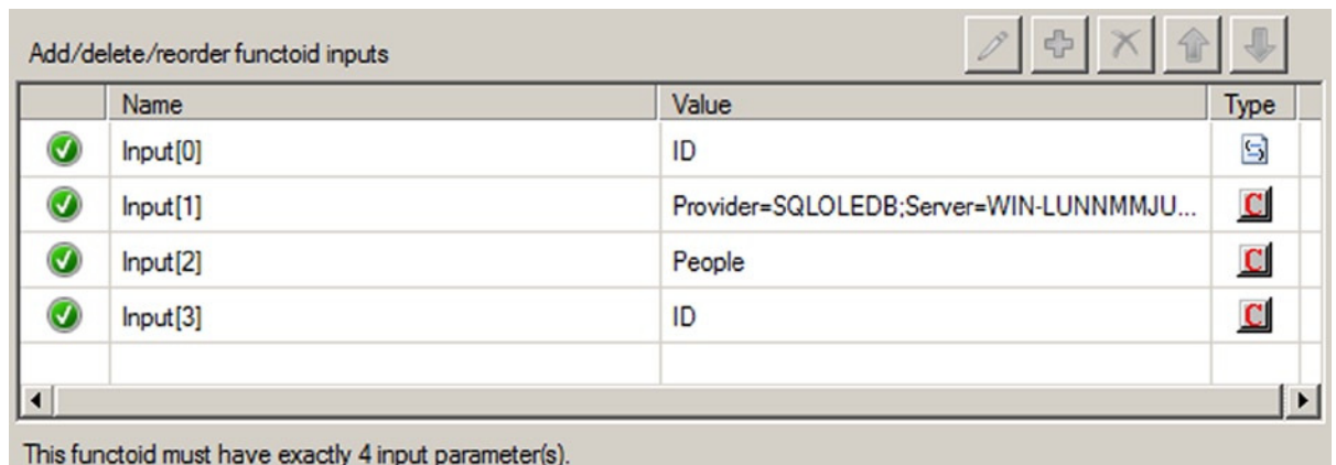
Figure 3-30. Database Lookup Functoid input parameters dialog box
