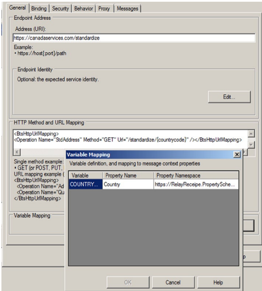
Figure 6-63. WCF-WebHttp Send Port Value Mapping Configuration
