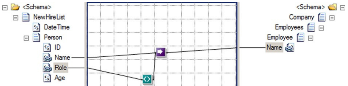
Figure 3-21. Using the Value Mapping functoid
