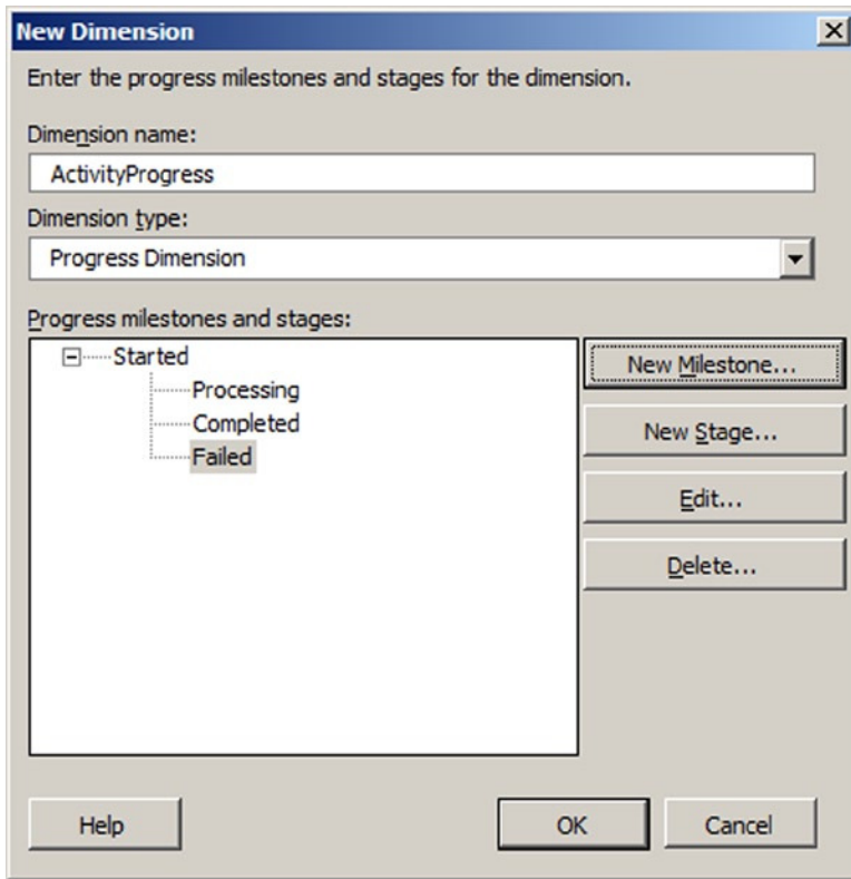
Figure 11-6. Finishing the progress dimension
