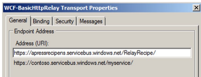
Figure 12-23. Configuring WCF-BasicHttpRelay Transport Properties—General tab
