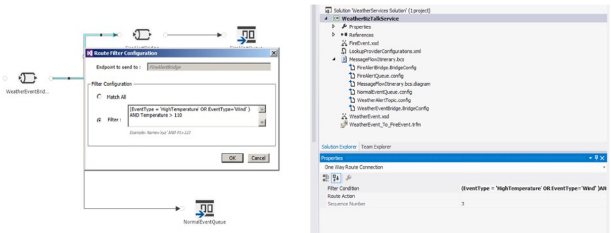
Figure 12-43. Route Filter Configuration
