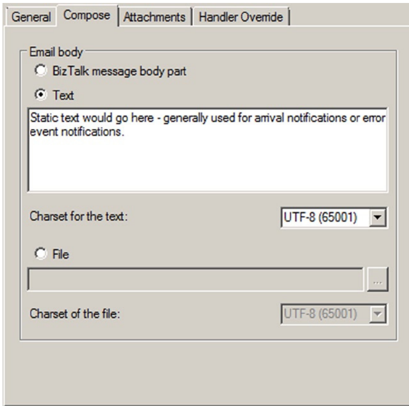
Figure 6-7. Configuring the Compose tab
