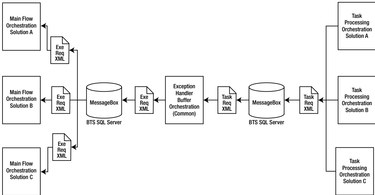
Figure 5-54. High-level architecture of the response
