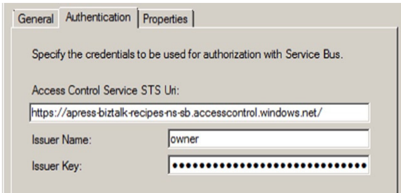
Figure 6-54. Receive Location's Authentication Tab
