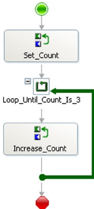
Figure 5-26. Loop shape with counter
