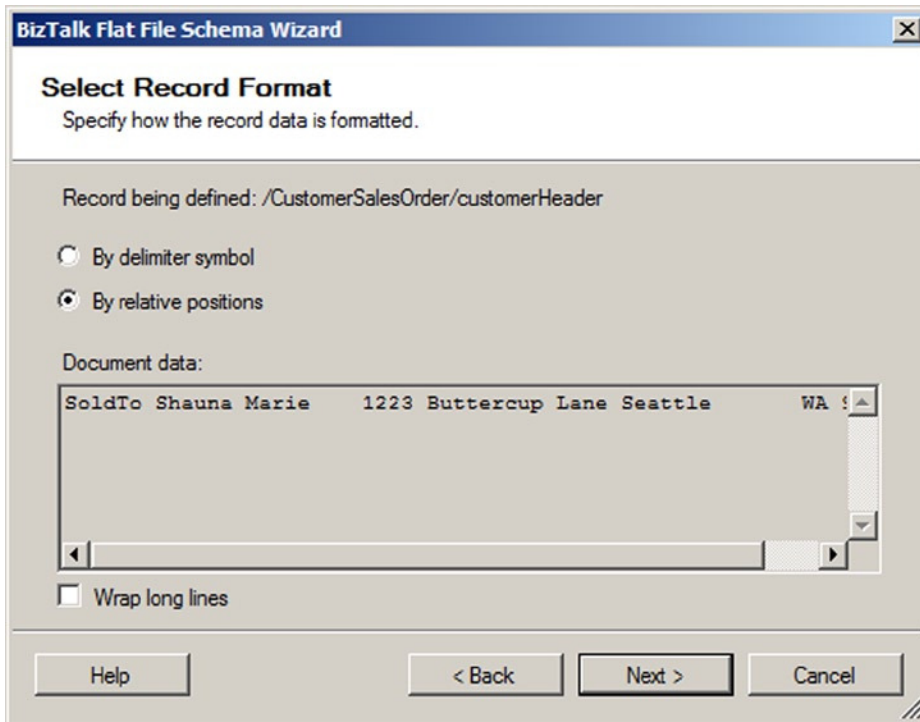
Figure 2-30. Record format—customer header
