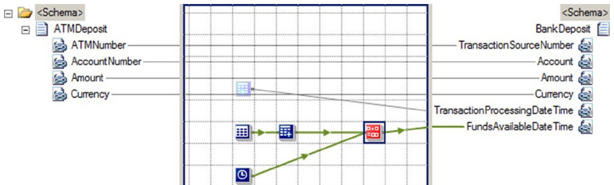
Figure 3-42. Using the Time functoid
