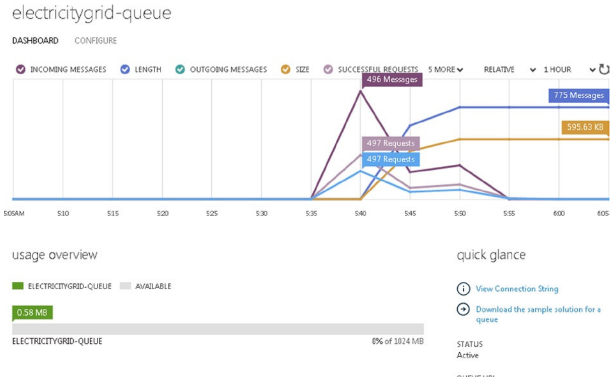
Figure 10-33. Dashboard for a Service Bus Queue
