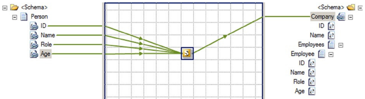
Figure 3-61. Scripting/XSLT call template in a map
