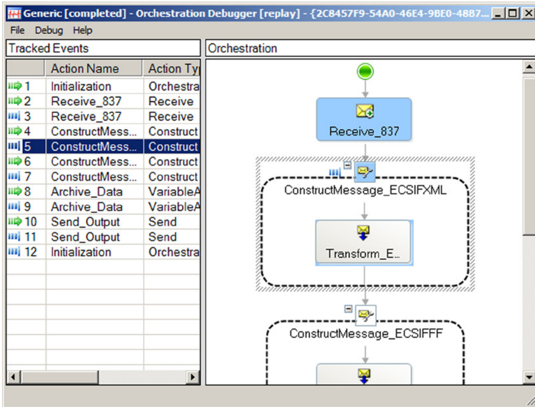
Figure 10-17. Orchestration Debugger window
