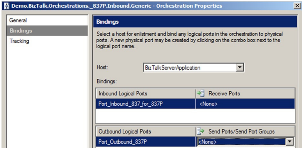
Figure 5-16. Port Bindings Properties dialog box
