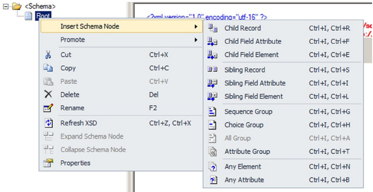
Figure 2-3. Adding schema nodes
