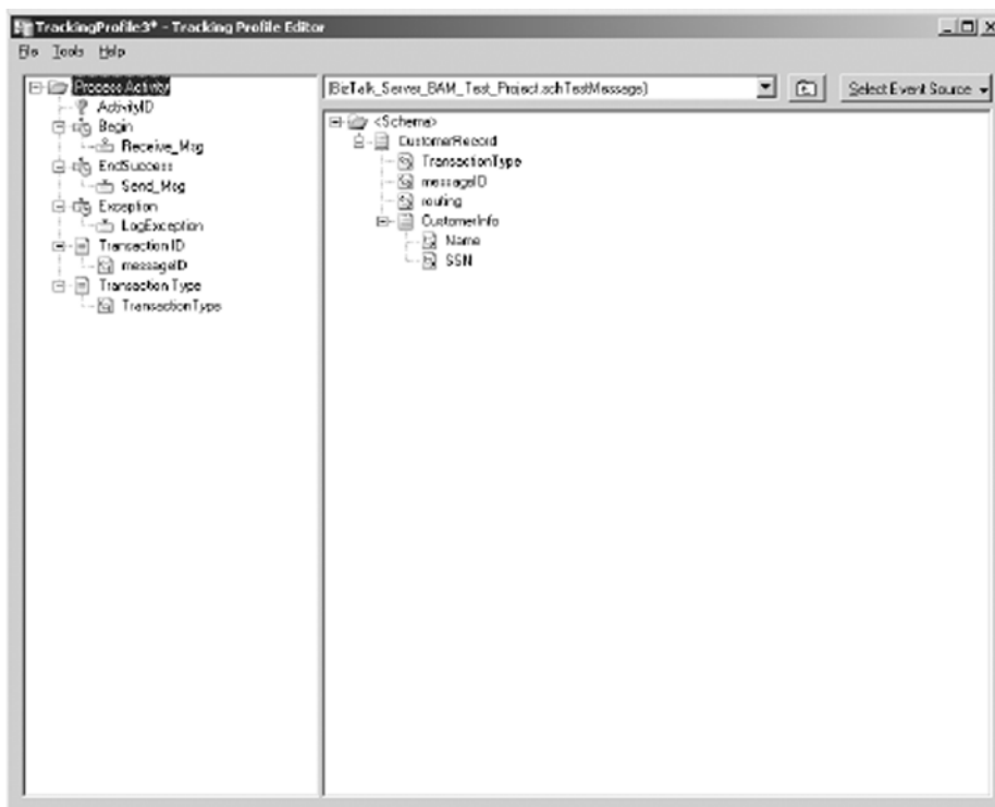
Figure 11-36. Completed mapped activity
