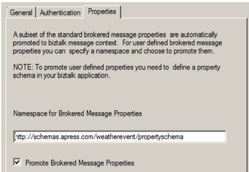
Figure 6-55. Receive Location's Properties Tab
