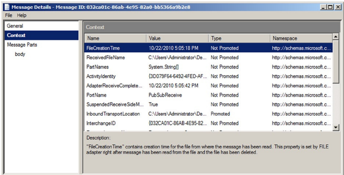
Figure 10-28. Message context properties
