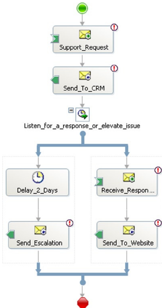
Figure 5-33. Defining the message flow
