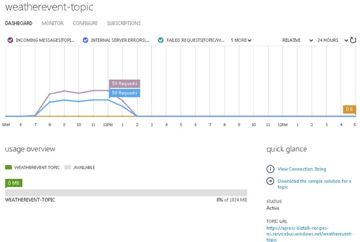
Figure 10-39. Dashboard for a Service Bus Topic
