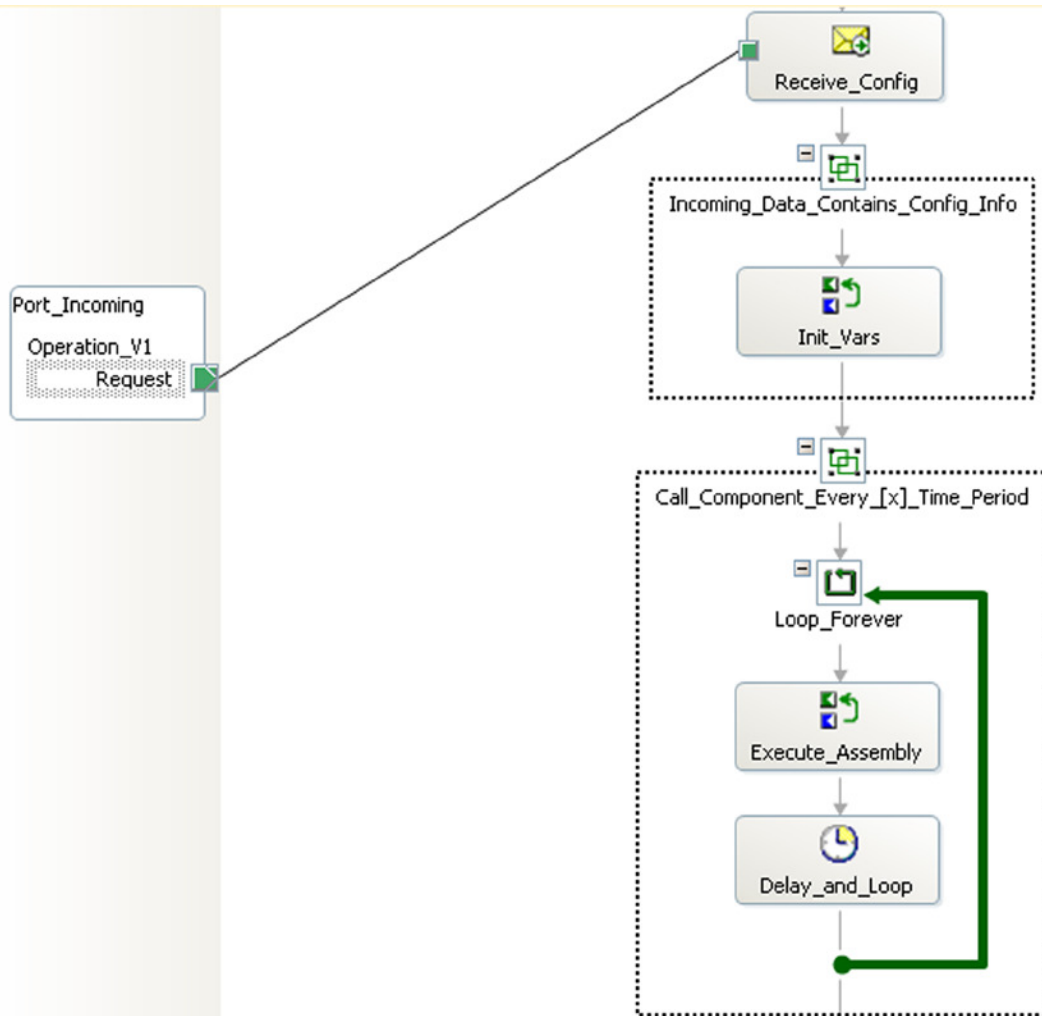
Figure 5-27. Long-running polling orchestration
