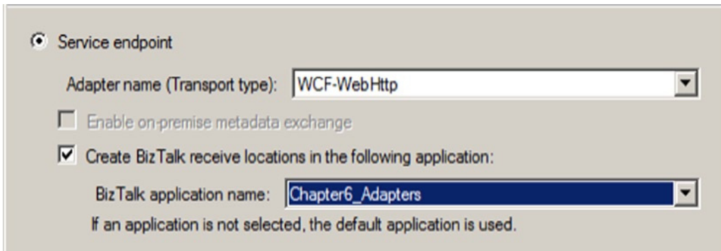
Figure 6-61. WCF Publishing Wizard with WCF-WebHttp Configuration
