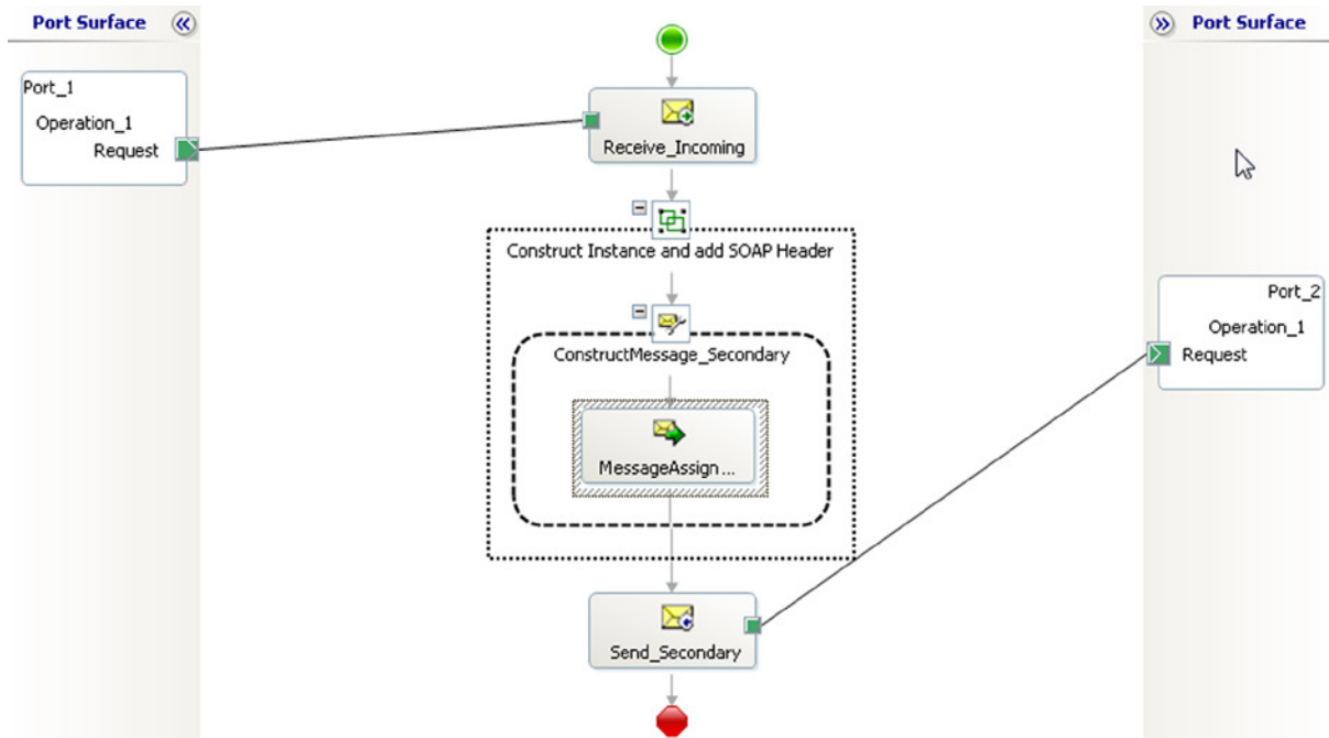
Figure 2-46. Sample solution primary orchestration
