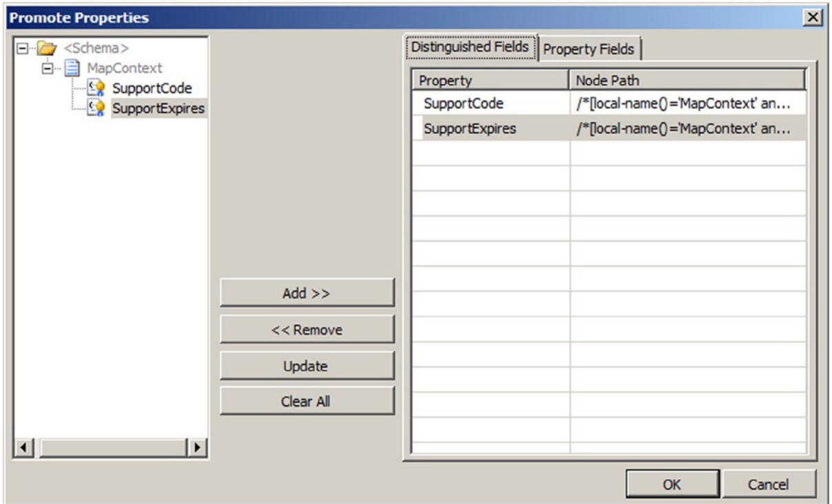
Figure 3-53. Designating the distinguished fields
