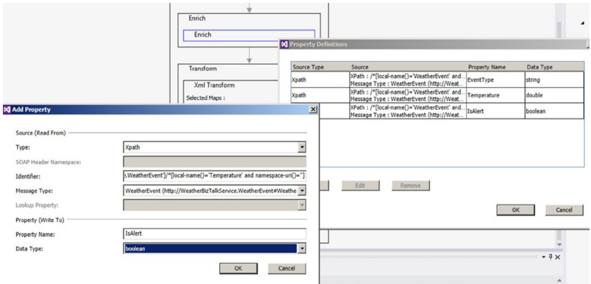
Figure 12-40. Xml One-Way Bridge—Property Definitions
