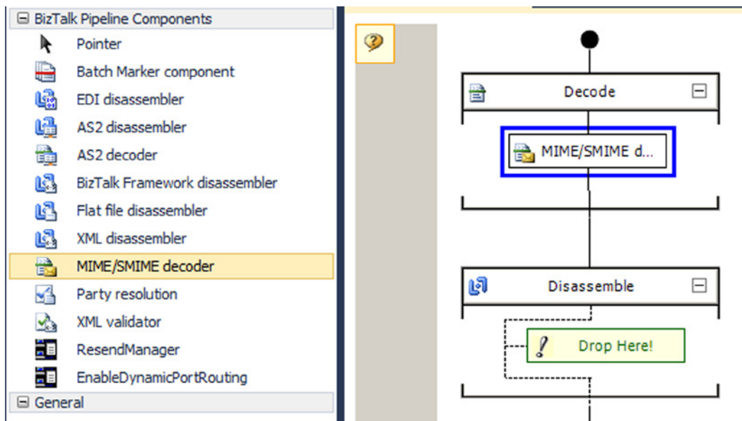
Figure 4-12. Adding the MIME/SMIME decoder
