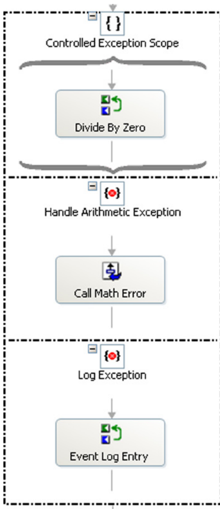
Figure 5-49. Defining arithmetic exception-specific shapes
