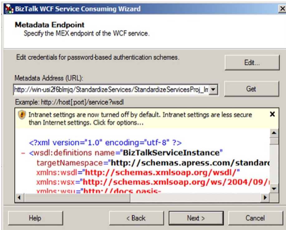
Figure 5-64. WCF Service Consuming Wizard Metadata Endpoint Screen
