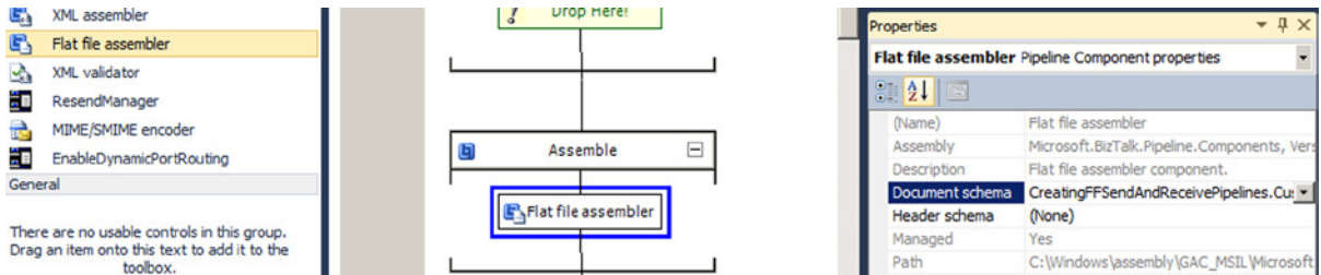
Figure 4-19. Configuring a send pipeline
