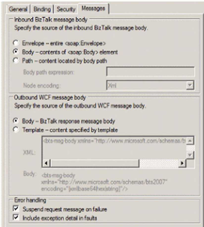
Figure 6-46. WCF-WSHttp Request Response Location – Messages Tab
