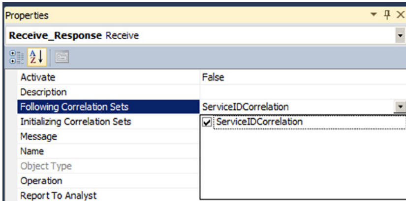
Figure 5-39. Following the initialized correlation set
