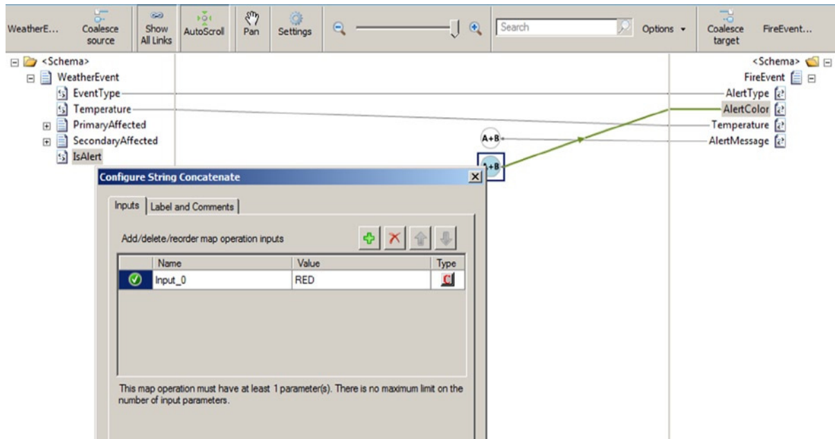
Figure 12-36. BizTalk Services mapper
