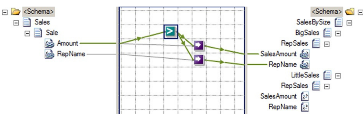
Figure 3-45. Defining conditional mapping actions
