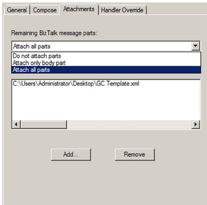
Figure 6-8. Setting the SMTP attachment
