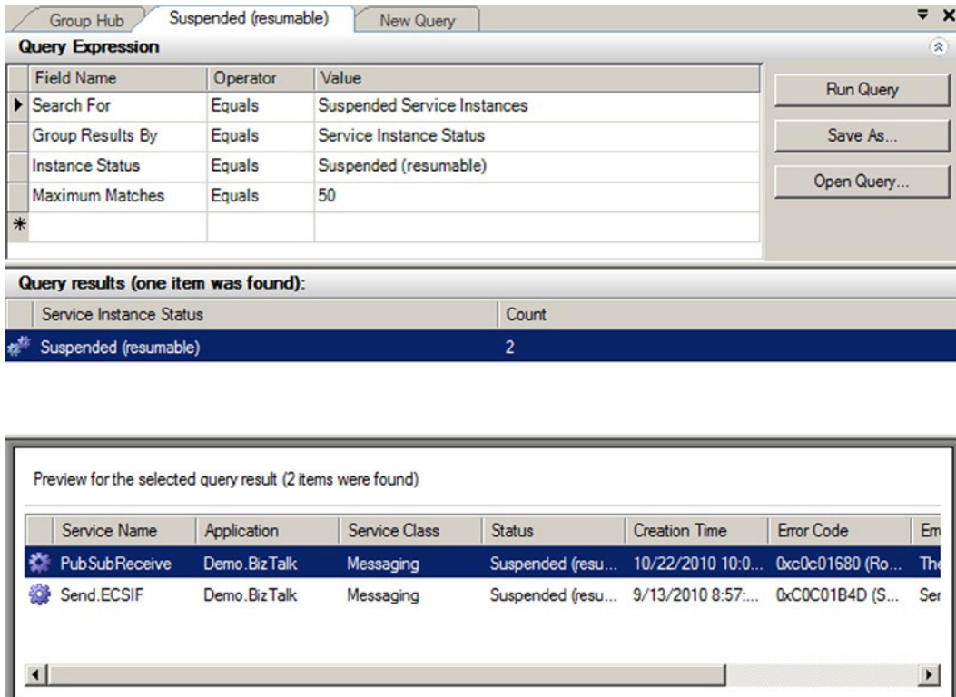
Figure 10-25. Resumable service instance
