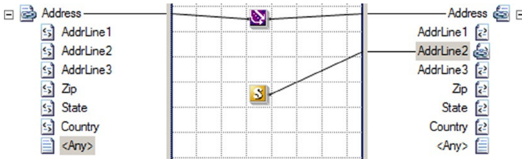
Figure 3-19. Overriding AddrLine2 within a Mass Copy functoid
