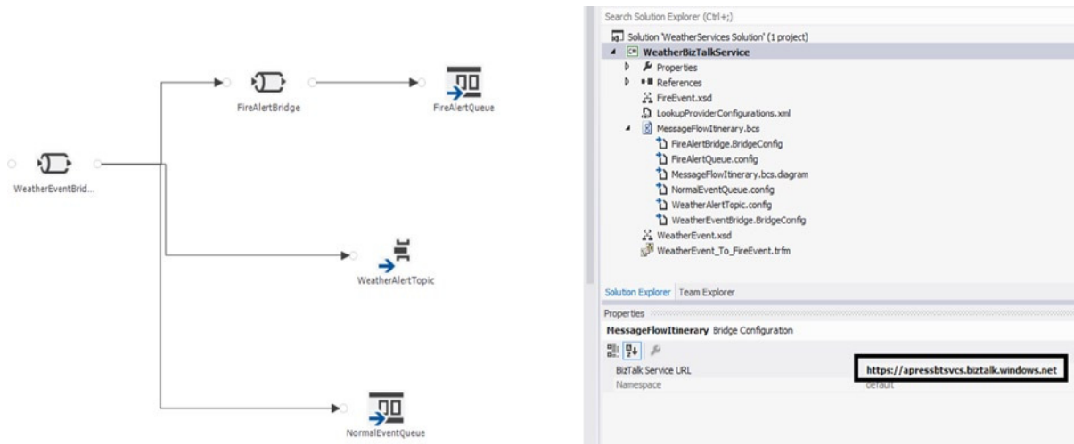
Figure 12-44. BizTalk Service URL setup
