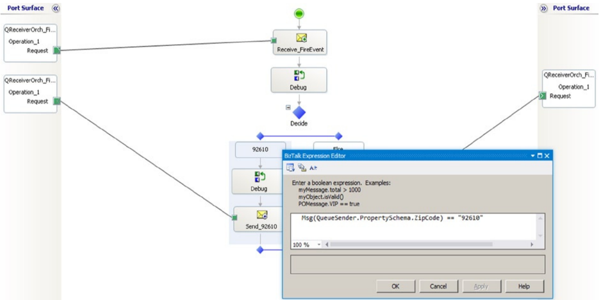
Figure 12-20. Orchestration-based routing with Brokered Message Properties
