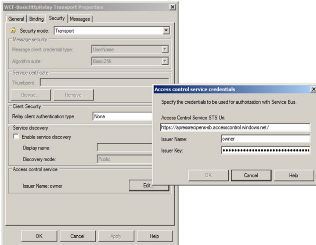
Figure 12-24. Configuring WCF-BasicHttpRelay Transport Properties—Security tab)
