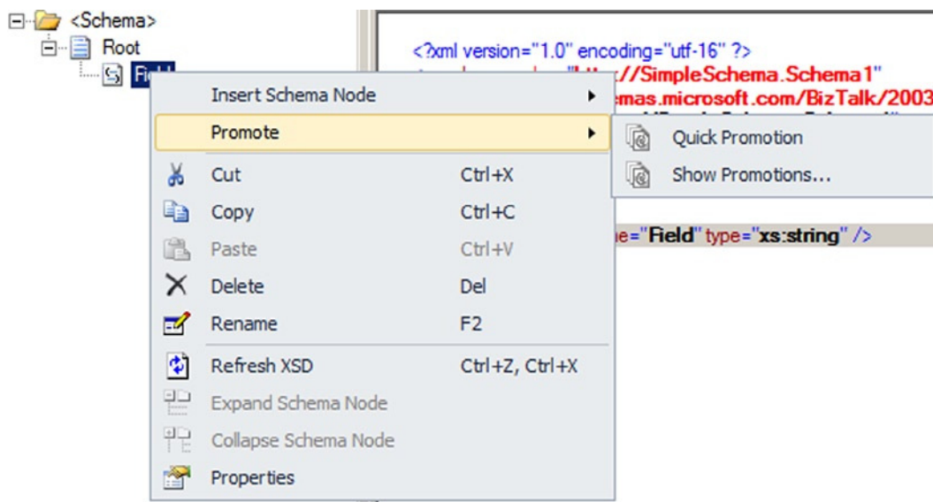
Figure 2-7. Completing a quick promotion of a property
