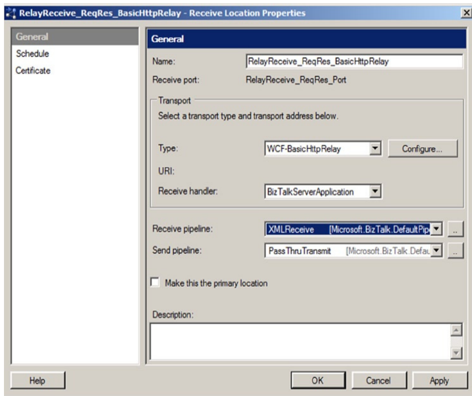
Figure 12-22. General settings for the receive location
