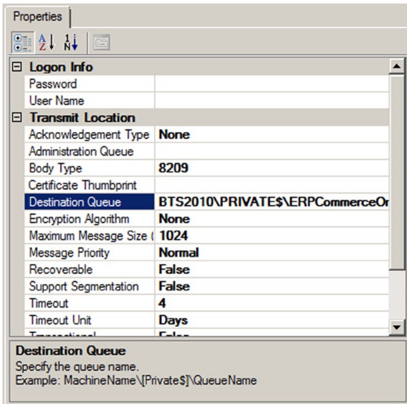
Figure 6-11. Configuring an MSMQ send port
