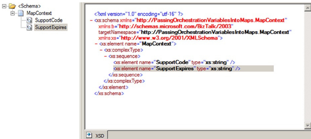
Figure 3-52. Defining the context message schema
