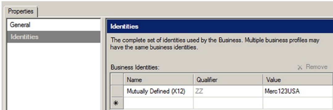
Figure 8-8. Setting a business profile's identities
