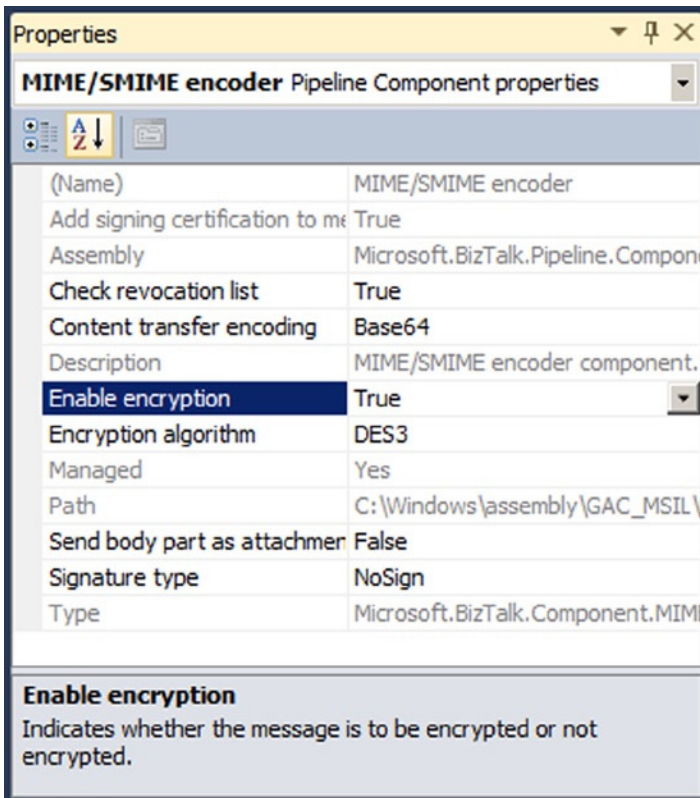
Figure 4-11. Enabling pipeline encryption
