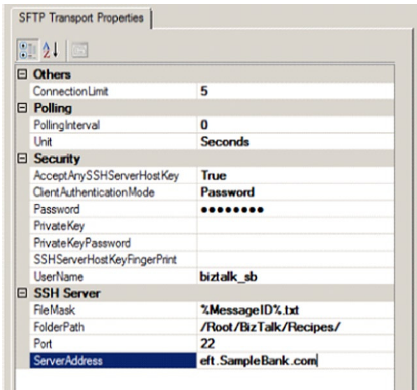
Figure 6-41. Configuring an SFTP receive location
