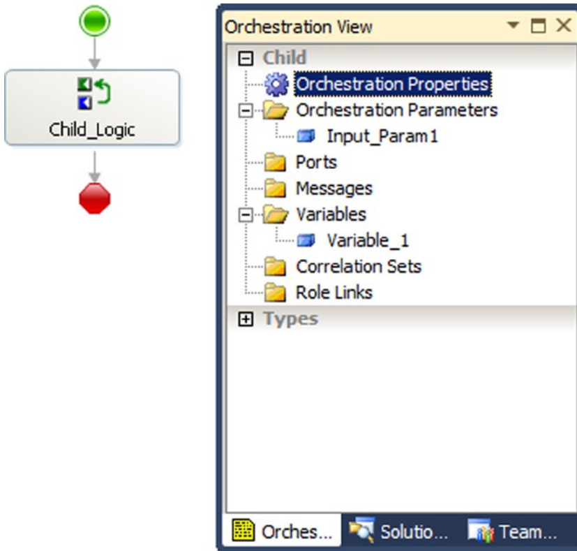
Figure 5-32. Configuring a callable orchestration
