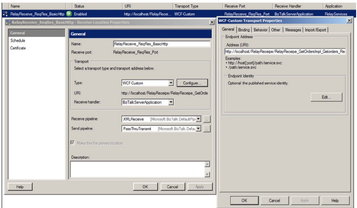
Figure 12-21. Receive location for on-premise WCF service
