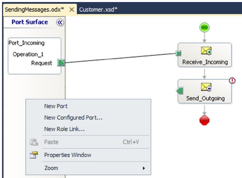
Figure 5-7. Creating a new port
