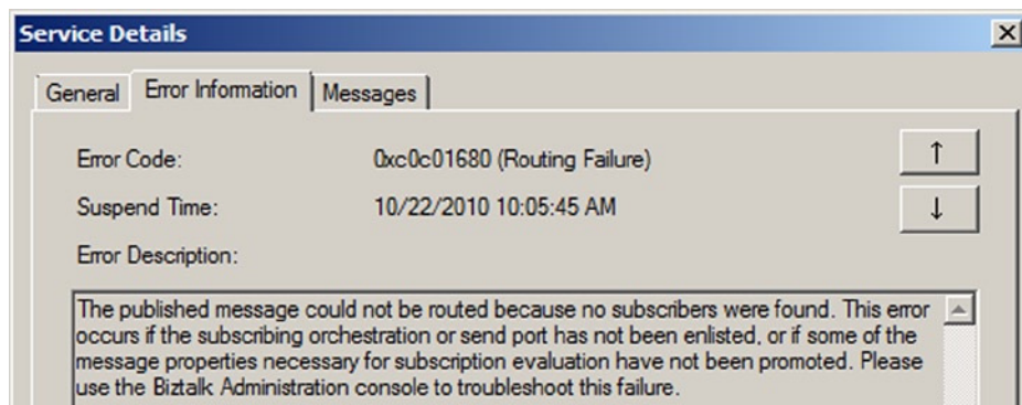
Figure 10-27. Viewing error information
