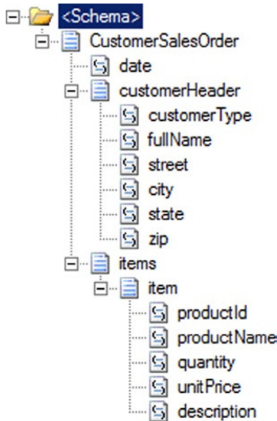
Figure 2-40. The finished schema
