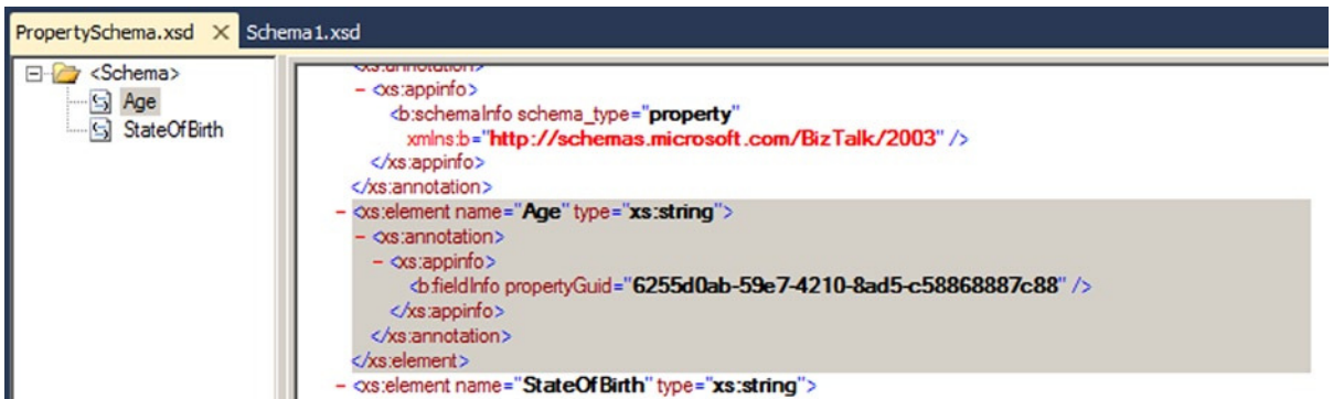
Figure 2-11. Adding a property to message context
