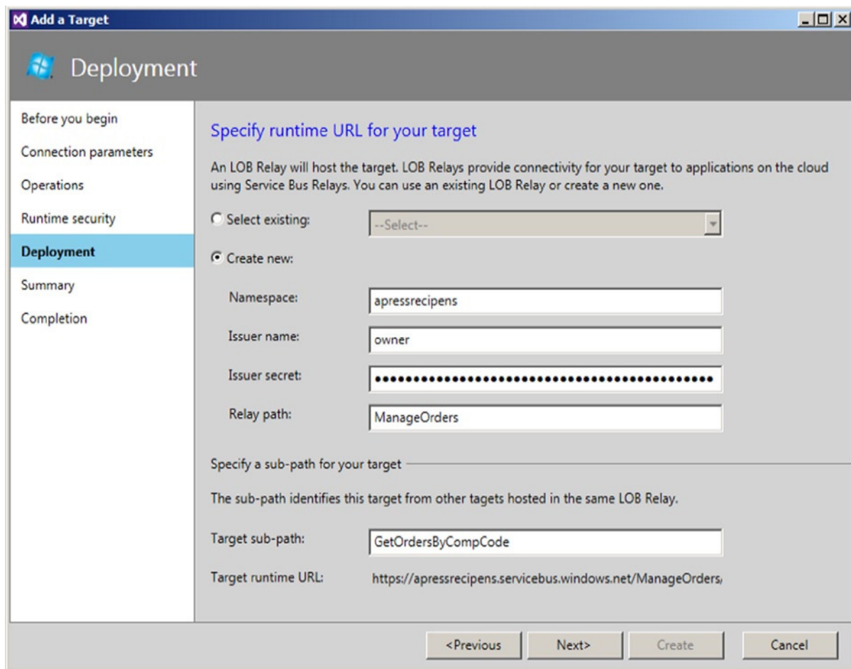
Figure 12-50. Add a Target—Deployment
