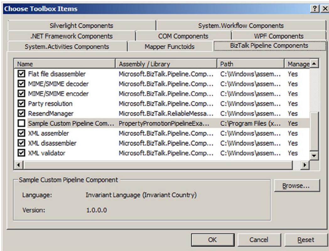
Figure 4-23. Adding a custom pipeline component to the toolbox
