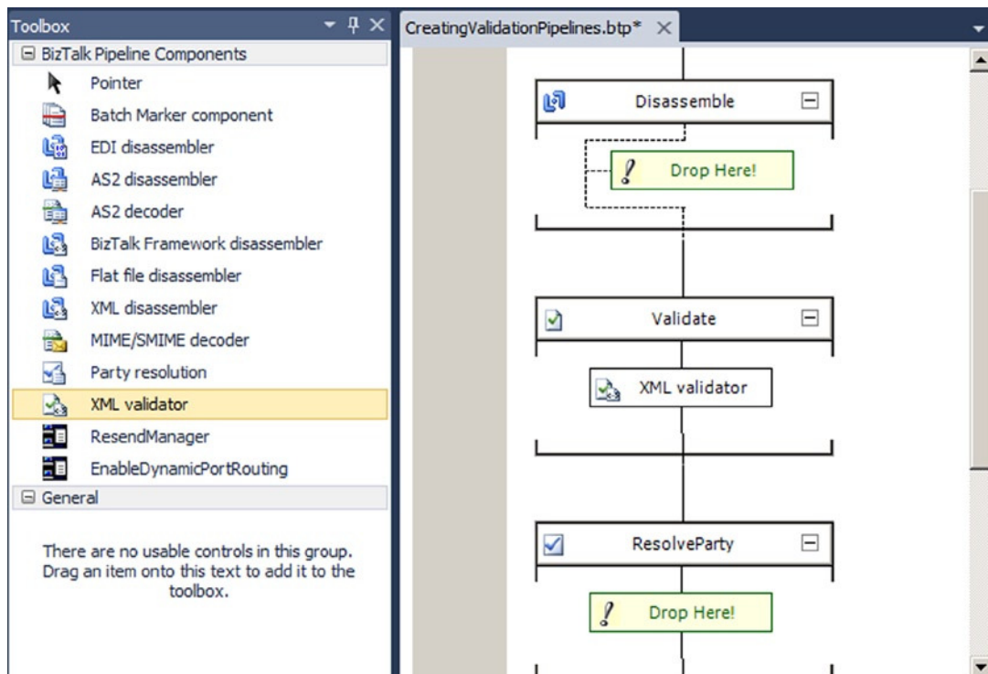
Figure 4-7. Creating an XML validator pipeline
