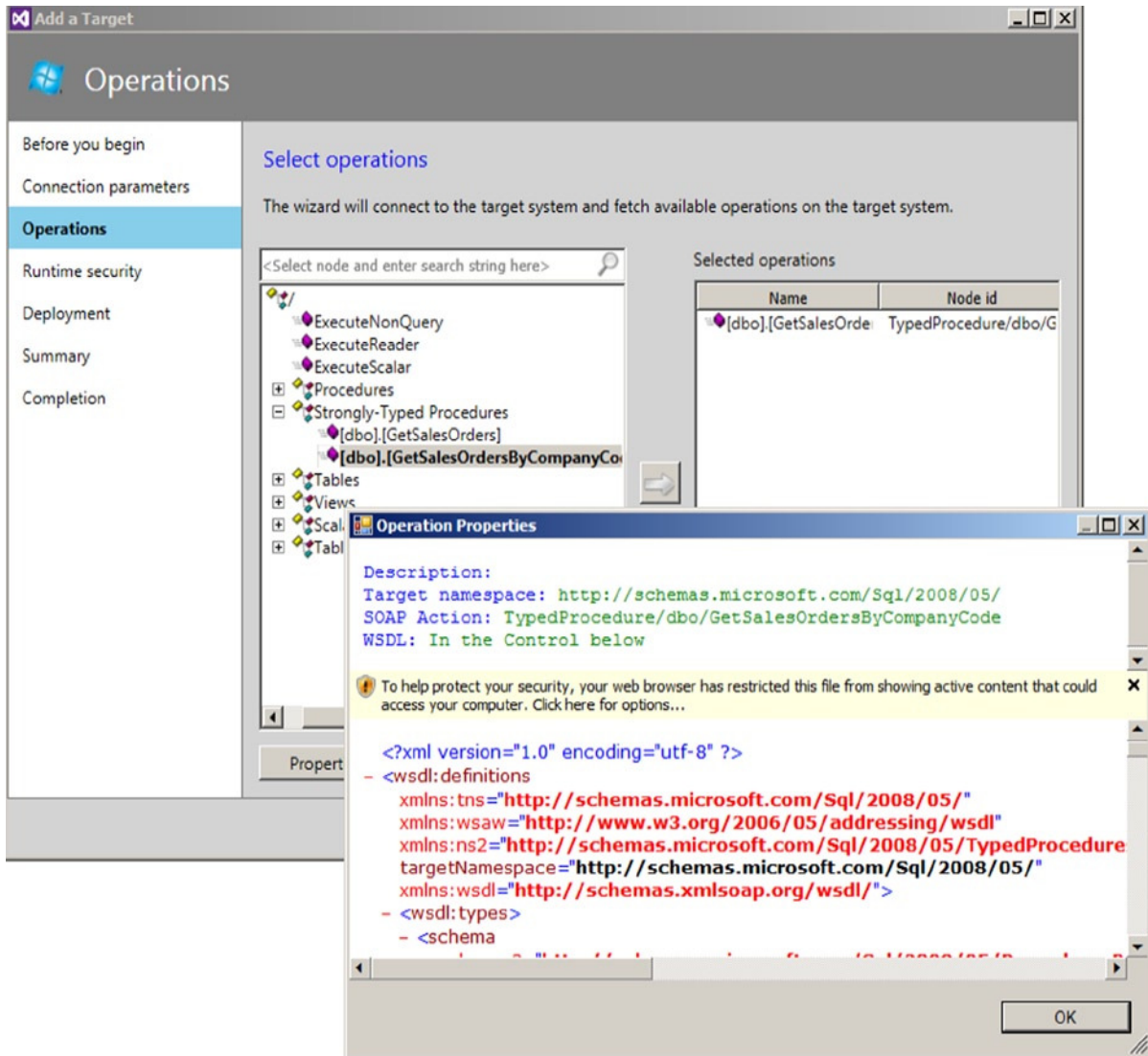
Figure 12-48. Add a Target—Operations
