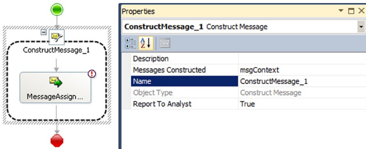
Figure 3-55. The Construct Message
