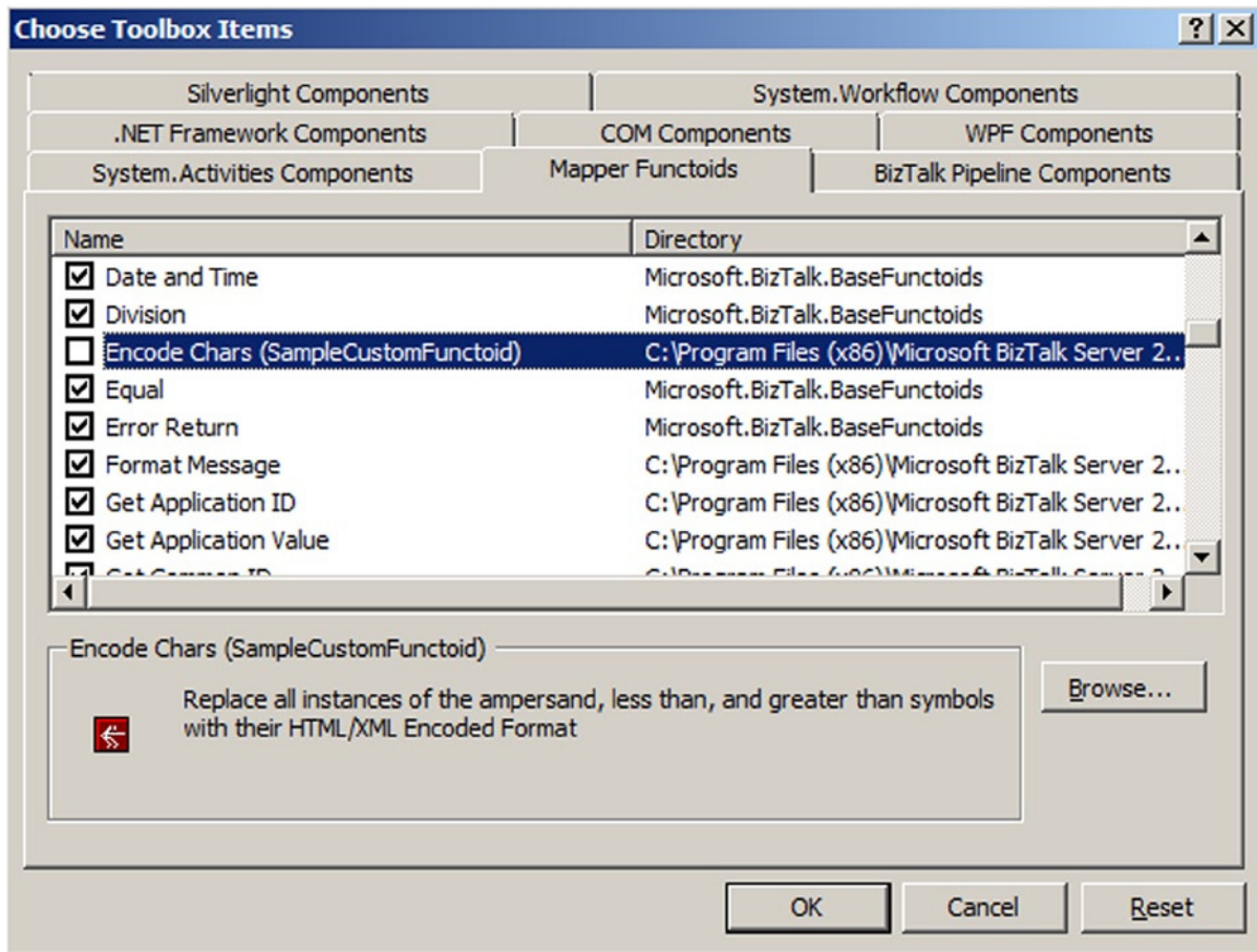
Figure 3-38. Adding a custom functoid to the Toolbox
