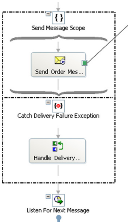
Figure 5-43. Capturing delivery failure exceptions
