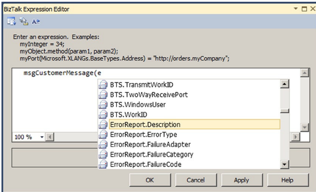
Figure 4-28. Accessing the ErrorReport properties
