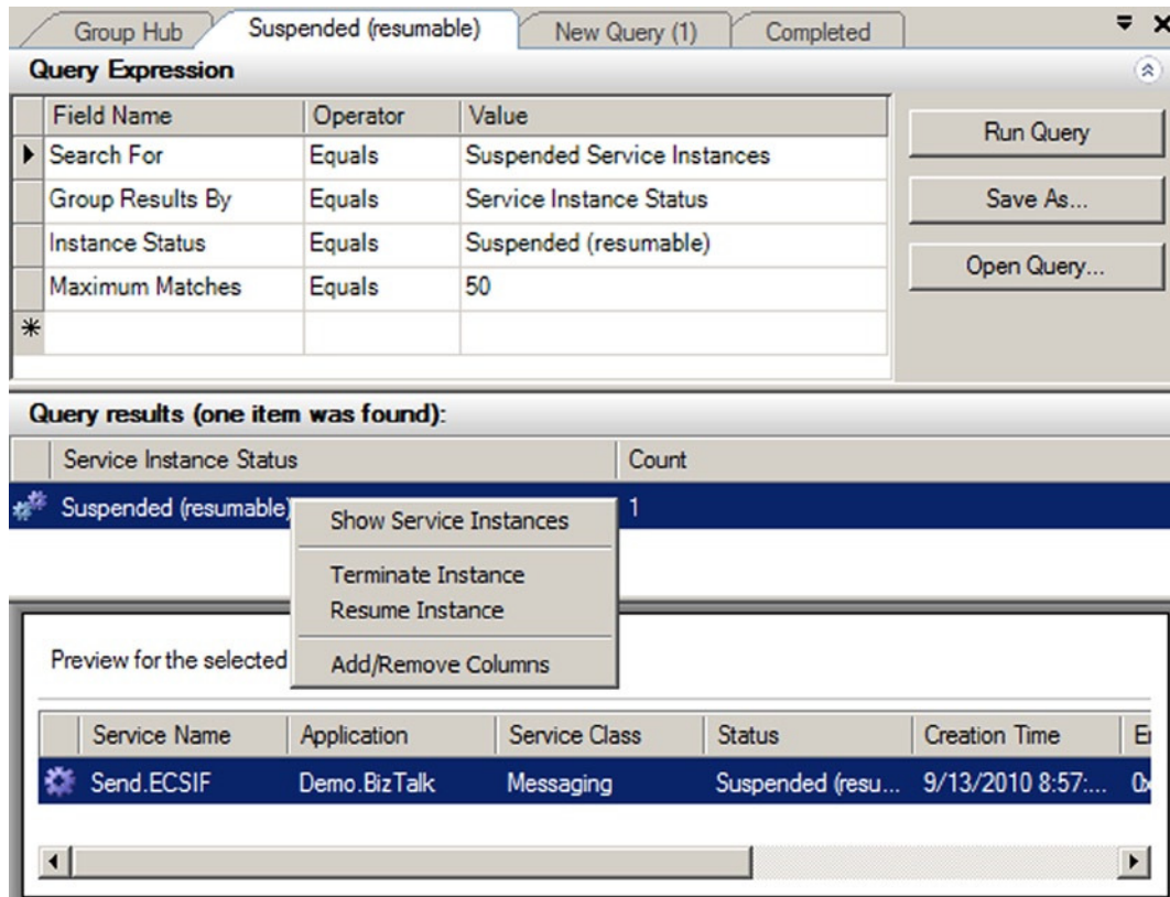
Figure 10-9. Resuming a single suspended instance
