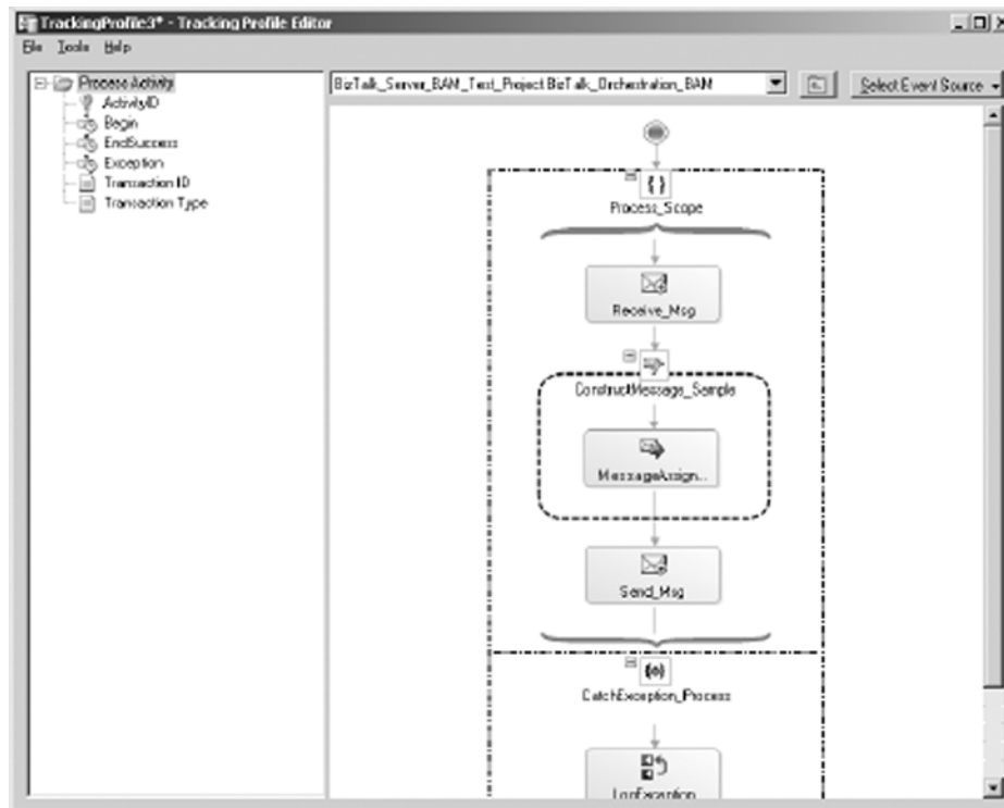
Figure 11-35. Completed Event Source Wizard
