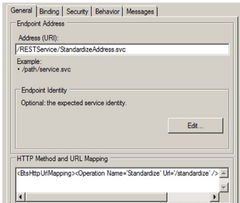
Figure 6-62. WCF-WebHttp Receive Location General Tab
