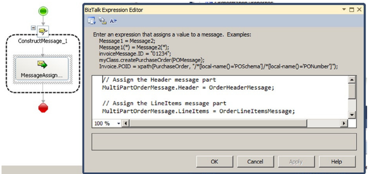
Figure 5-15. Assigning message parts
