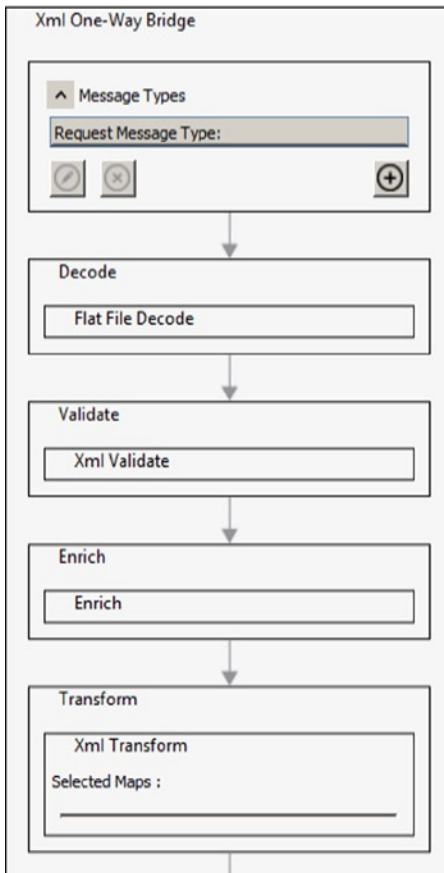
Figure 12-38. Xml One-Way Bridge
