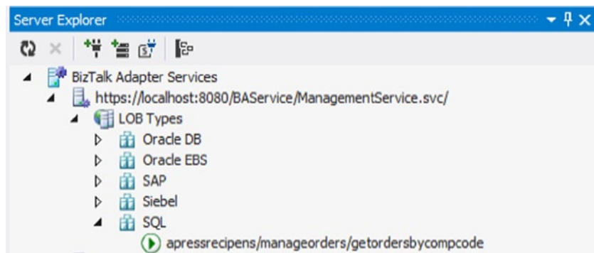
Figure 12-51. Server Explorer—SQL LOB Target
