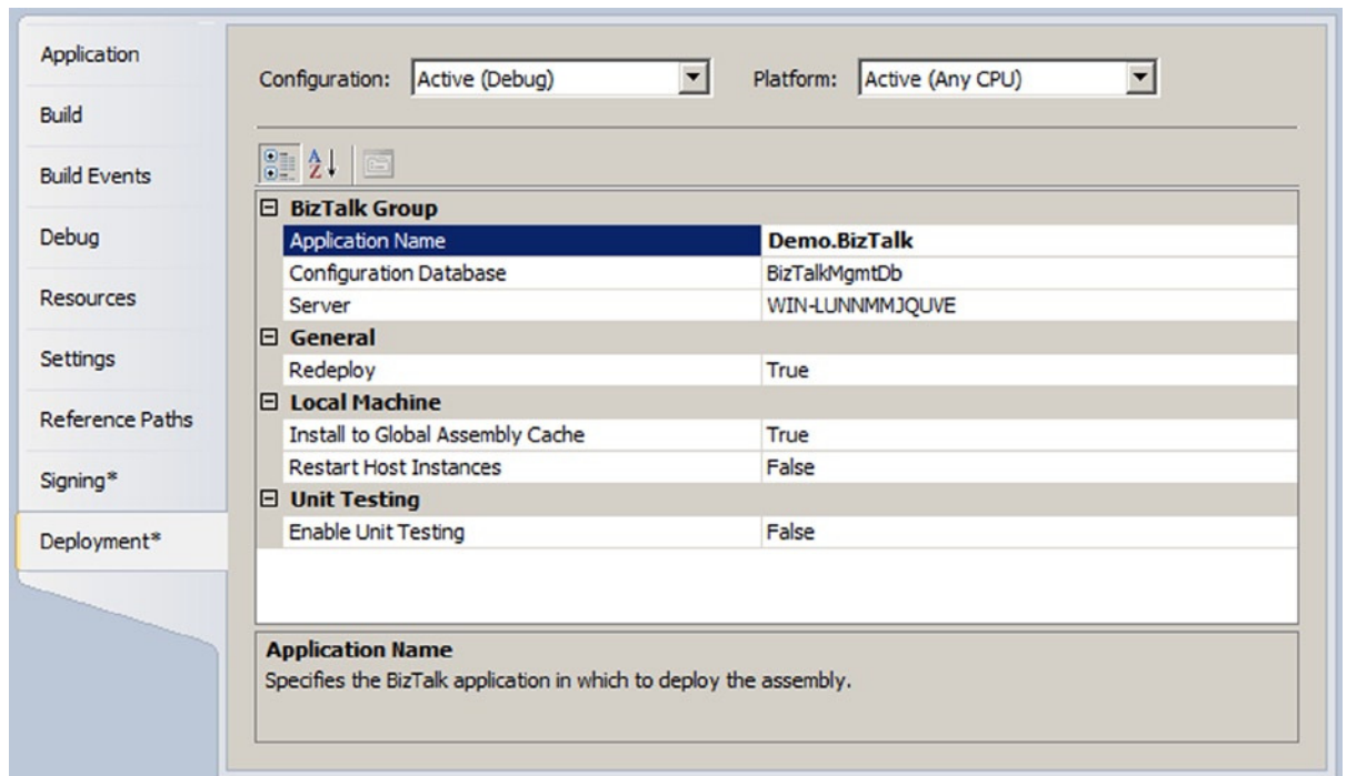
Figure 9-15. Setting deployment properties
