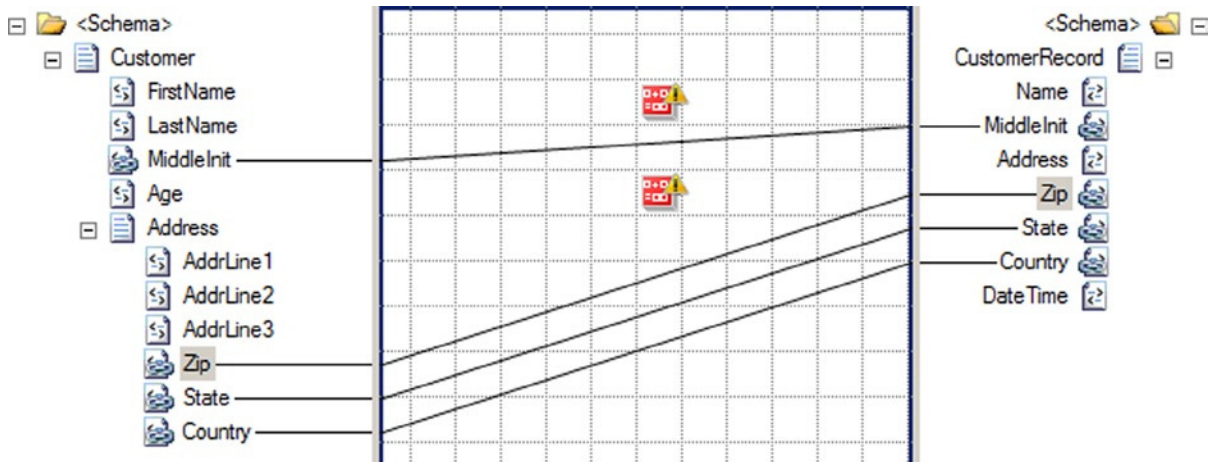
Figure 3-4. String Concatenate functoids on the design surface
