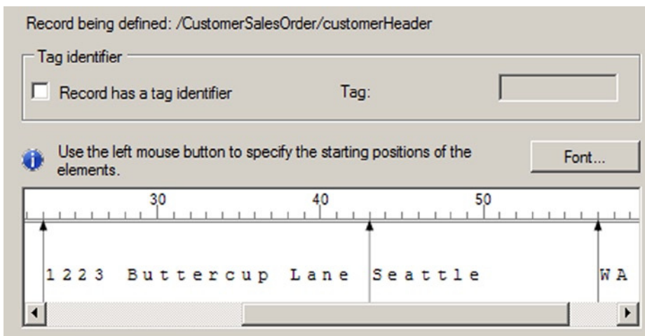
Figure 2-31. Specifying the positional record
