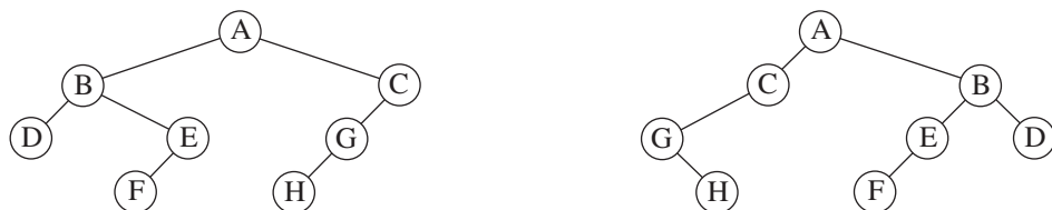
Figure 4.78 Two isomorphic trees
