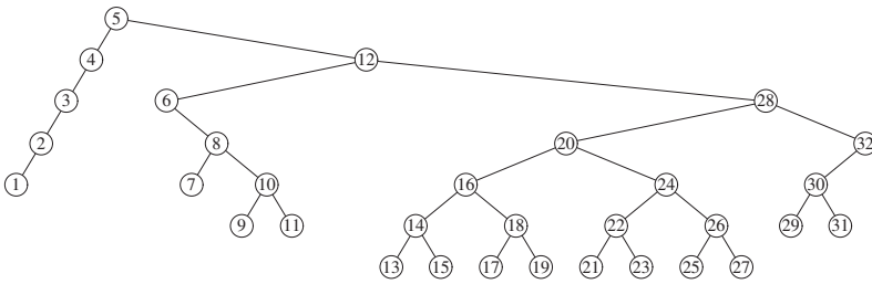
Figure 4.55 Result of splaying the previous tree at node 5
