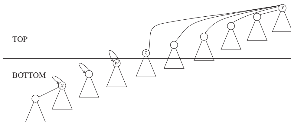
Figure 8.24 Recursive decomposition, case 3: The bottom node new parents are the nodes themselves
