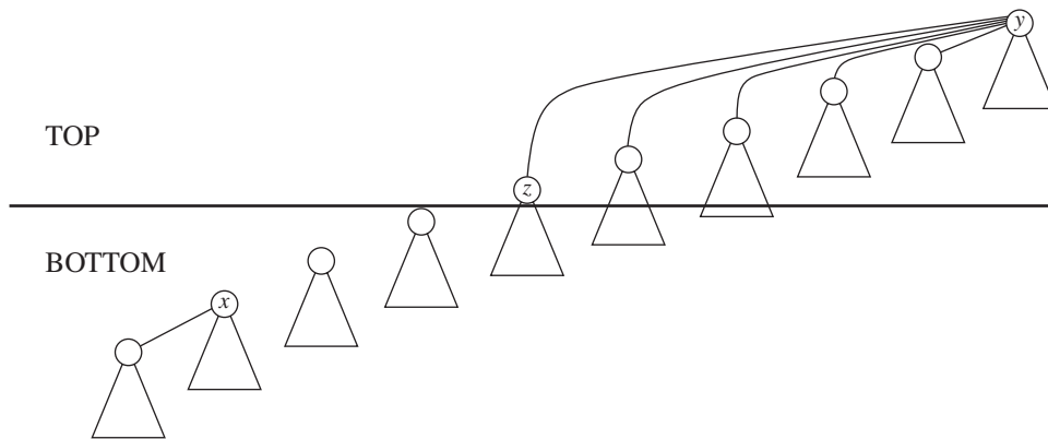
Figure 8.23 Recursive decomposition, case 3: Path compression can be performed on the top nodes, but the bottom nodes must get new parents; the parents cannot be top parents, and they cannot be other bottom nodes
