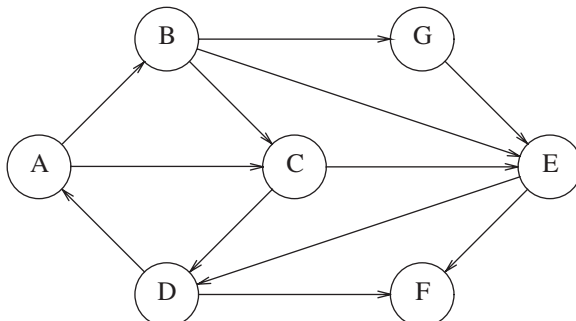
Figure 9.86 Graph used in Exercise 9.26
