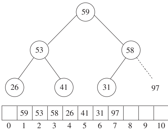
Figure 7.9 Heap after first deleteMax
