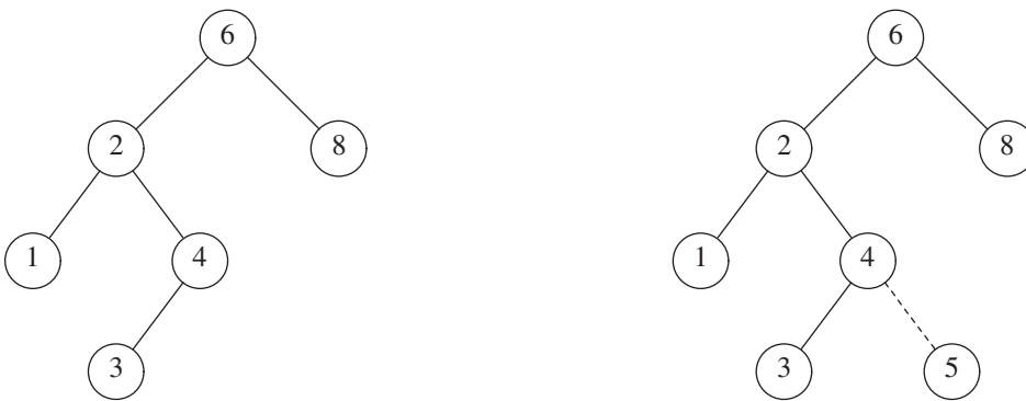
Figure 4.22 Binary search trees before and after inserting 5
