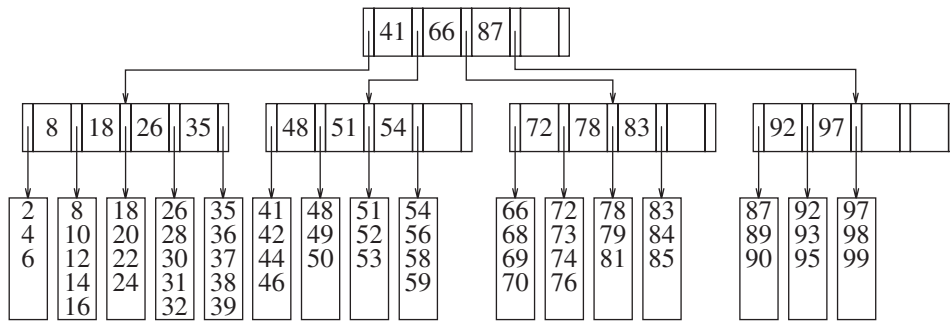
Figure 4.63 B-tree of order 5
