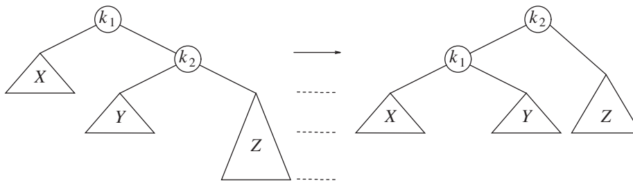
Figure 4.36 Single rotation fixes case 4
