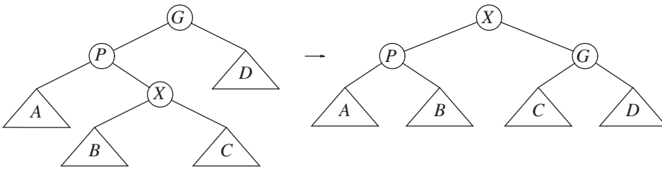
Figure 4.48 Zig-zag
