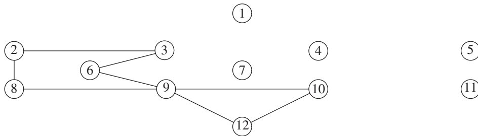
Figure 9.74 Graph after the path 5, 4, 1, 3, 7, 4, 11, 10, 7, 9, 3, 4, 10, 5
