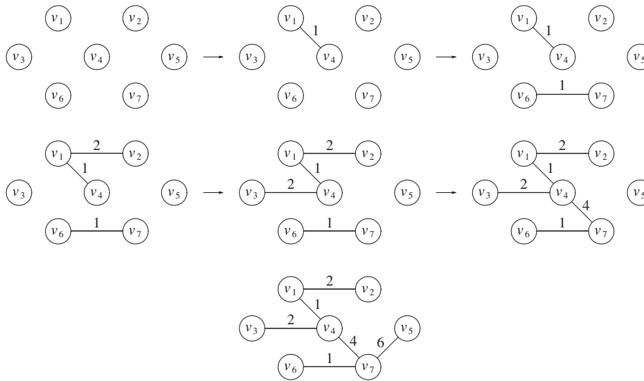
Figure 9.59 Kruskal's algorithm after each stage
