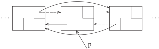
Figure 3.19 Removing node specified by p from a doubly linked list
