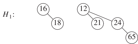
Figure 6.35 Binomial queue H_1 with six elements
