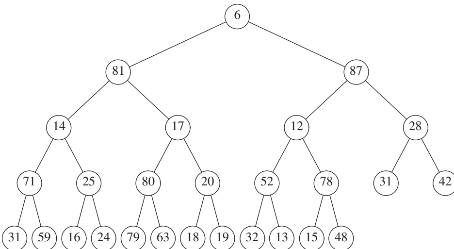
Figure 6.58 Min-max heap
