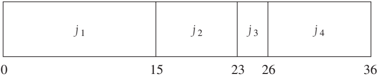
Figure 10.2 Schedule #1
