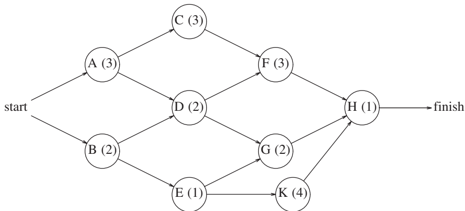
Figure 9.33 Activity-node graph
