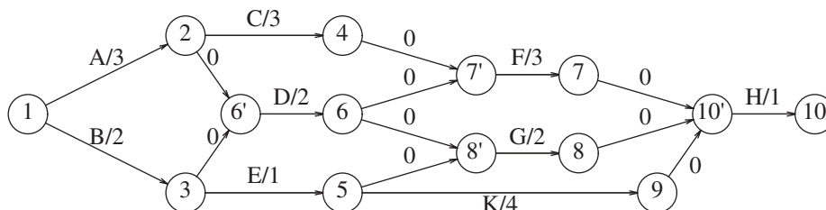
Figure 9.34 Event-node graph
