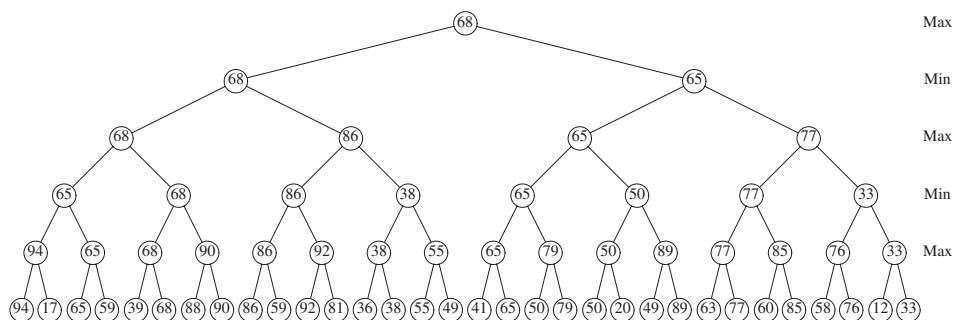
Figure 10.76 Game tree, which can be pruned
