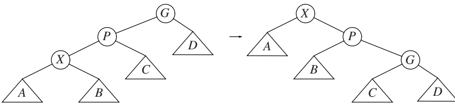
Figure 4.49 Zig-zig
