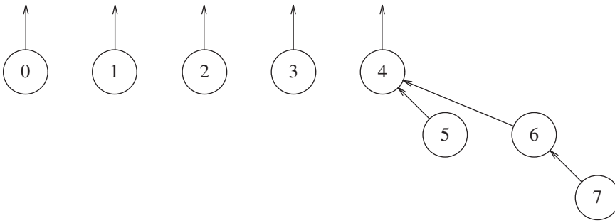
Figure 8.4 After union(4,6)
