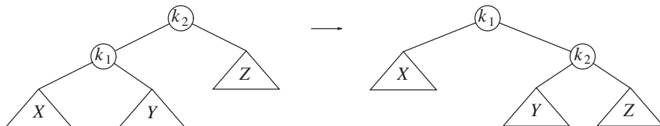
Figure 4.43 Single rotation
