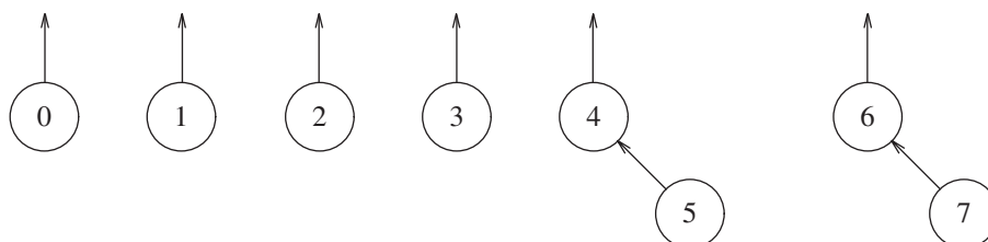
Figure 8.3 After union (6,7)
