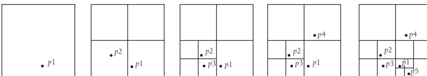
Figure 12.51 The plane partitioned by a quad tree after the insertion of p1 = (53, 14) , p2 = (27, 28) , p3 = (30, 11) , p4 = (67, 51) , p5 = (70, 3)
