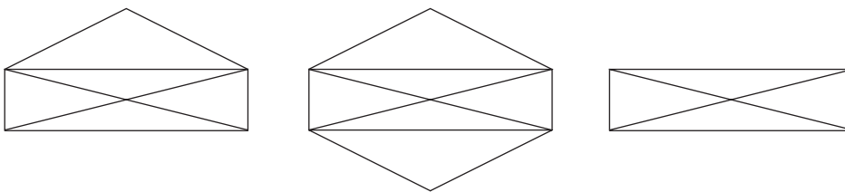
Figure 9.70 Three drawings
