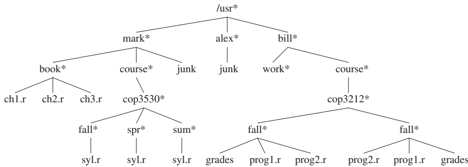
Figure 4.5 UNIX directory
