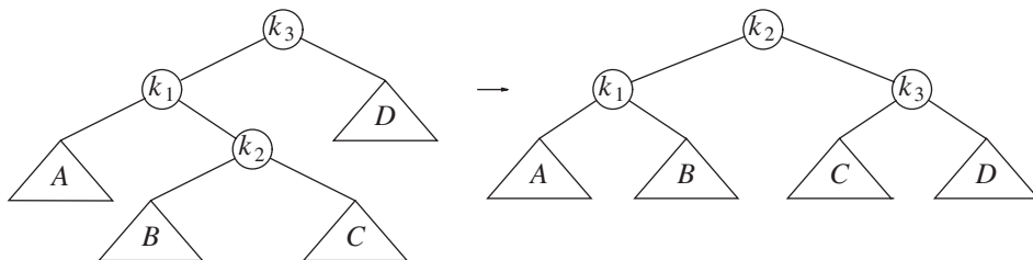
Figure 4.45 Double rotation
