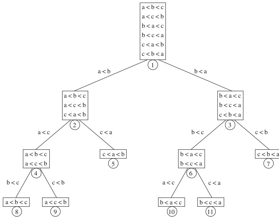
Figure 7.20 A decision tree for three-element sort
