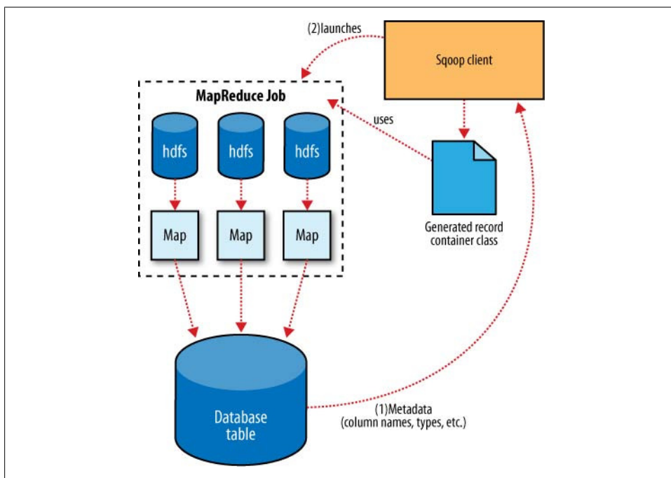
Figure 15-4. Exports are performed in parallel using MapReduce
