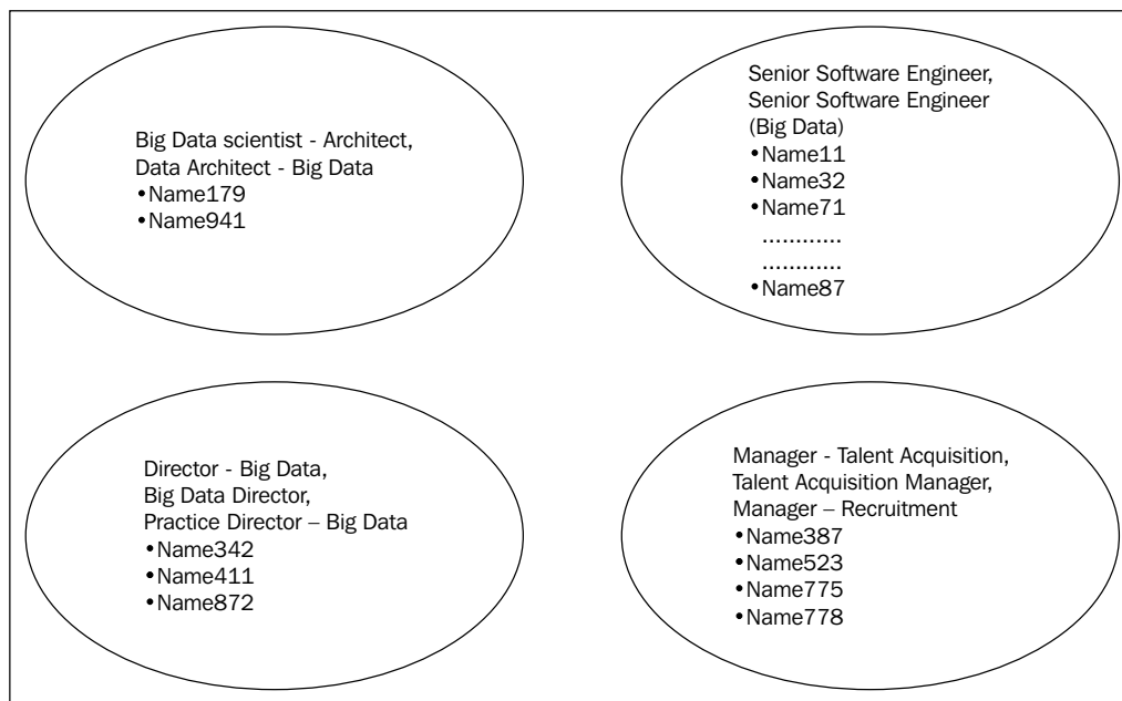
Clustering output
