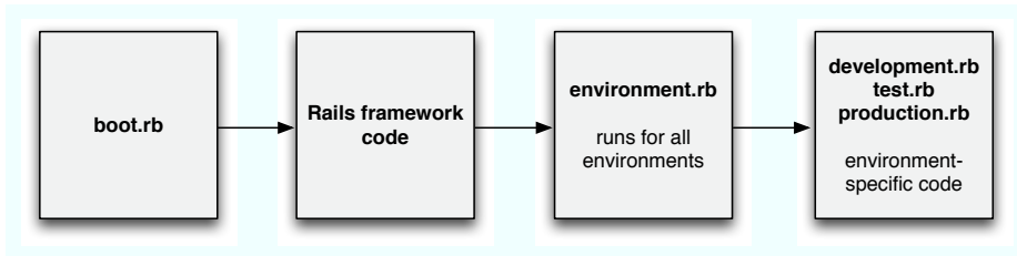
Figure 4.2: The Rails boot/initialization process
