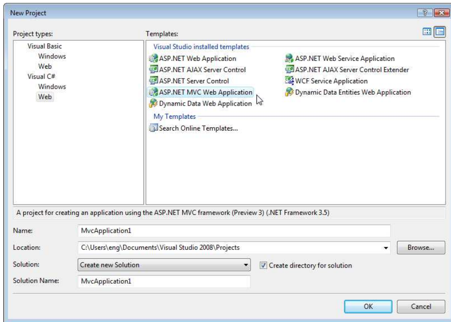
Figure 13.2: Creating a new ASP.NET MVC project
