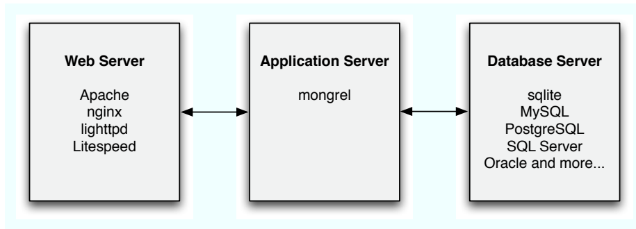
Figure 4.1: The typical Rails stack
