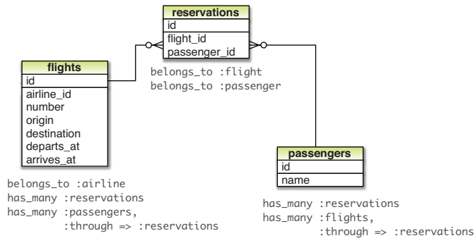
Figure 6.4: Relationship between flights and passengers
