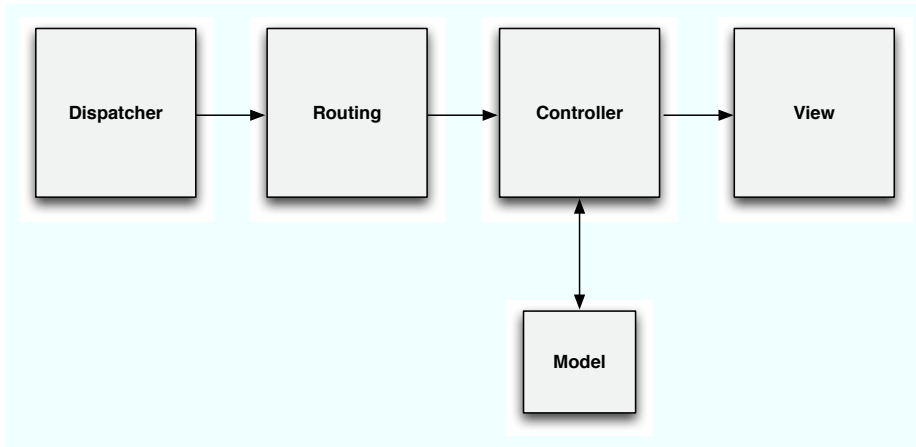
Figure 4.3: The journey of an HTTP request in a Rails app
