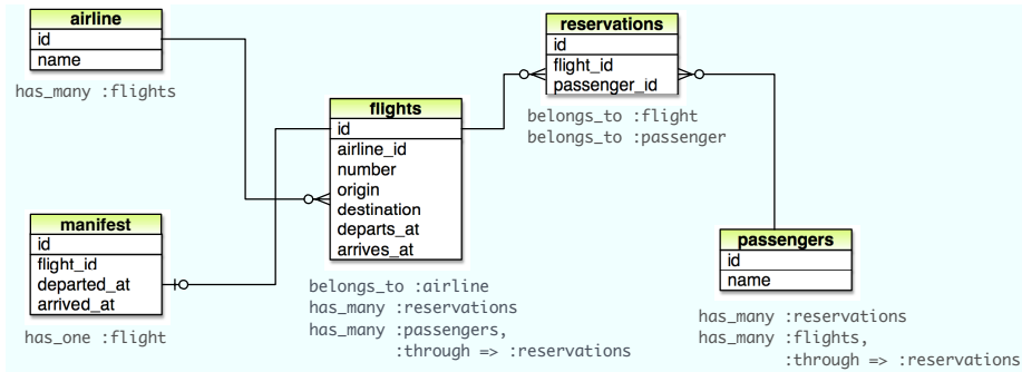
Figure 5.1: Database diagram for flight reservation example
