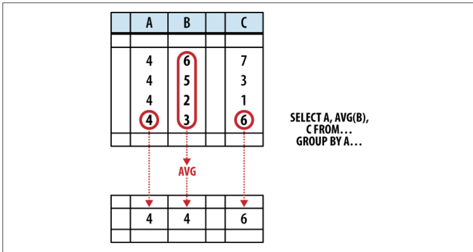
Figure 5-7. The SELECT header will flatten any row groups created by GROUP BY. This figure shows how different columns from one row-group are flattened into an output row. Any value not computed by an aggregate function comes from the last row. Because column A was used as a GROUP BY expression, all the rows are known to have the same value, and it is safe to return. Column B is run through an aggregate function, and is also safe to return. Column C is not safe to return, as the order of the rows within a group is undefined.
